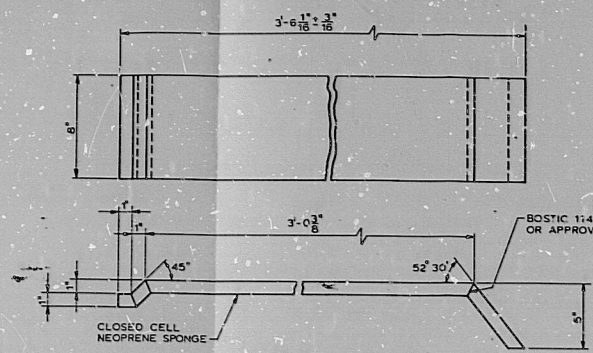
DETAIL 8 RADIAL SPLICE GASKET 4 RECD NOTE 2 SCALE: 3/4\"/>
