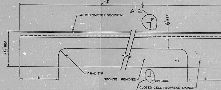
DETAIL 12 SEAL GASKET NOTE 2 MTS SCALE: 3/4\"/>
