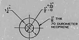
DETAIL 9 WASHER 260 RECD (INCLUDES 100% SPARES) NOTE 2 MTS SCALE: 3/4\"/>
