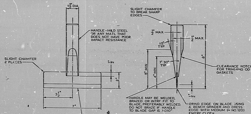
DETAIL 11 GASKET CUTTING TOOL HALF SIZE
