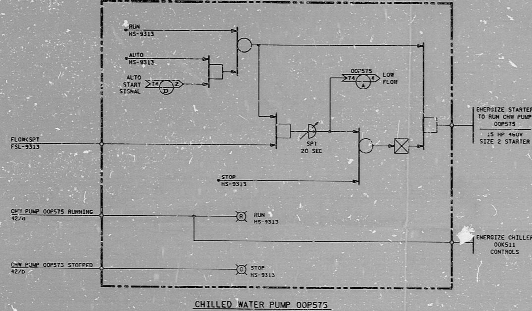
CHILLED WATER PUMP OOP575
