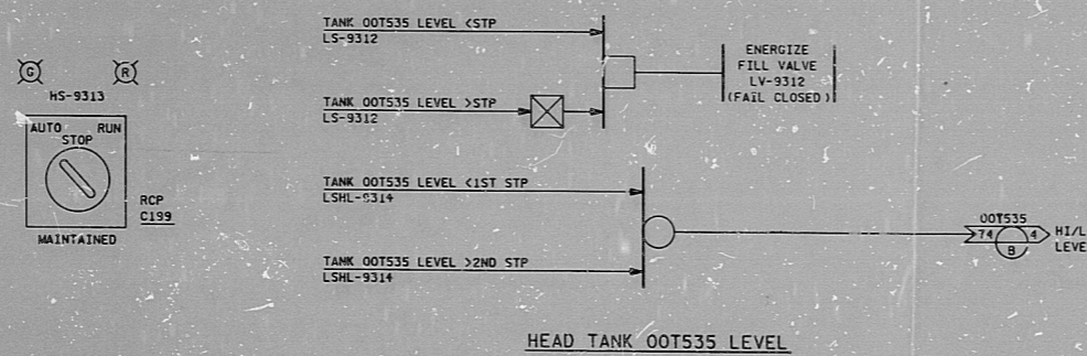
HEAD TANK OOT535 LEVEL
