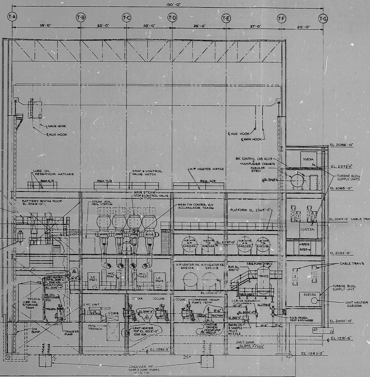
SECTION G LOOKING SOUTH M-06071 (SEE DWG'S M-06060 THRU M-06064)
