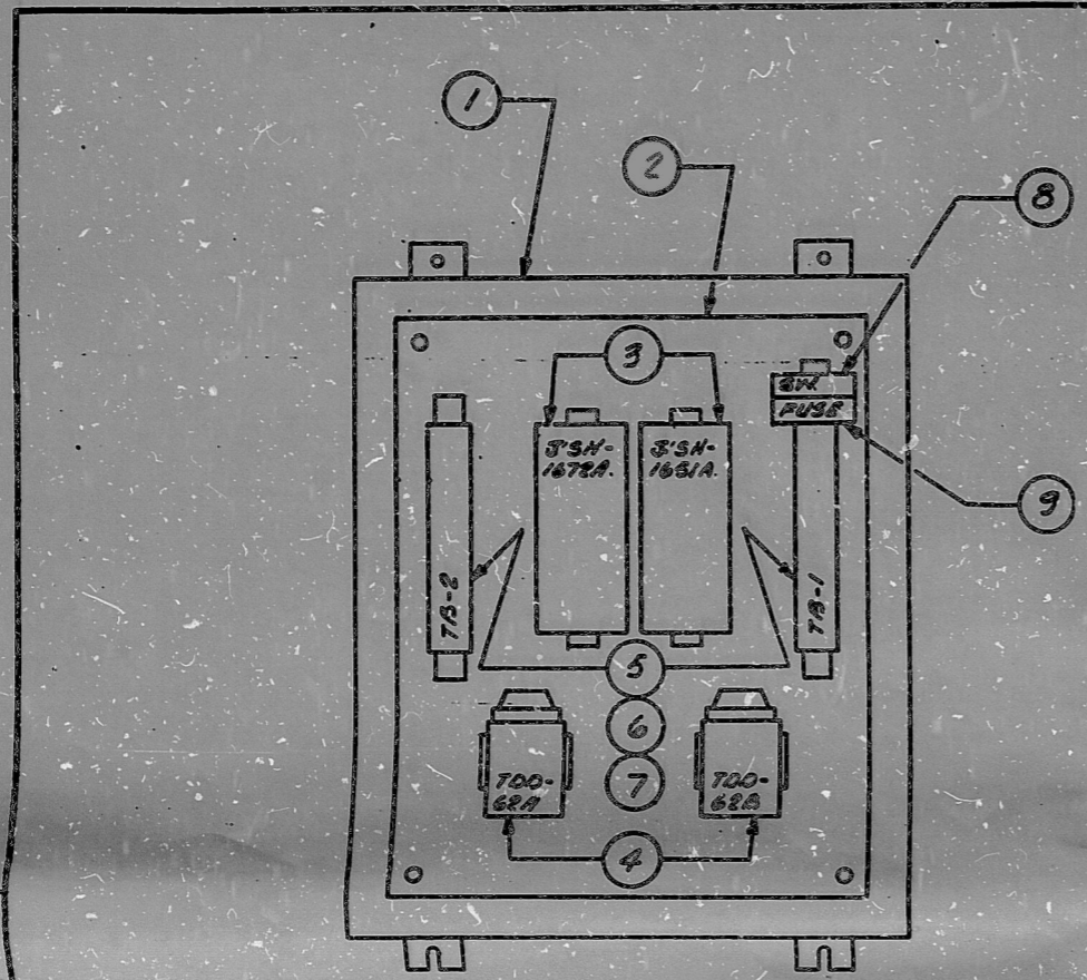
LAYOUT ARRANGEMENT SCALE: 3" = 1'-0"
