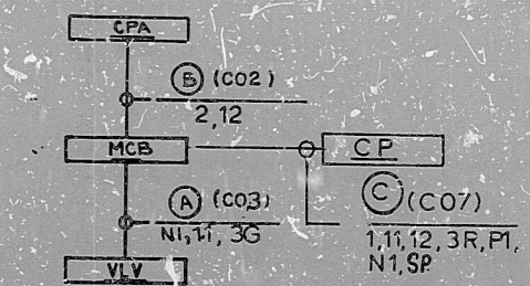
BLOCK DIAGRAM SCHEME NO. SEE TABLE
