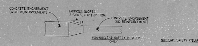
DETAIL "C" (SEE NOTE "22" ON DWG. D-216-001) NO SCALE
