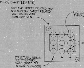
DETAIL "H" (SEE NOTE "14" ON DWG. D-216-001) NO SCALE
