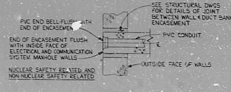
DETAIL "B" (SEE NOTE "5" ON DWG. D-216-001) NO SCALE
