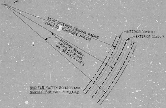
DETAIL "E" (SEE NOTE "7" ON DWG. D-216-001) NO SCALE
