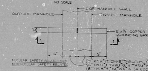
DETAIL "G" (SEE NOTE "24" ON DWG. D-216-001) NO SCALE
