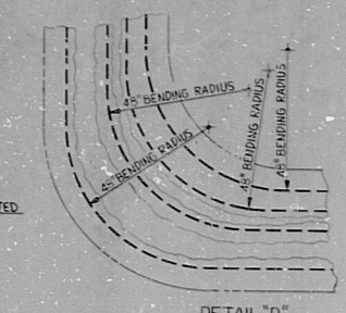
DETAIL "D" (SEE NOTE "2" ON DWG. D-216-001) NO SCALE
