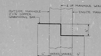
SECTION 1-1 (SEE NOTE "24" ON DWG. D-216-001) NO SCALE
