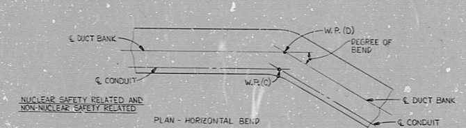
DETAIL "K" (SEE NOTE "16" ON DWG. D-216-001) NO SCALE
