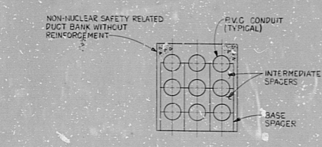
DETAIL "J" (SEE NOTE "14" ON DWG. D-216-001) NO SCALE
