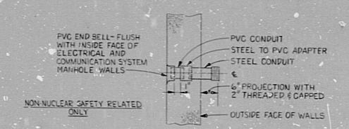
DETAIL "F" (SEE NOTE "18" ON DWG. D-216-001) NO SCALE
