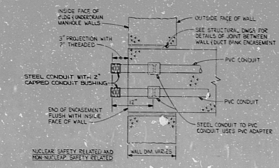
DETAIL "A" (SEE NOTE "15" ON DWG. D-216-001) NO SCALE
