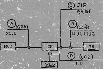
BLOCK DIAGRAM SCHEME NO. -SEE TABLE
