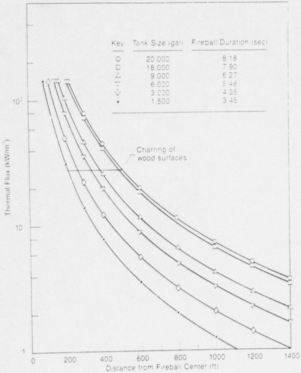
FIGURE 11. THERMAL FLUX VS. DISTANCE FROM FIREBALL CENTER FOR LIQUID HYDROGEN STORAGE SYSTEM
