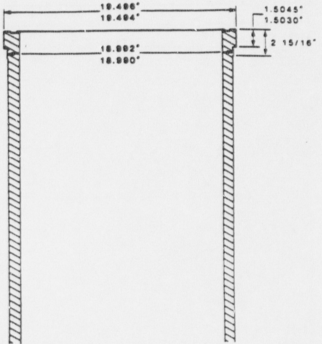
Cylinder liner.
