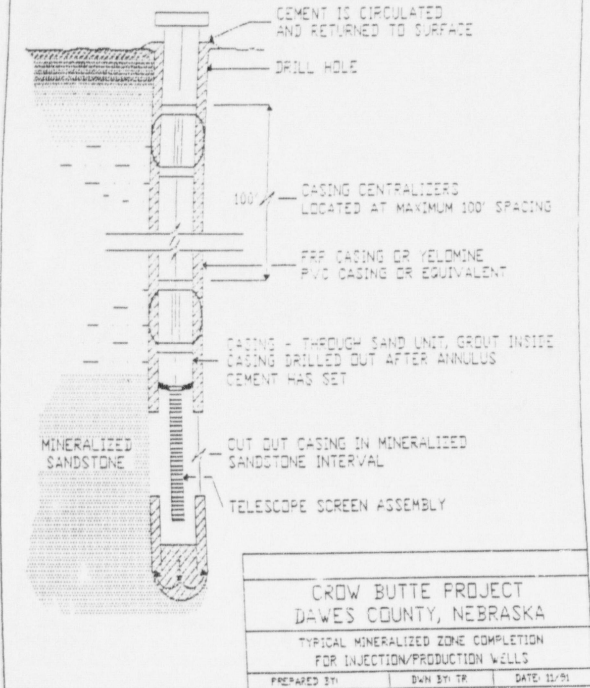
Figure 3-5. Well completion method three at the Crow Butte Uranium Project (from CBR, 1995)
