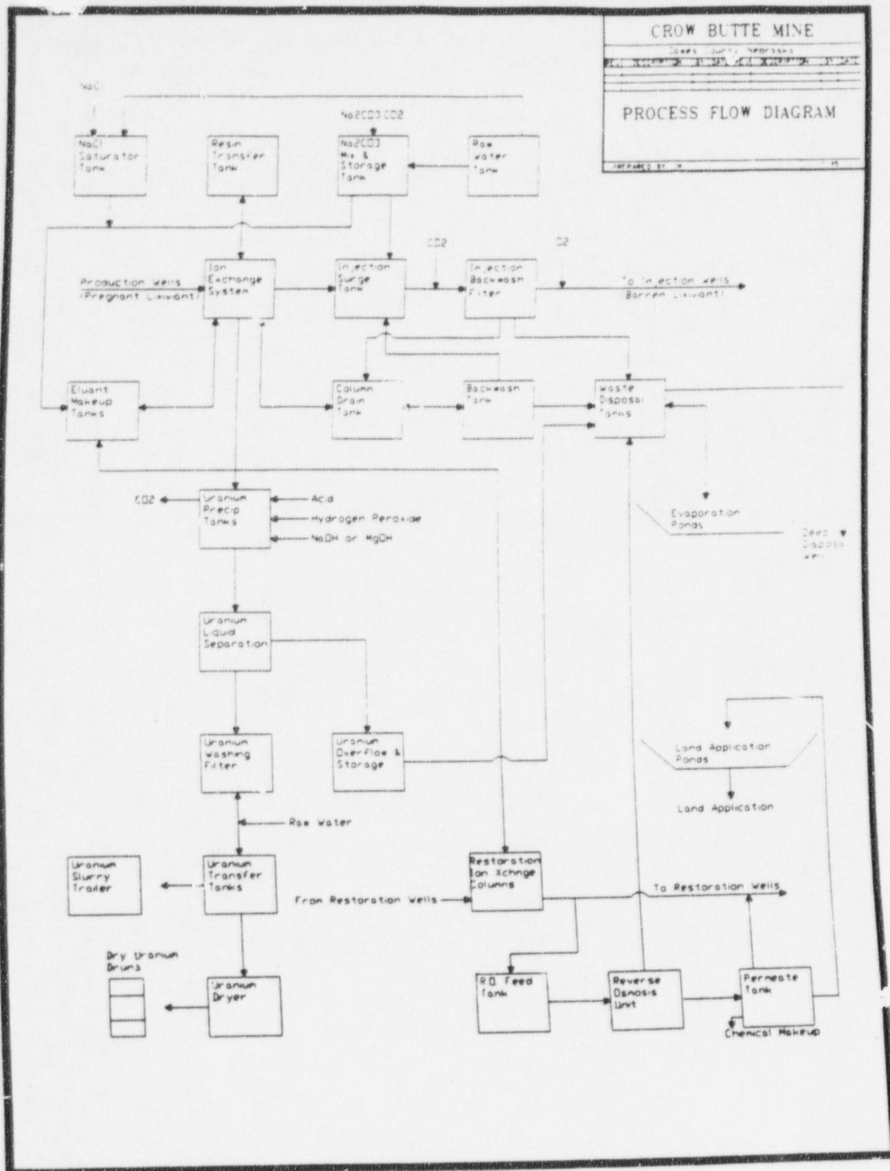
Figure 3-6. Flow sheet of the uranium recovery process at the Crow Butte Uranium Project (from CBR, 1995)
