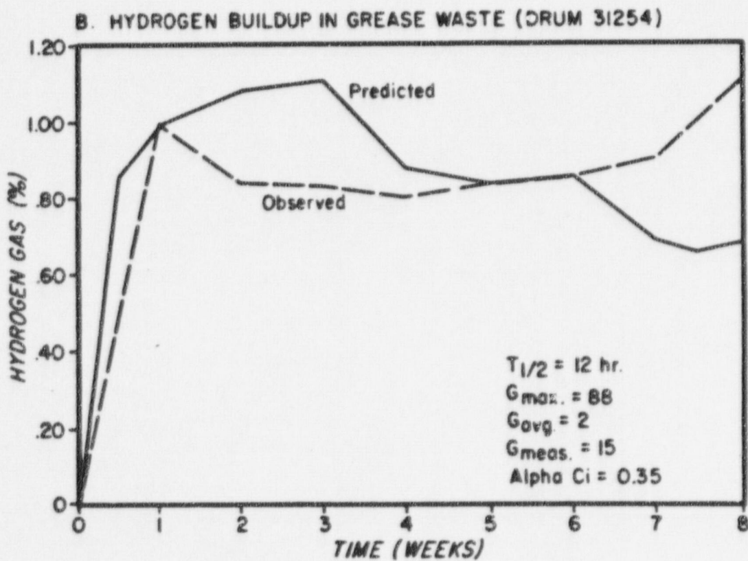
Figure 13. Hydrogen buildup in vented drums.
