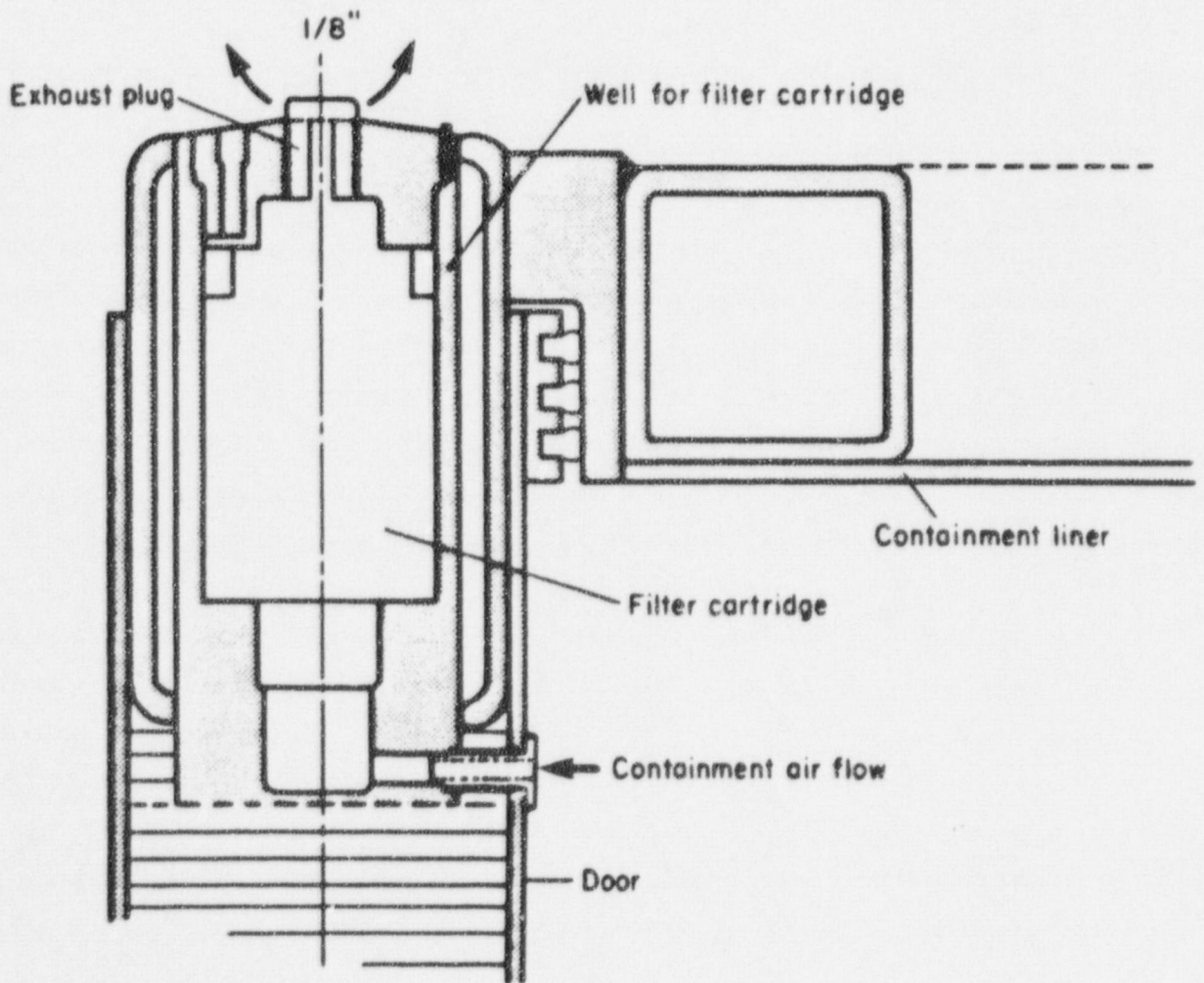
Figure 10. Filter vent concepts.
