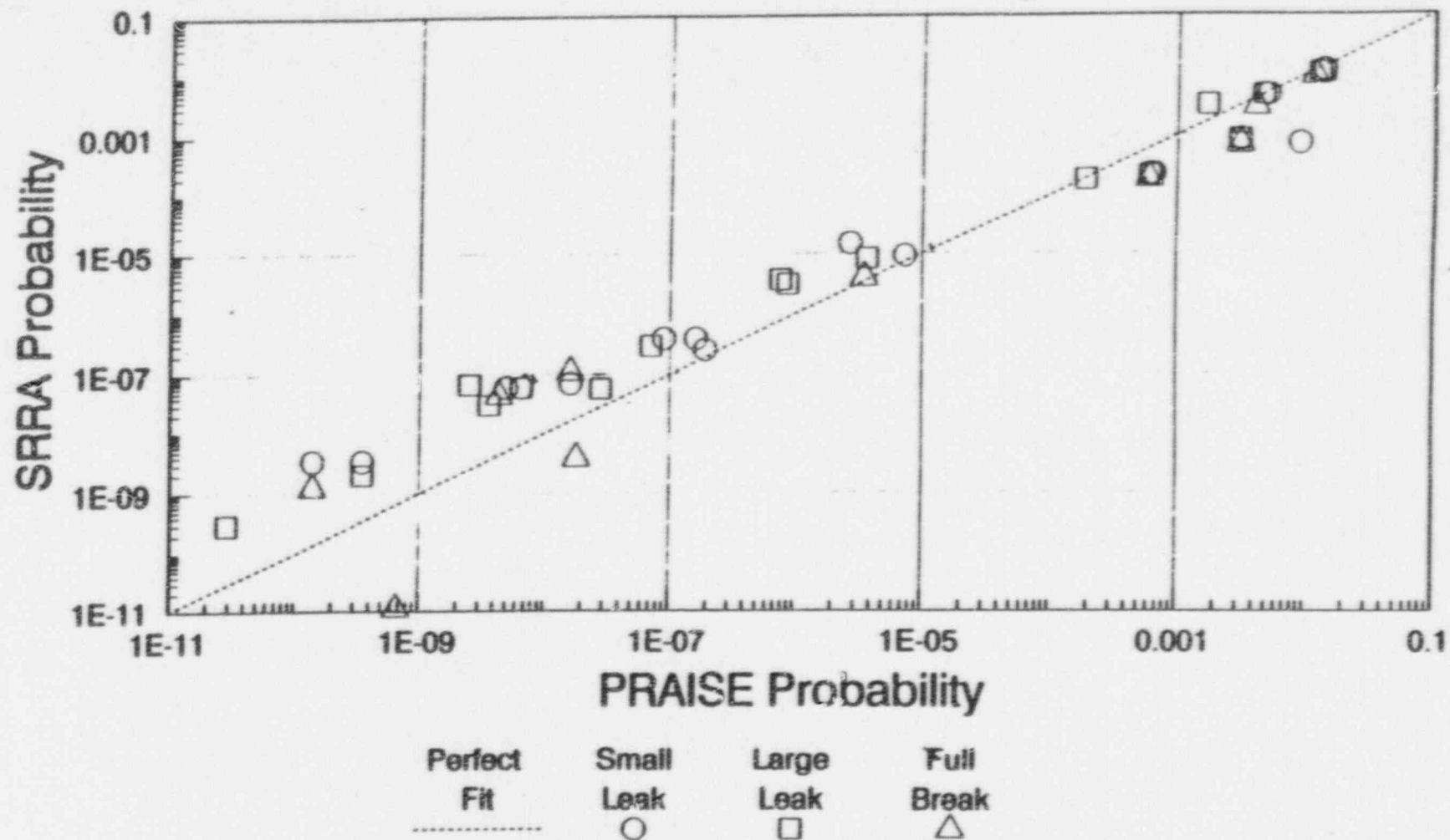
Figure 3-5 Comparison of Calculated Piping Probabilities
