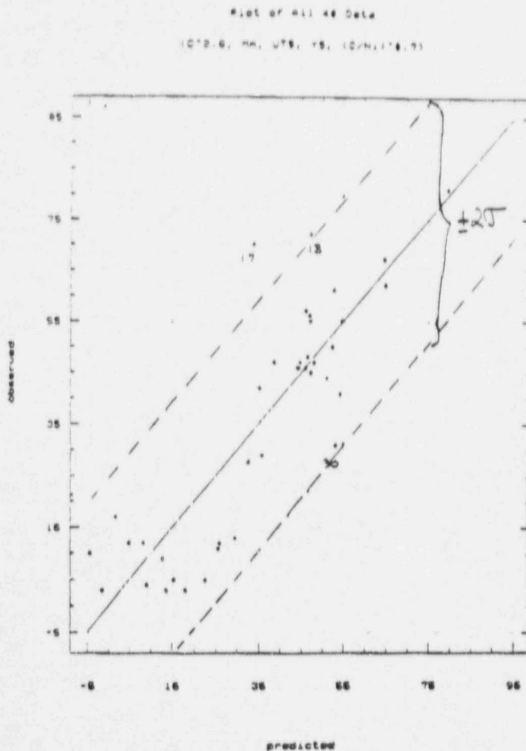
Figure 3-4 Curve Fit of Alloy 600 Grain Boundary Carbide Coverage Results [7]
