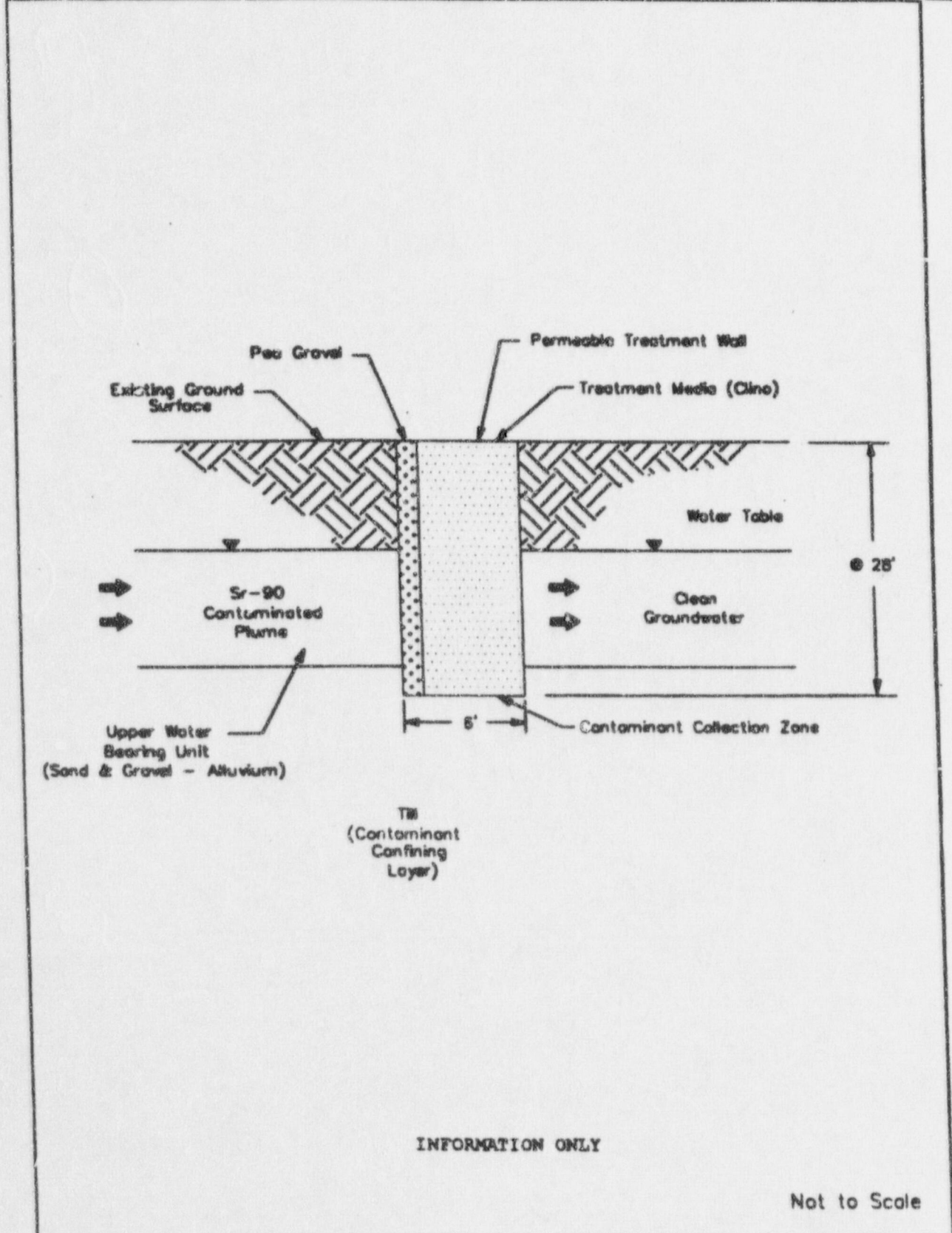
Figure 1 Process Flow Diagram - Permeable Treatment Wall
