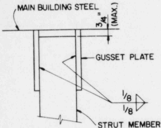
AS-DESIGNED :
