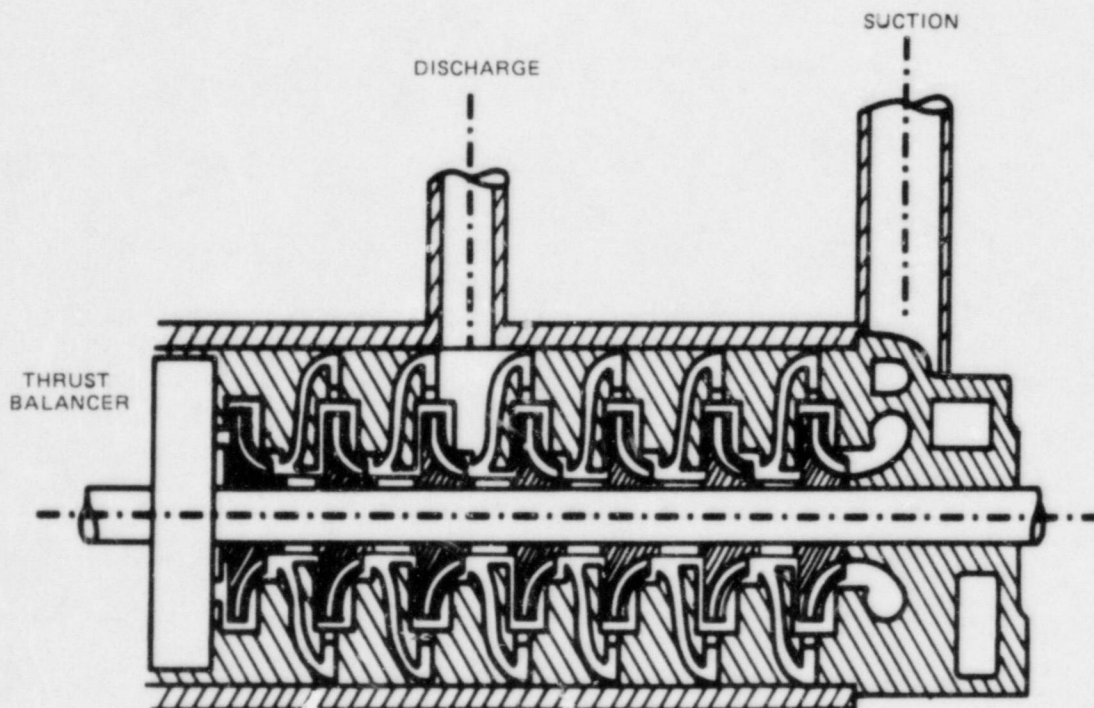
Fig. 3. Single-suction, in-line-impellers AUXFP.
