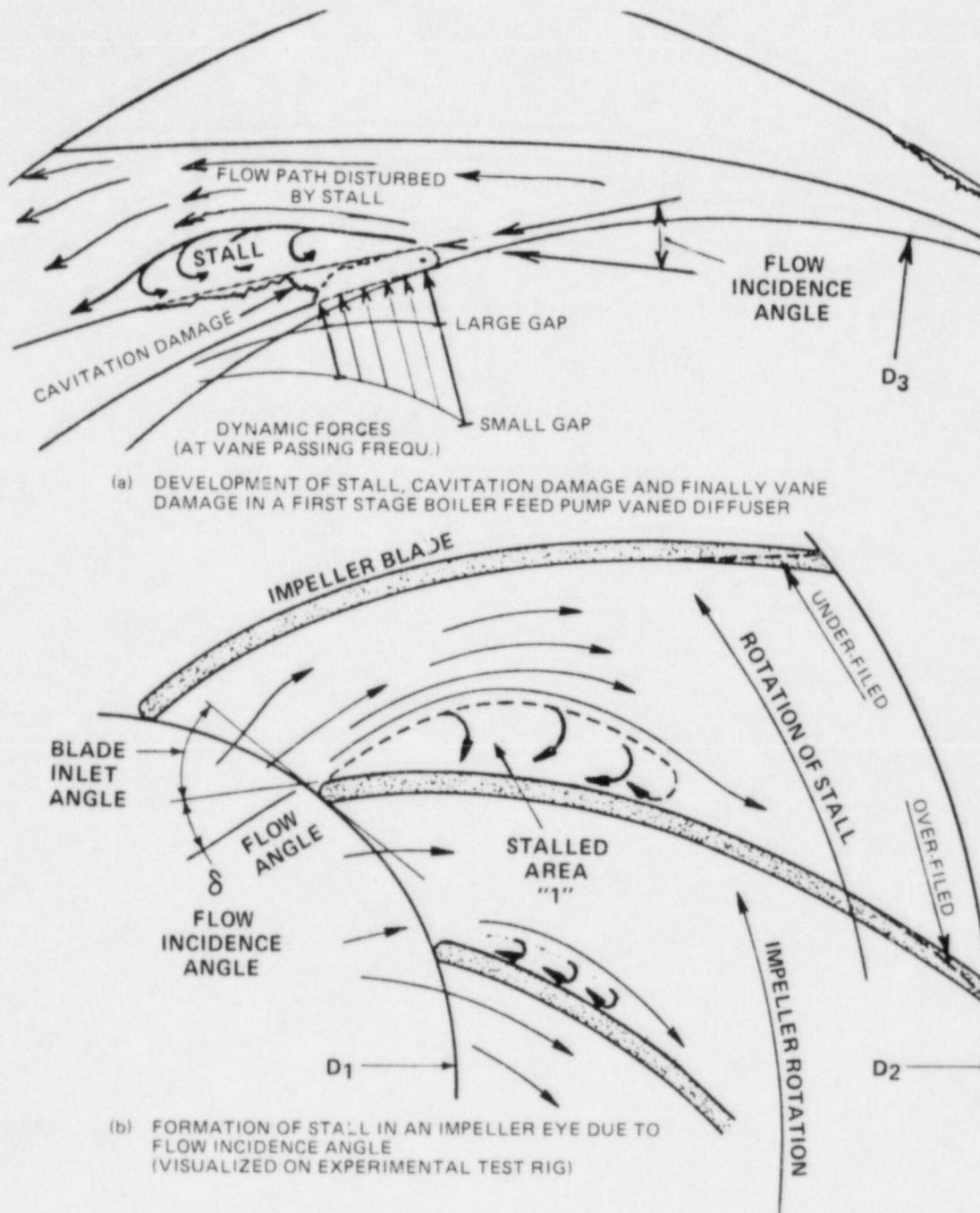
Fig. D.2. Formation of stall (a) in diffuser and (b) in eye of impeller. Source: E. Makay and O. Szamody, Recommended Design Guidelines for Feedwater Pumps in Large Power Generating Units , EPRI CS-1512, Electric Power Research Institute, September 1980.
