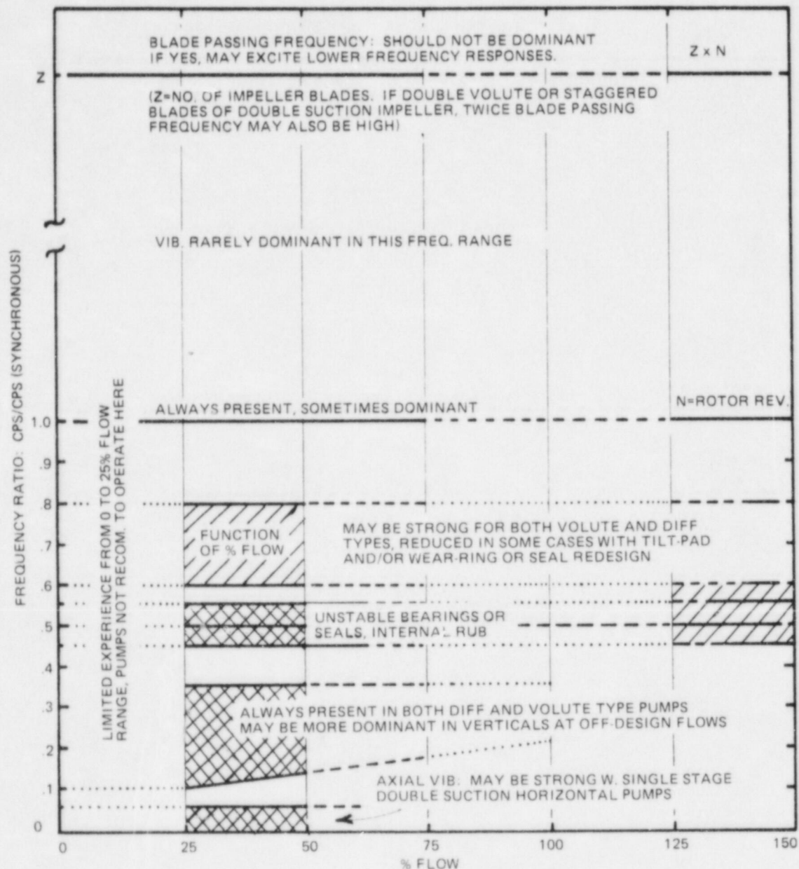
Fig. D.6. Frequencies of hydraulically induced dynamic forces acting on the rotor of a centrifugal pump. Source: E. Makay and O. Szamody, Survey of Feed Pump Outages , EPRI FP-754, Electric Power Research Institute, April 1978.
