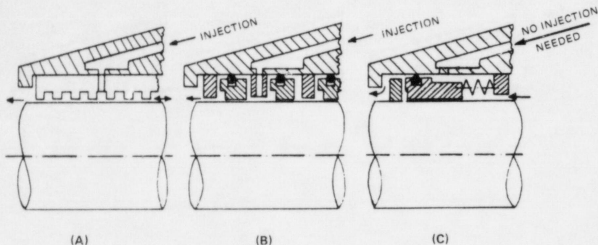
Fig. D.11. Shaft seal types used in boiler feed, nuclear feed, and feedwater booster pumps. (a) Labyrinth, (b) floating ring seals with single injection, and (c) mechanical seal. Source: E. Makay and O. Szamody, Survey of Feed Pump Outages , EPRI FP-754, Electric Power Research Institute, April 1978.
