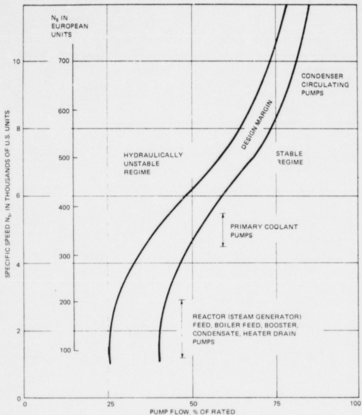
Fig. D.1. Anticipated useful operating ranges for pumps used in large nuclear and fossil power generating units. (Inner line of design margin area is preferred; if hydraulic instability occurs at higher flows various pump and system problems can be expected.) Source: E. Makay and O. Szamody, Survey of Feed Pump Outages , EPRI FP-754, Electric Power Research Institute, April 1978.
