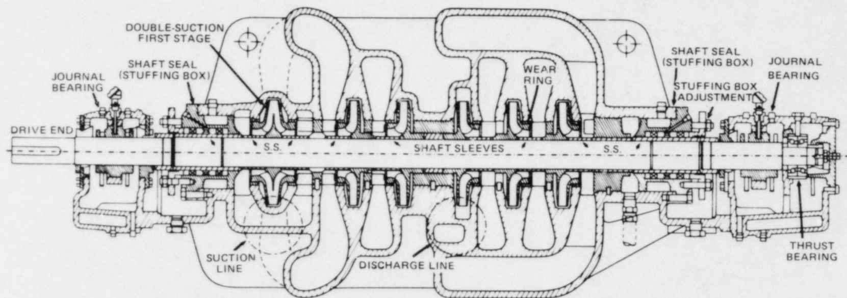
Fig. 1. Double-suction, opposed-impellers AUXFP.
