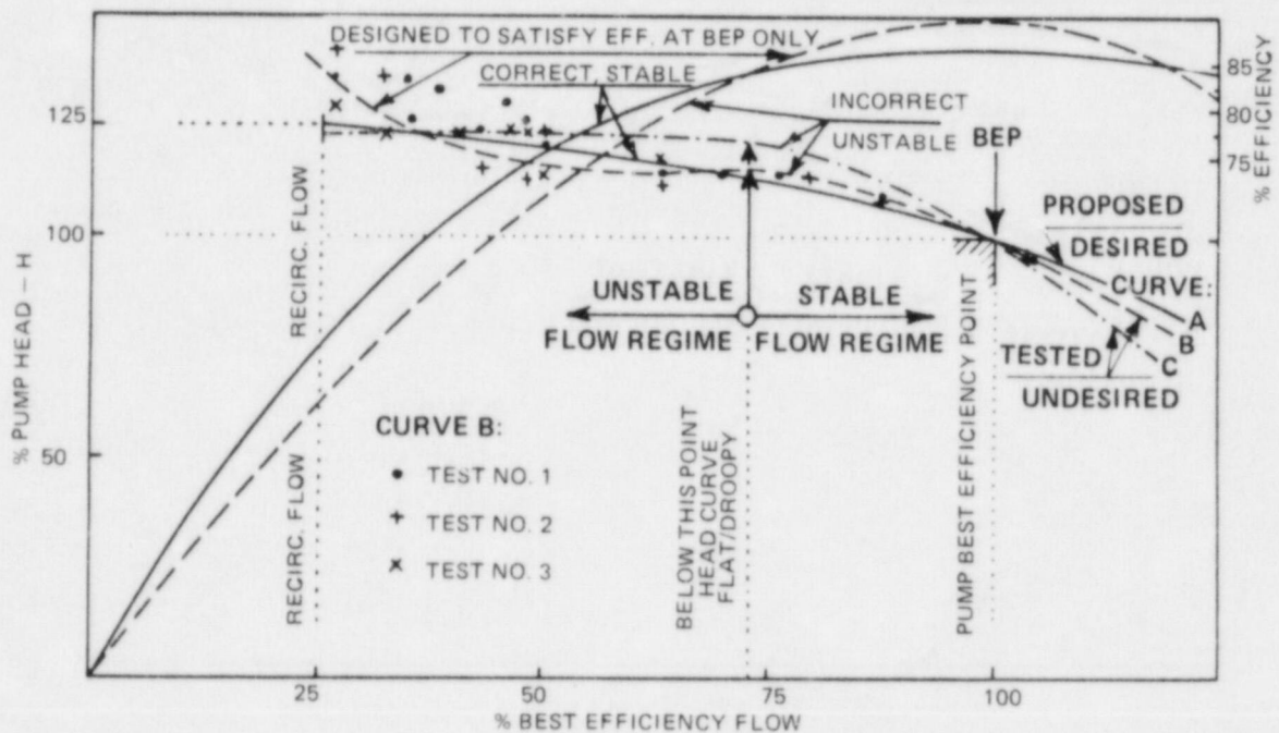
Fig. D.4. Head-capacity characteristics of multistage boiler feed pumps. Curve "A" is correct and desired for stable system operation. Curve "B" represents hydraulically unstable impeller-diffuser design. Parallel- as well as single-pump operation is difficult in the unstable flow regime. Curve "C" shows design with flat head curve at part load resulting in control system malfunctioning. Single-pump operation is possible in unstable regime. Designs "B" and "C" are not acceptable for utility applications. Source: E. Makay and O. Szamody, Survey of Feed Pump Outages, EPRI FP-754, Electric Power Research Institute, April 1978.
