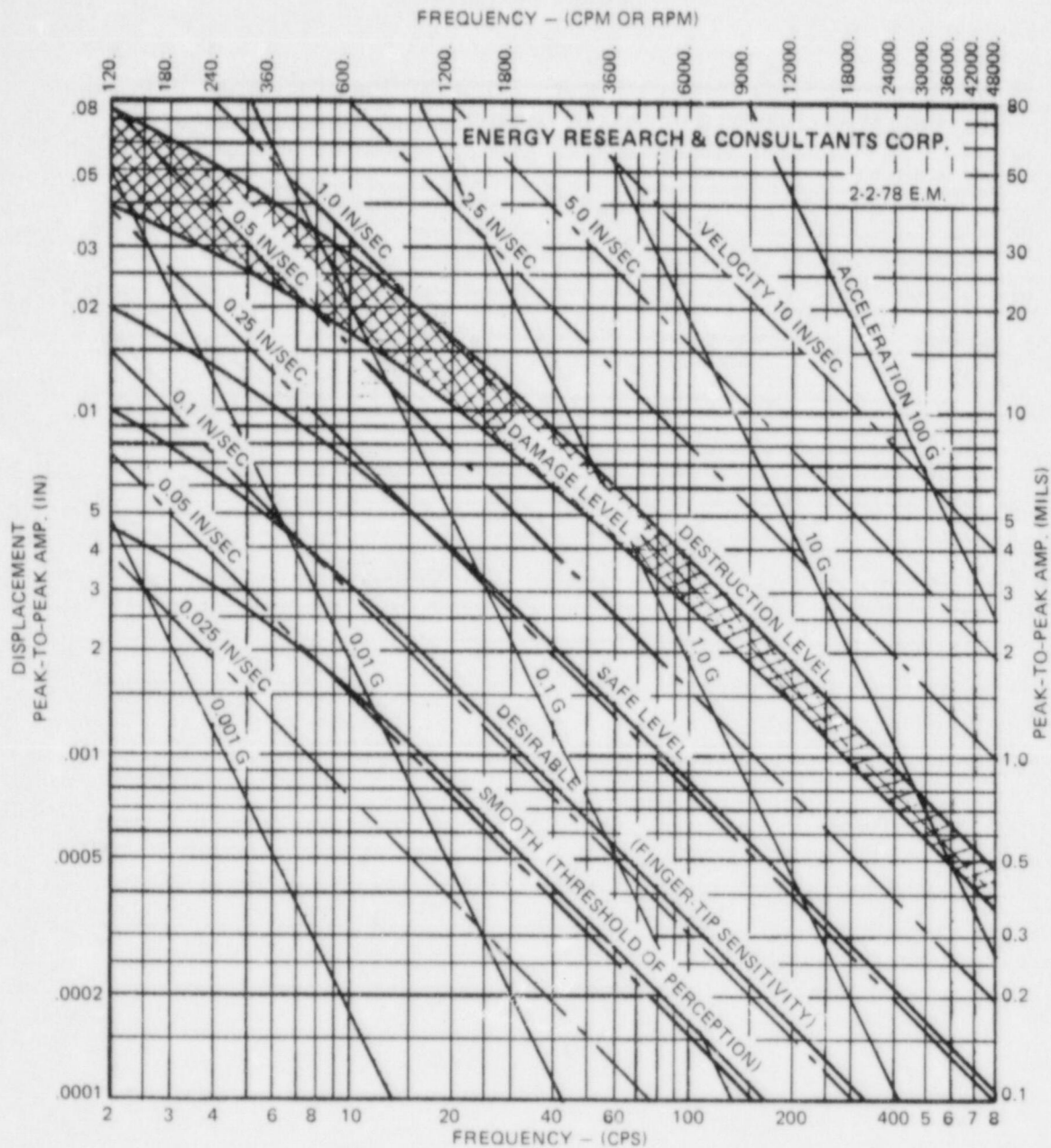
Fig. D.8. Allowable rotor vibration levels measured relative to bearing cap. (Values shown are filtered readings at that particular RPM or frequency; experimental standards). Source: E. Makay and O. Szamody, Survey of Feed Pump Outages , EPRI FP-754, Electric Power Research Institute, April 1978.
