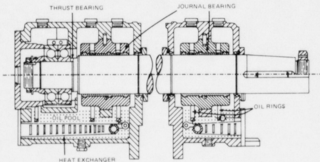
Fig. D.12. Typical AUXFP bearing system.
