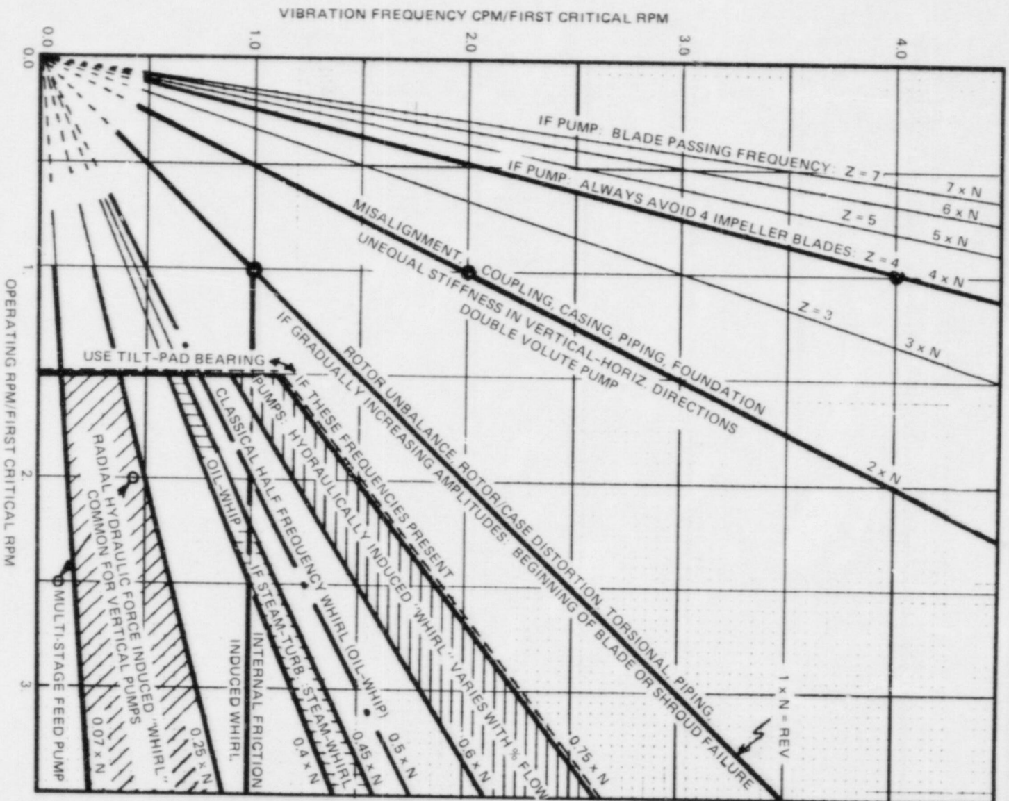
Fig. D.7. Vibration frequency vs speed. Causes and cures of common vibration problems of centrifugal pumps, steam and gas turbines, fans and blowers, compressors, and other centrifugal equipment. Source: E. Makay and O. Szamody, Survey of Feed Pump Outages , EPRI FP-754, Electric Power Research Institute, April 1978.
