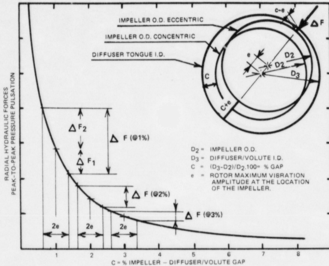
Fig. D.5. Influence of pump impeller to diffuser/volute radial gap on pressure pulsation at blade-passing frequency and rotor deflection caused radial forces. Source: R. Makay and U. Szamody, Survey of Feed Pump Outages , EPRI FP-754, Electric Power Research Institute, April 1978.
