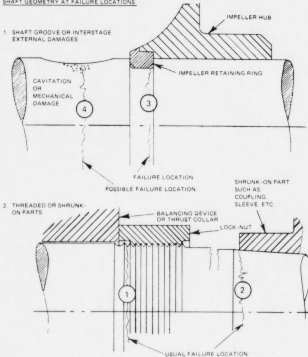
Fig. D.13. Typical multistage centrifugal pump shaft failure locations. The four most frequent locations are shown in order of failure frequency. Source: E. Makay and O. Szamody, Recommended Design Guidelines for Feedwater Pumps in Large Power Generating Units , EPRI CS-1512, Electric Power Research Institute, September 1980.
