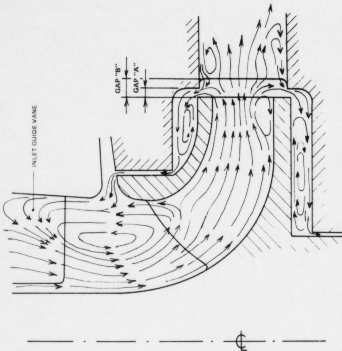
Fig. D.3. Secondary flow pattern in and around pump impeller stage at off-design flow operation. Source: E. Makay and O. Szamody, Survey of Feed Pump Outages , EPRI FP-754, Electric Power Research Institute, April 1978.
