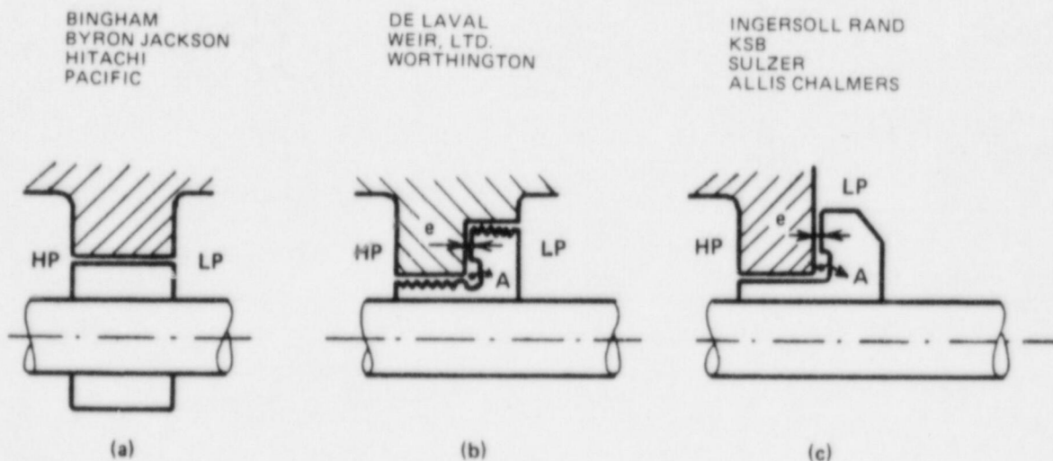
Fig. D.9. Customary axial balancing devices for high-pressure multistage boiler feed pumps. (a) Balance drum (b) and (c) balance disk. Source: E. Makay and O. Szamody, Survey of Feed Pump Outages , EPRI FP-754, Electric Power Research Institute, April 1978.
