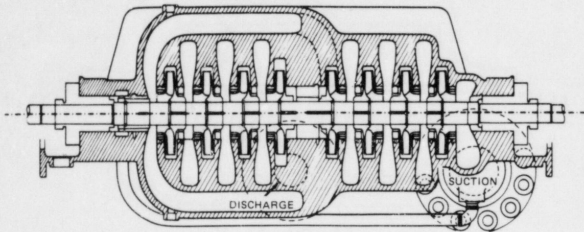
Fig. 2. Single-suction, opposed-impellers AUXFP.
