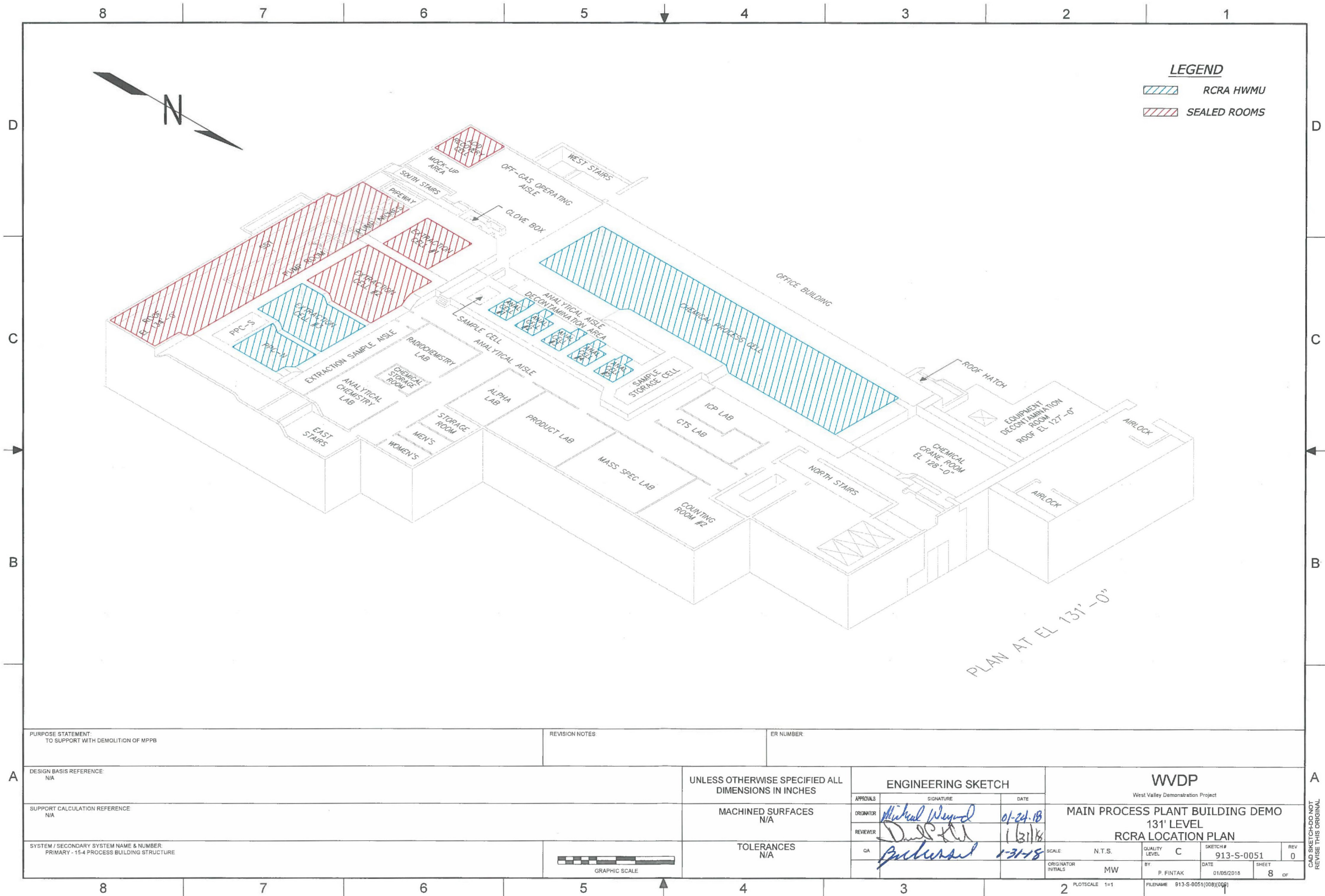
Attachment A (continued) Main Plant Process Building Breakdown By Level
