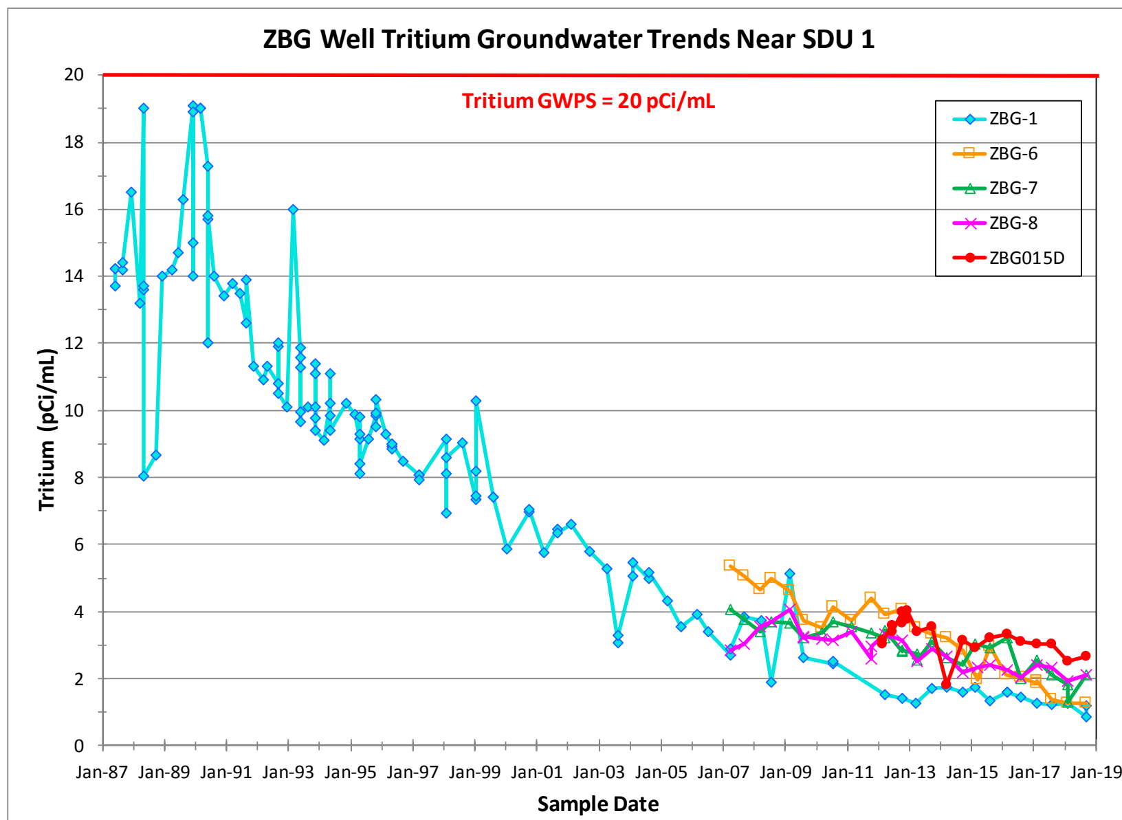
Figure 11. ZBG Well Tritium Groundwater Trends
