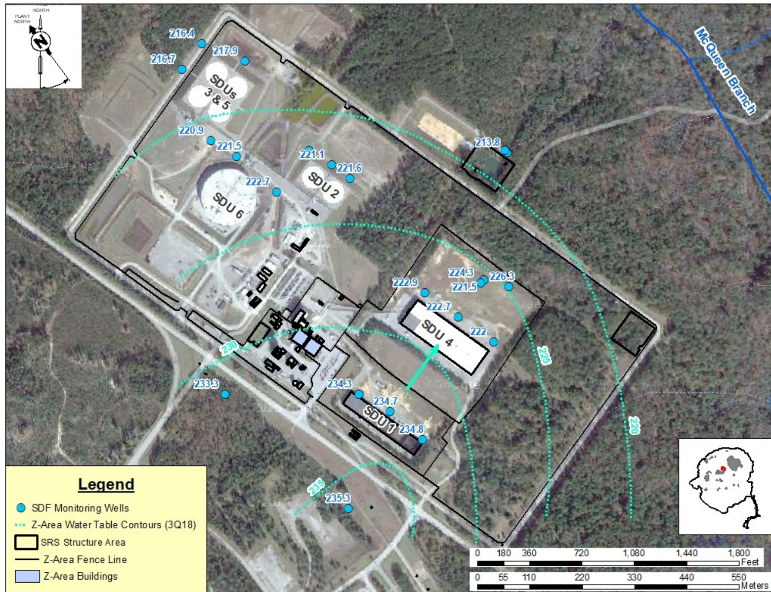
Figure 4. 3Q18 Water Table Elevations (ft-msl)
