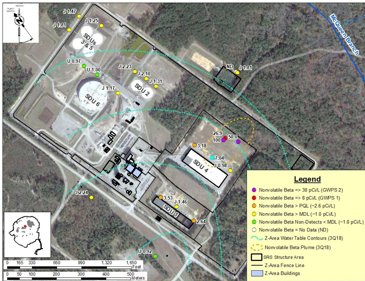
Figure 8. Approximate Nonvolatile Beta Groundwater Plume (3Q18)
