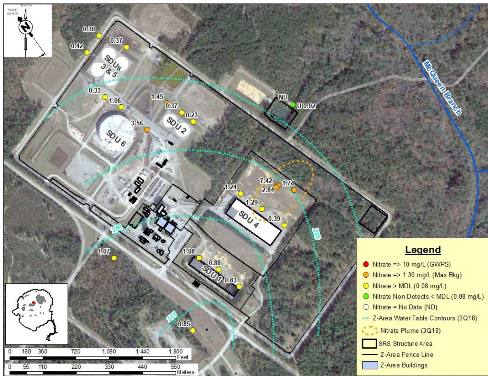
Figure 10. Approximate Nitrate Groundwater Plume (3Q18)
