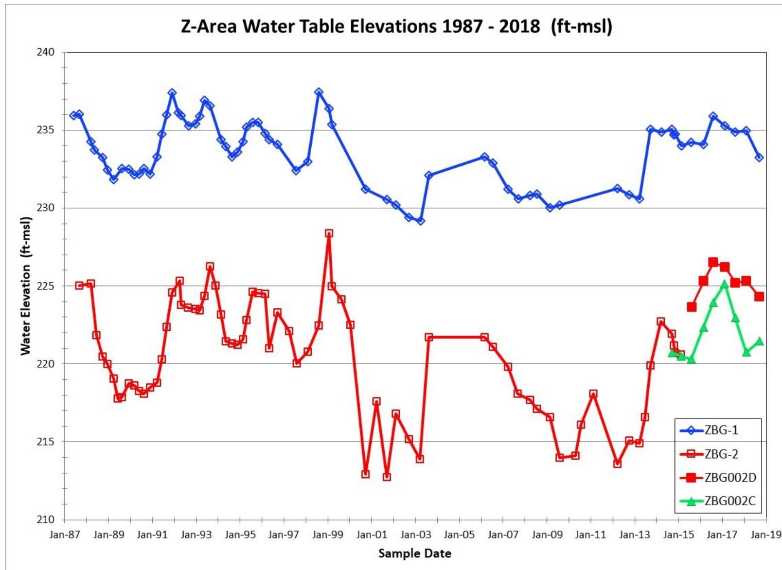
Figure 5. Z-Area Water Table Elevations (ft-msl)
