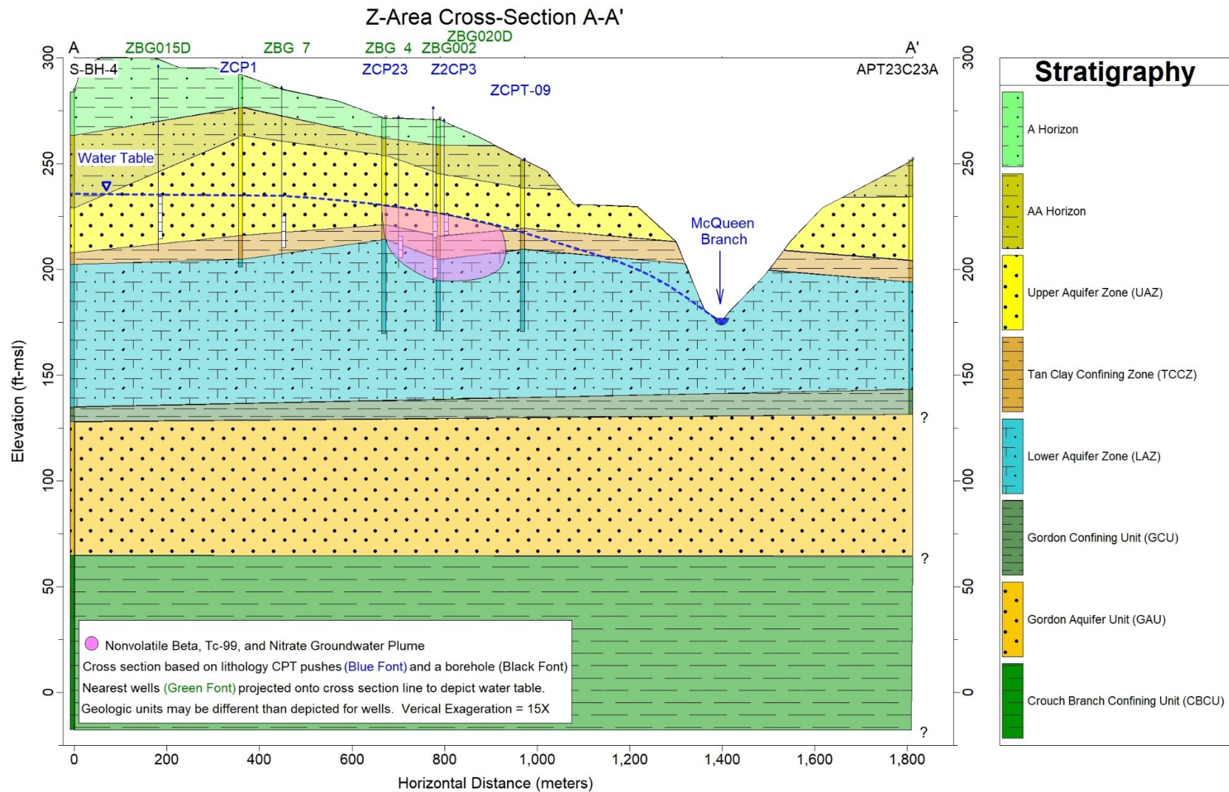
Figure 6. Z-Area Cross Section with 3Q18 Water Table
