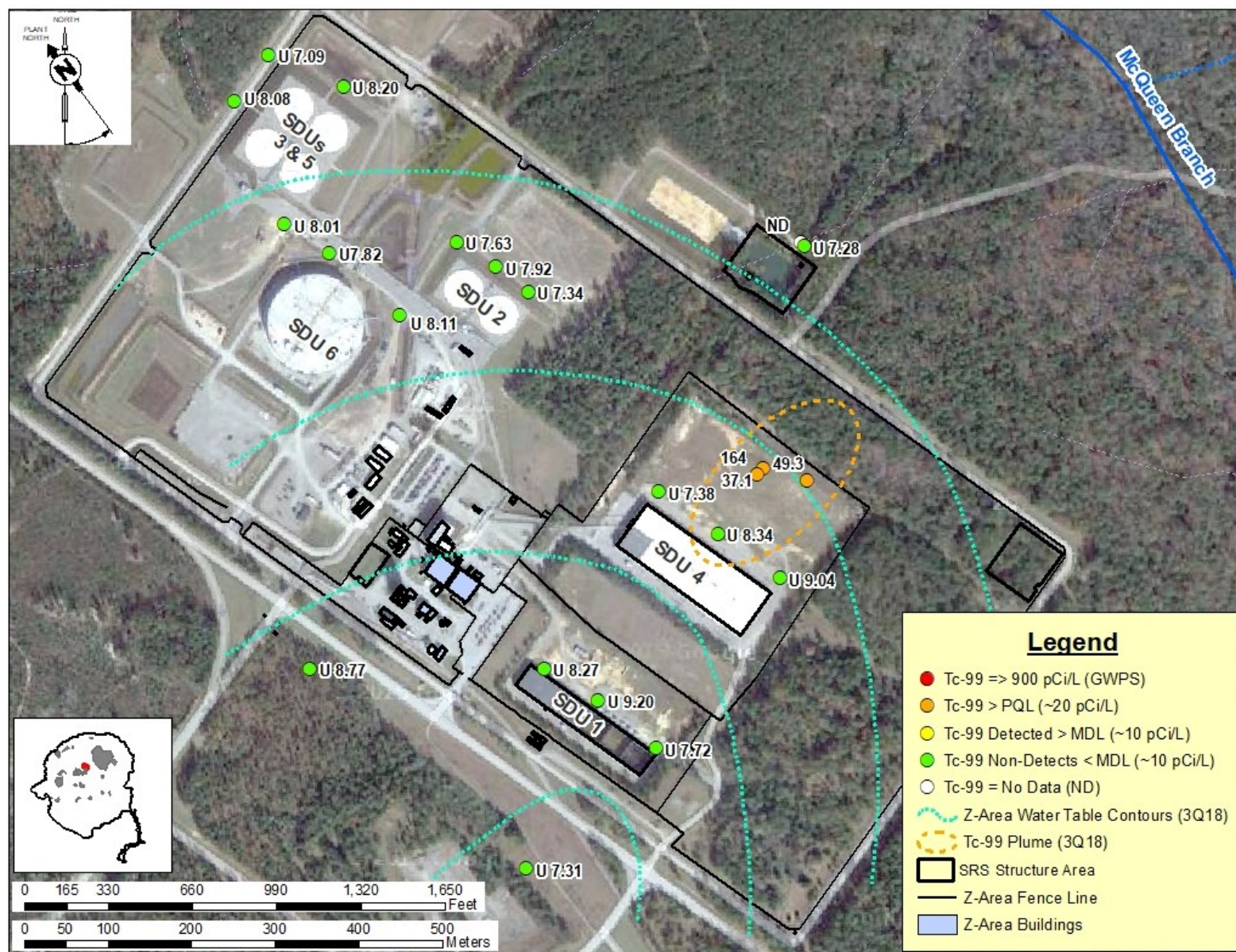
Figure 9. Approximate Tc-99 Groundwater Plume (3Q18)
