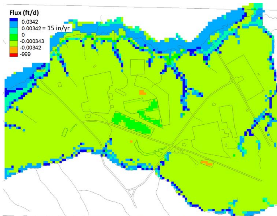
Figure 7-36. Simulated surface flux for the PEST.51 / GSA2016.LW case (ft/d).
