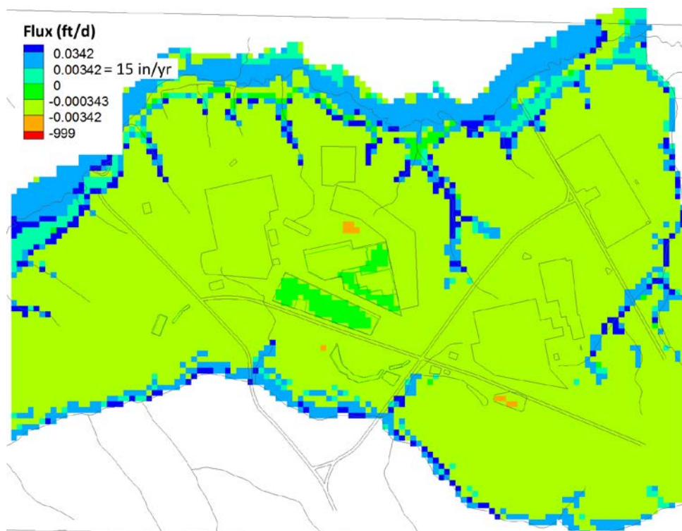
Figure 7-35. Simulated surface flux for the PEST.47 / GSA2016.LU case (ft/d).
