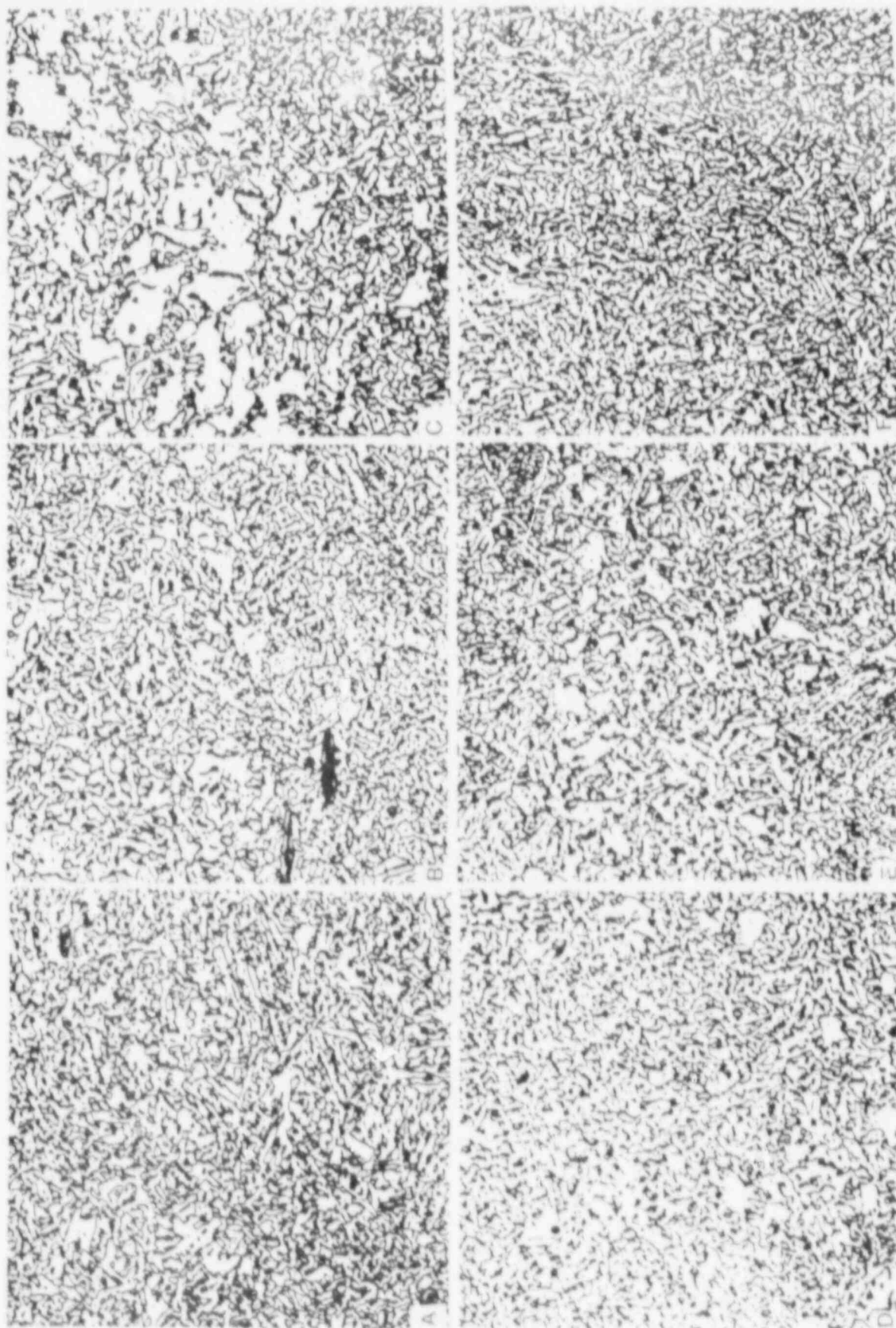
Fig. 6 Microstructures of Base Metal CEB-1 through its thickness: A. I.D. Surface B. 1/8T Location C. 1/2T Location D. 3/4T Location E. 7/8T Location F. O.D. Surface
