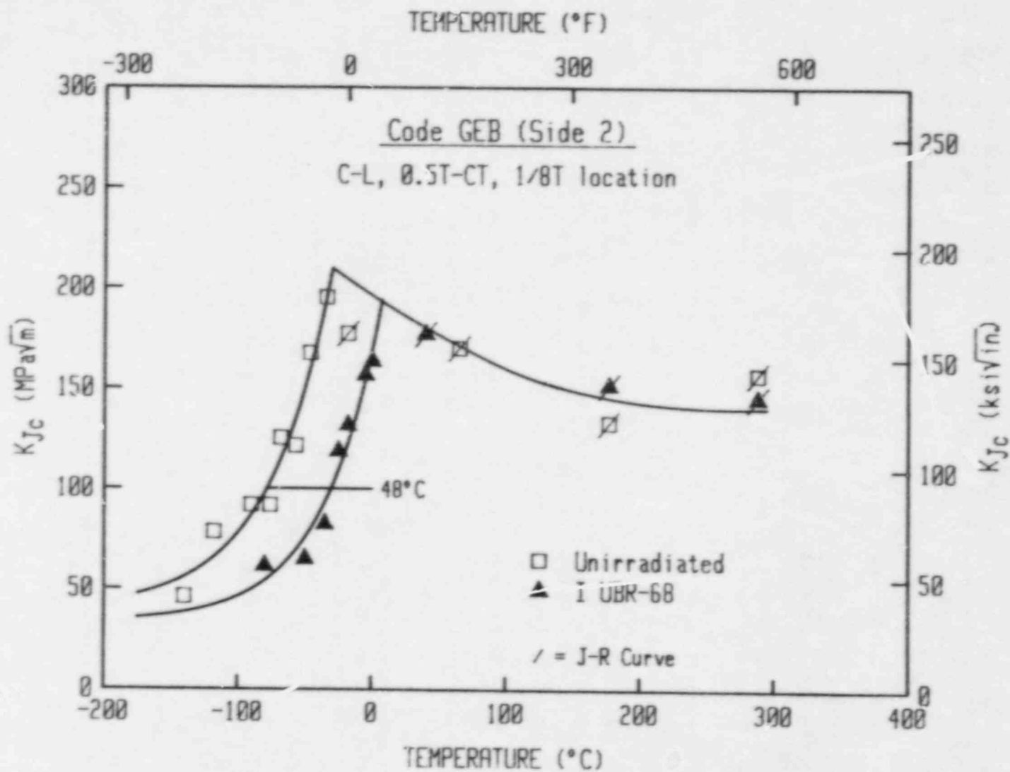
Fig. 10 Fracture toughness of Code GEB-2 material before and after irradiation at 288°C to 8.6 \times 10^{18} n/cm 2 (Experiment UBR-68).
