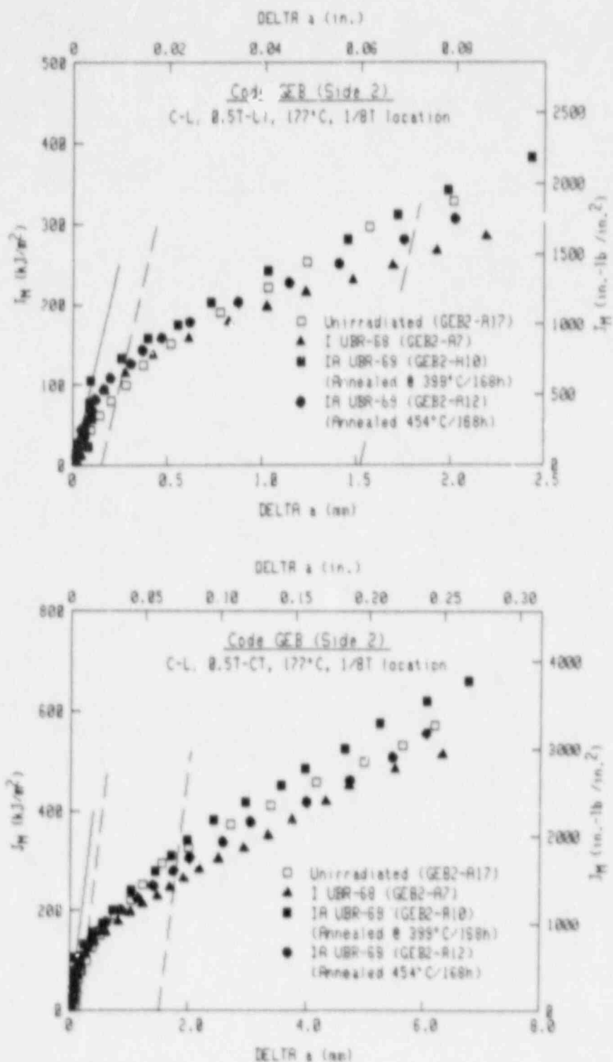
Fig. 16 J-R curves for unirradiated, UBR-68 irradiated and two postirradiated heat treated conditions at 177°C. The tests show similar J-R curve levels; the lowest curve is for the as-irradiated condition.
