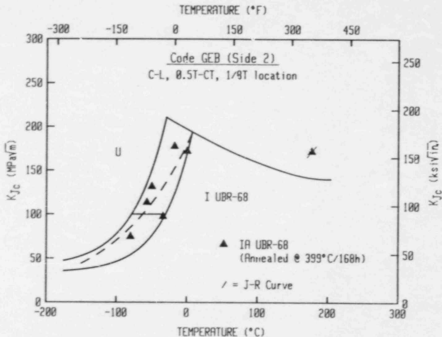
Fig. 14 Fracture toughness of Code GEB-2 material before and after postirradiation annealing at 399°C for 168 h. Individual data points show a variation in transition temperature ranging from 0% to 80% (Experiment UBR-68).
