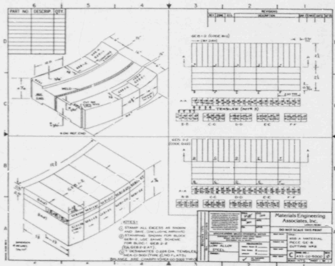
Fig. 2 Cutting Plan for removal of Charpy-V ( C_v ) and tensile (T) specimens from the quarter thickness region of Ring GEB (Base Metals GEB-1 and GEB-2).
