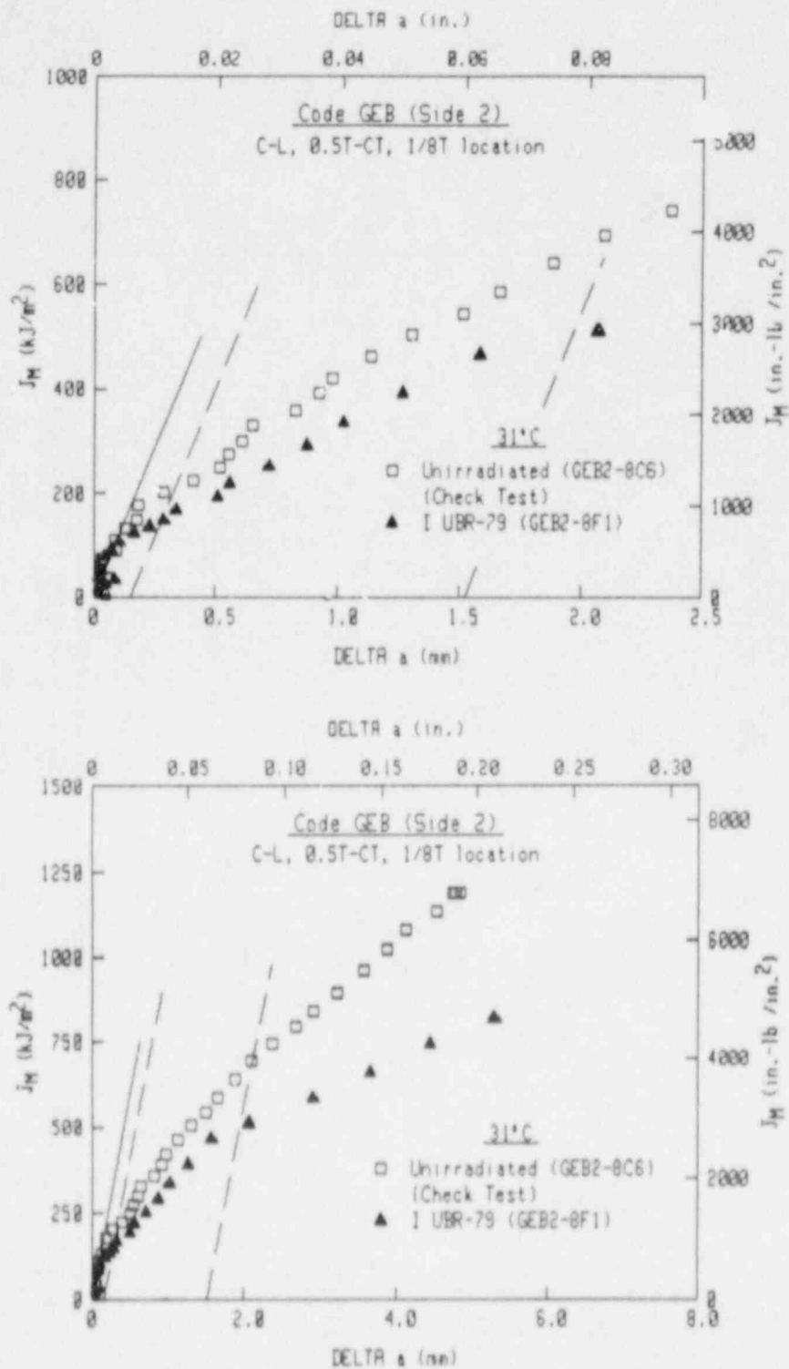
Fig. 31 J-R curves for unirradiated vs. UBR-79 irradiated conditions at 31°C. A fairly large reduction in J level is evident for the irradiated condition.
