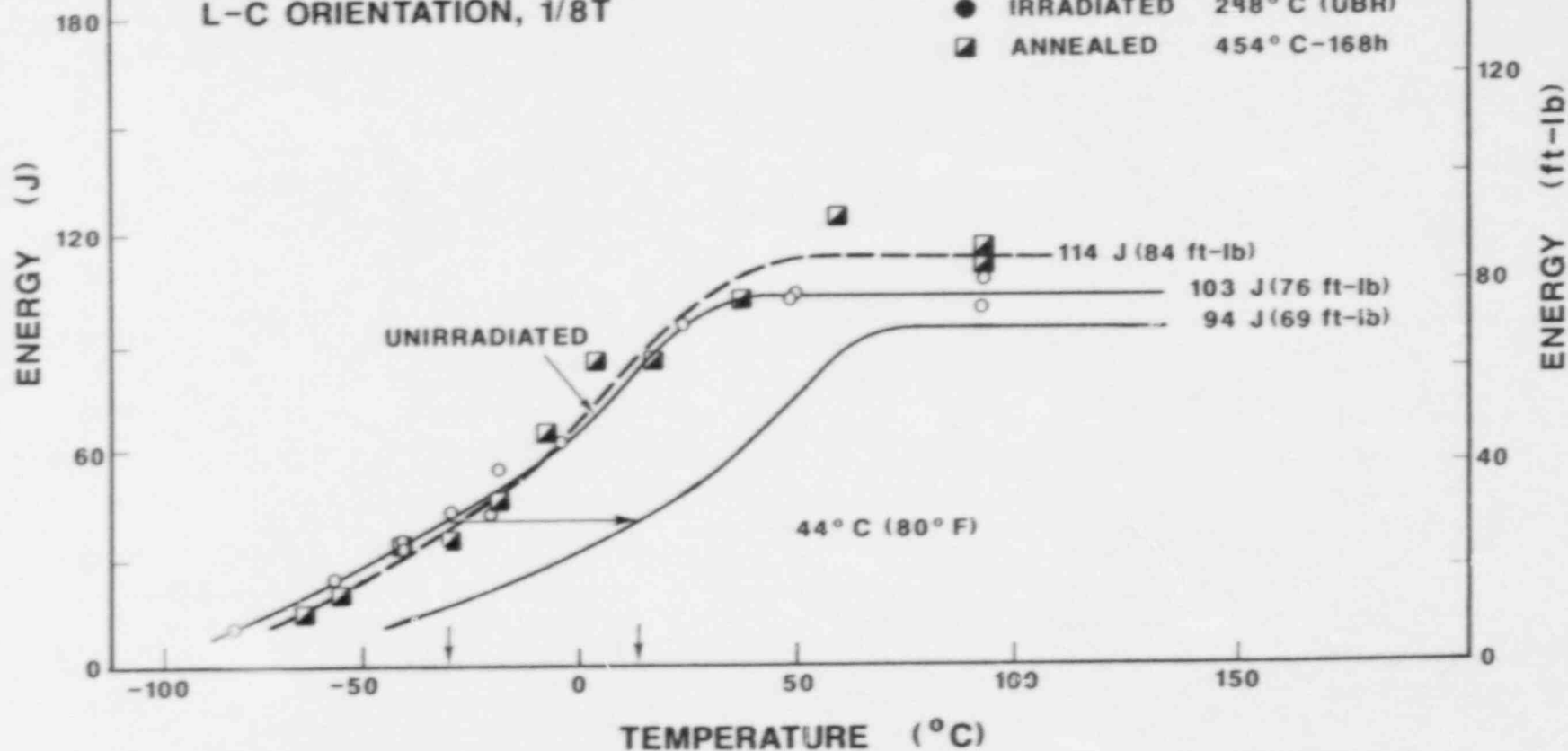
Fig. 9 Charpy-V notch ductility of Code GEB-2 material before and after postirradiation annealing at 454 ^{\circ}\text{C} for 168 h (Experiment UBR-68).
