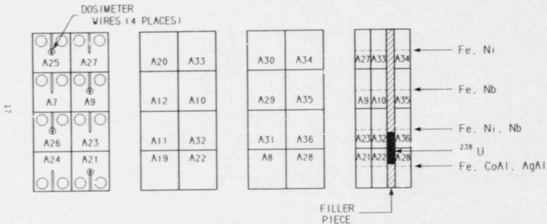
Fig. 6a Placement of Charpy-V, tensile and 0.5T-CT specimens in Experiment UBR-68 (Capsule A; elevation view).
