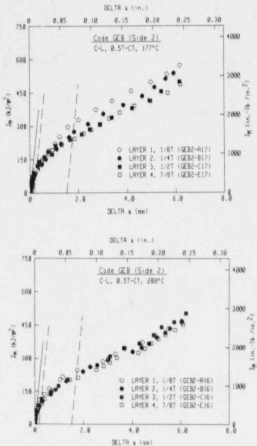
Fig. 4 J-R curves for four thickness locations in the Code GEB-2 material at 177°C and at 288°C.
