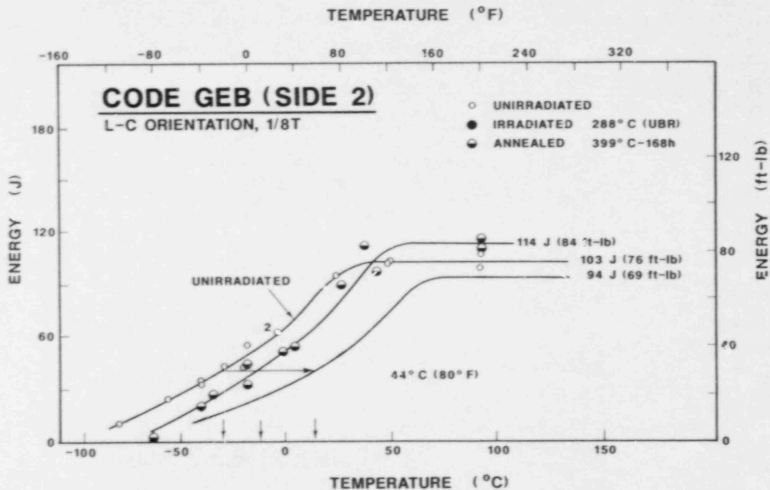
Fig. 8 Charpy-V notch ductility of Code GEB-2 material before and after postirradiation annealing at 399 ^{\circ}\text{C} for 168 h (Experiment UBR-68).
