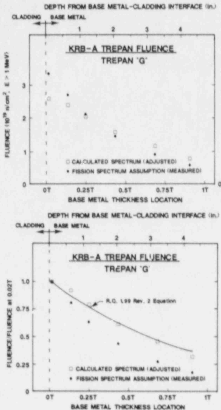
Fig. 18 EG&G Idaho, Inc. fluence measurements for through-thickness positions in Trepan G. The upper graph compares the calculated spectrum vs. assumed fission spectrum determinations; the lower graph shows measured vs. projected through-thickness fluence attenuation. (Note: 1 in. = 25.4 mm)
