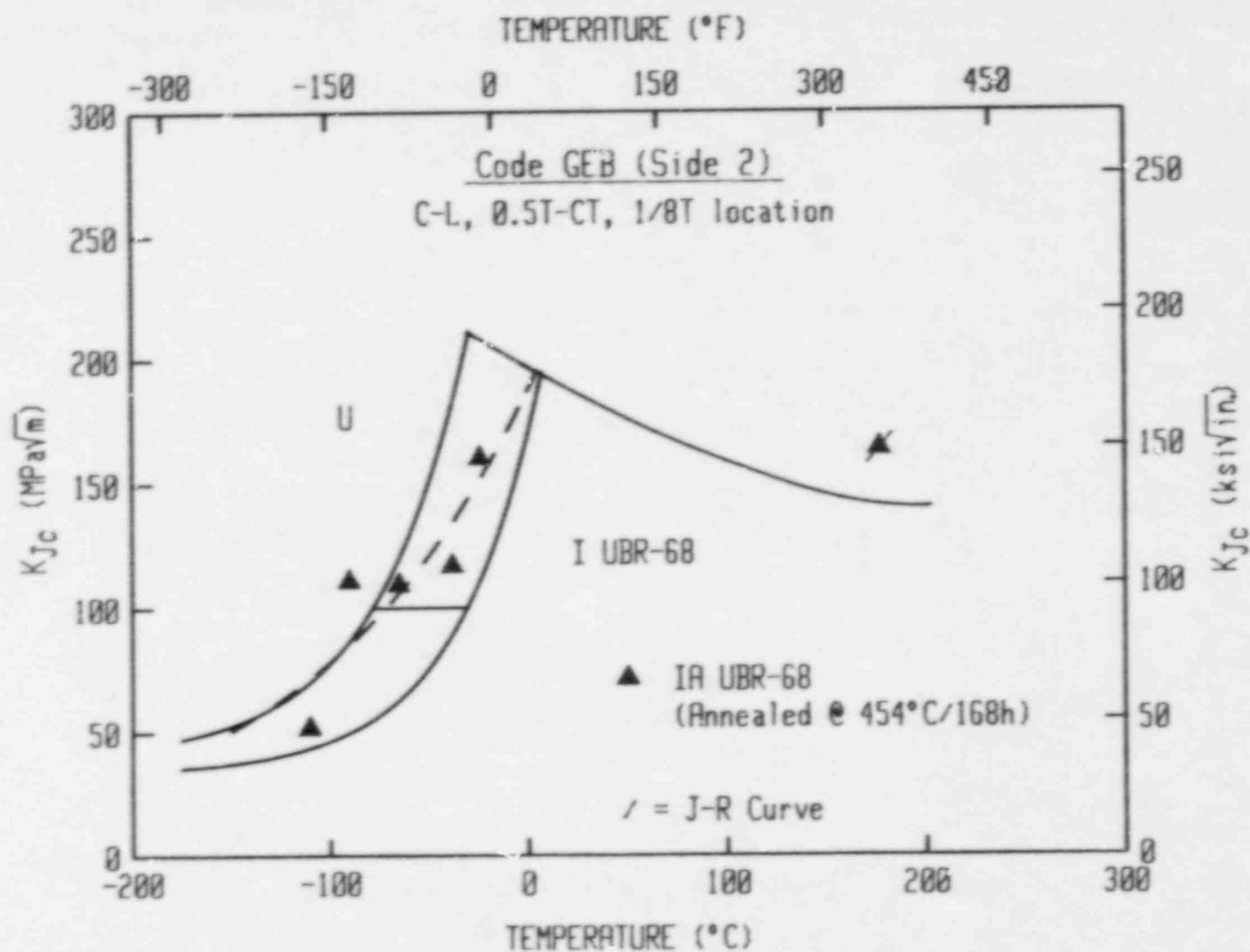
Fig. 15 Fracture toughness of Code GEB-2 material before and after postirradiation annealing at 454°C for 168 h. The wide variation in transition temperature recovery is not understood (Experiment UBR-68).
