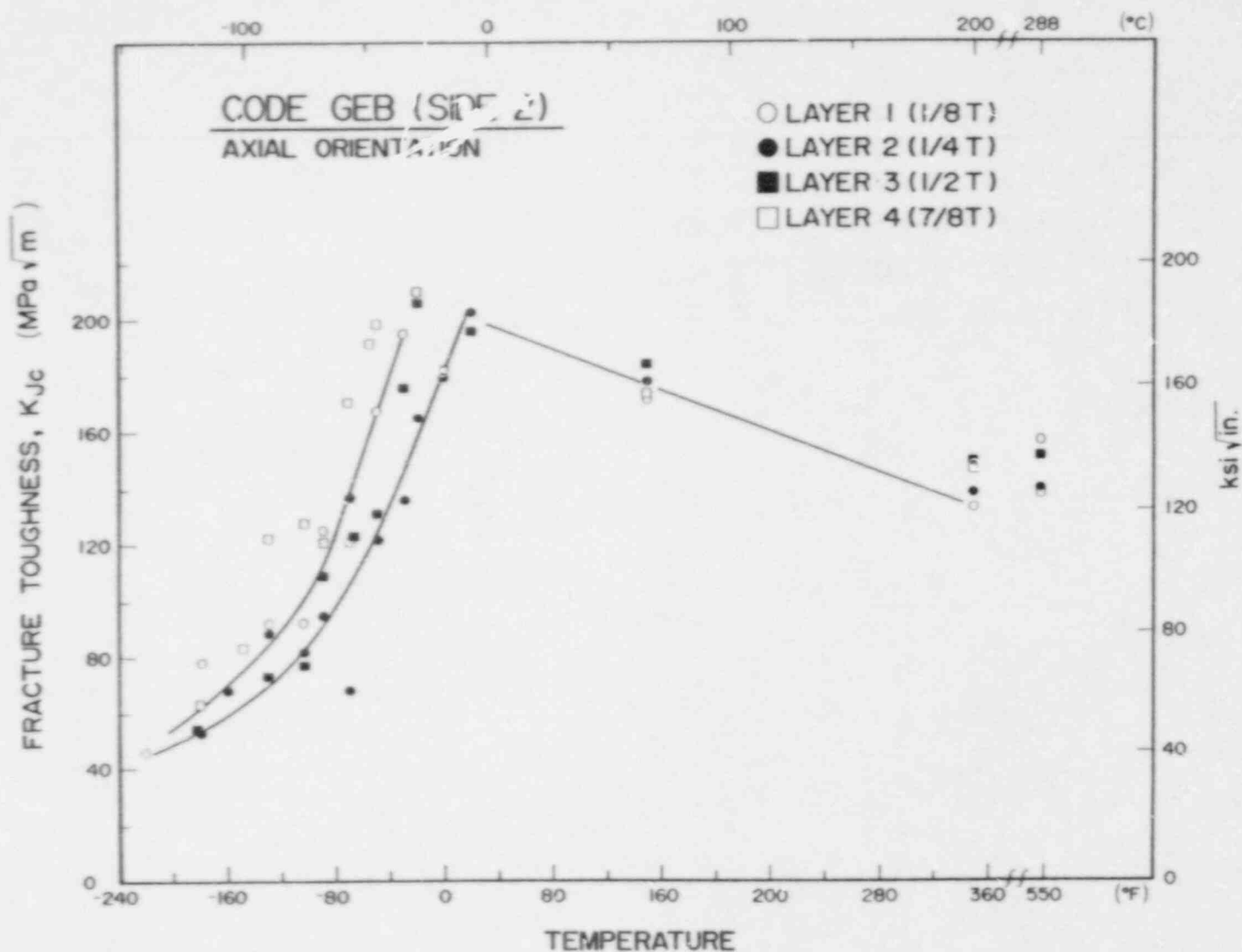
Fig. 8 Fracture toughness of code GEB-2 material at four locations through the thickness.
