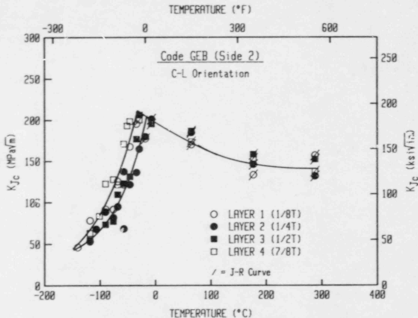
Fig. 3 Fracture toughness of Code GEB-2 material at four thickness locations. Notice the similarity in toughness vs. temperature trends. Tests producing a J-R curve are indicated by a slash (/) through the data point.
