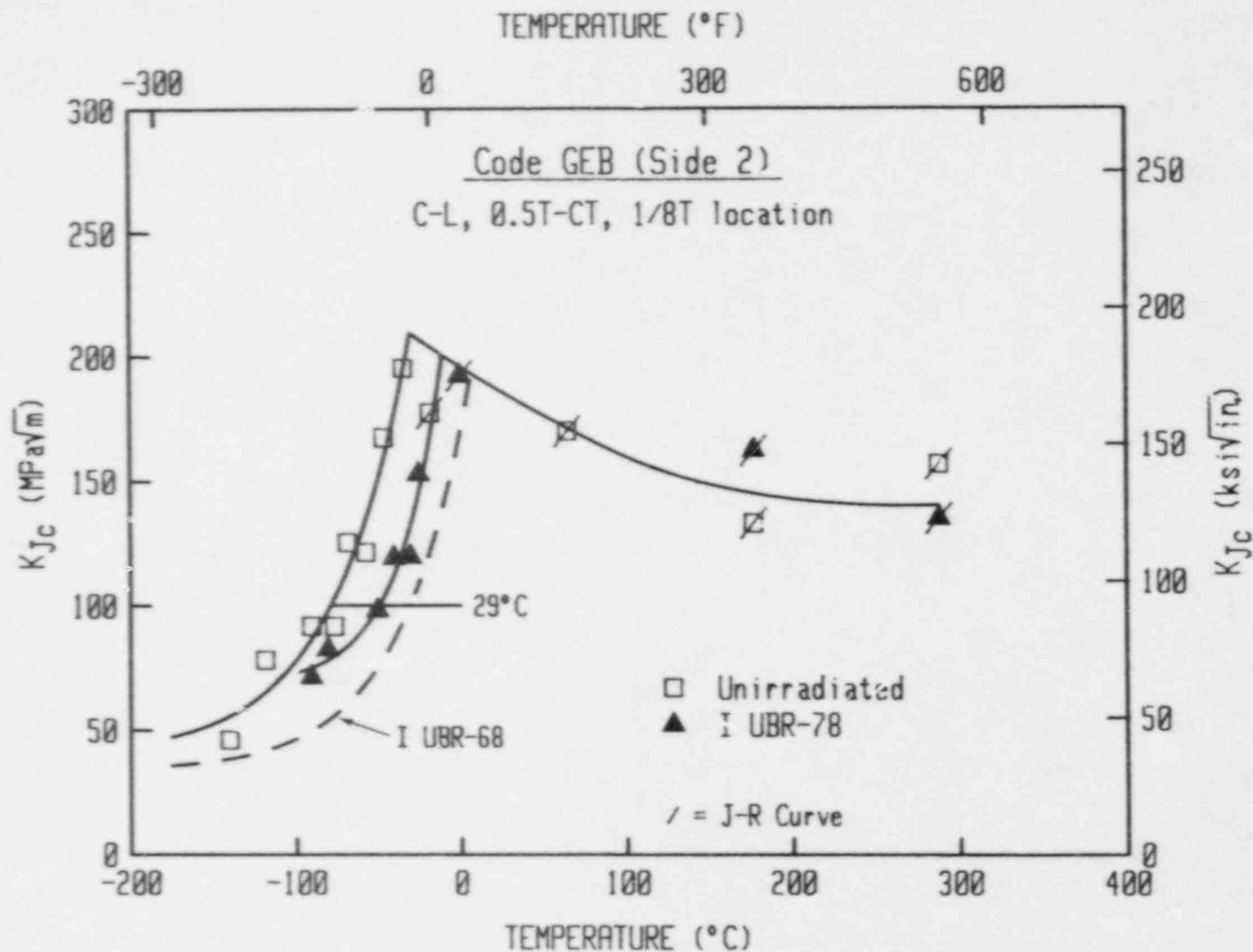
Fig. 26 Fracture toughness of the Code GEB-2 material before and after irradiation at 288°C to 2.6 \times 10^{18} n/cm 2 (Experiment UBR-78). The trend for a 288°C irradiation to 8.6 \times 10^{18} n/cm 2 is also indicated (see dashed curve).
