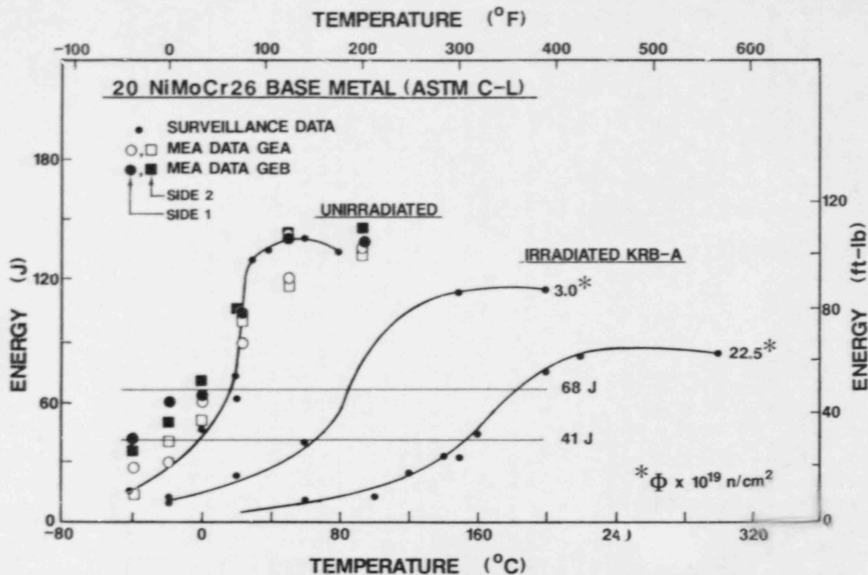
Fig. 1 Charpy-V notch ductility data for the archive base metals vs. data from the KRB-A reactor surveillance program for the same test orientation (ASTM C-L). Surveillance data for two fluence conditions are also shown.
