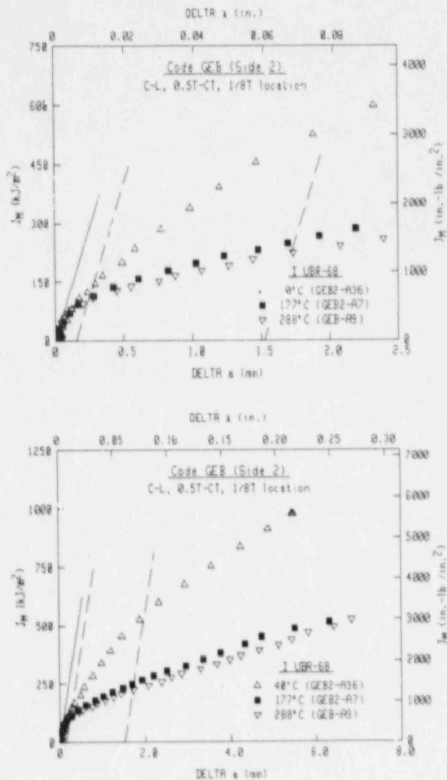
Fig. 13 J-R curves for the UBR-68 irradiated condition at 177°C and 288°C, showing a similarity in toughness level.
