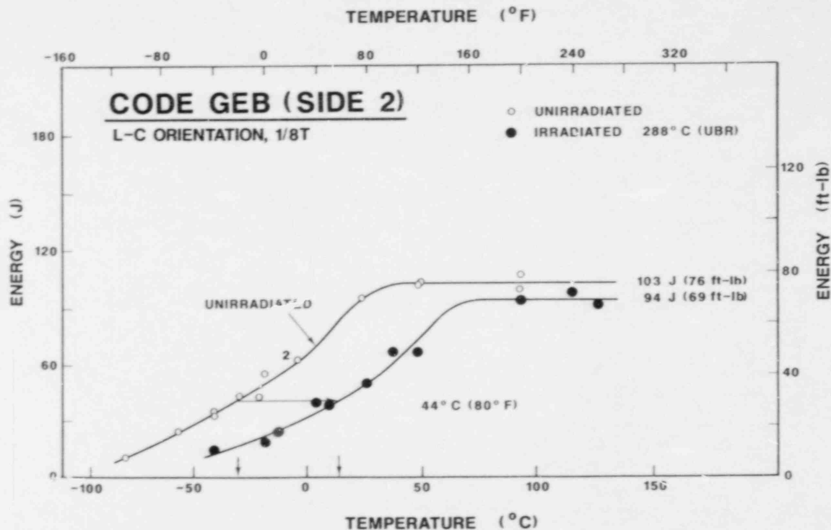
Fig. 7 Charpy-V notch ductility of Code GEB-2 material before and after irradiation at 288°C to 8.8 \times 10^{18} \text{ n/cm}^2 , E > 1 \text{ MeV} . The irradiation was conducted in the light-water-cooled and moderated UBR test reactor (Experiment UBR-68).
