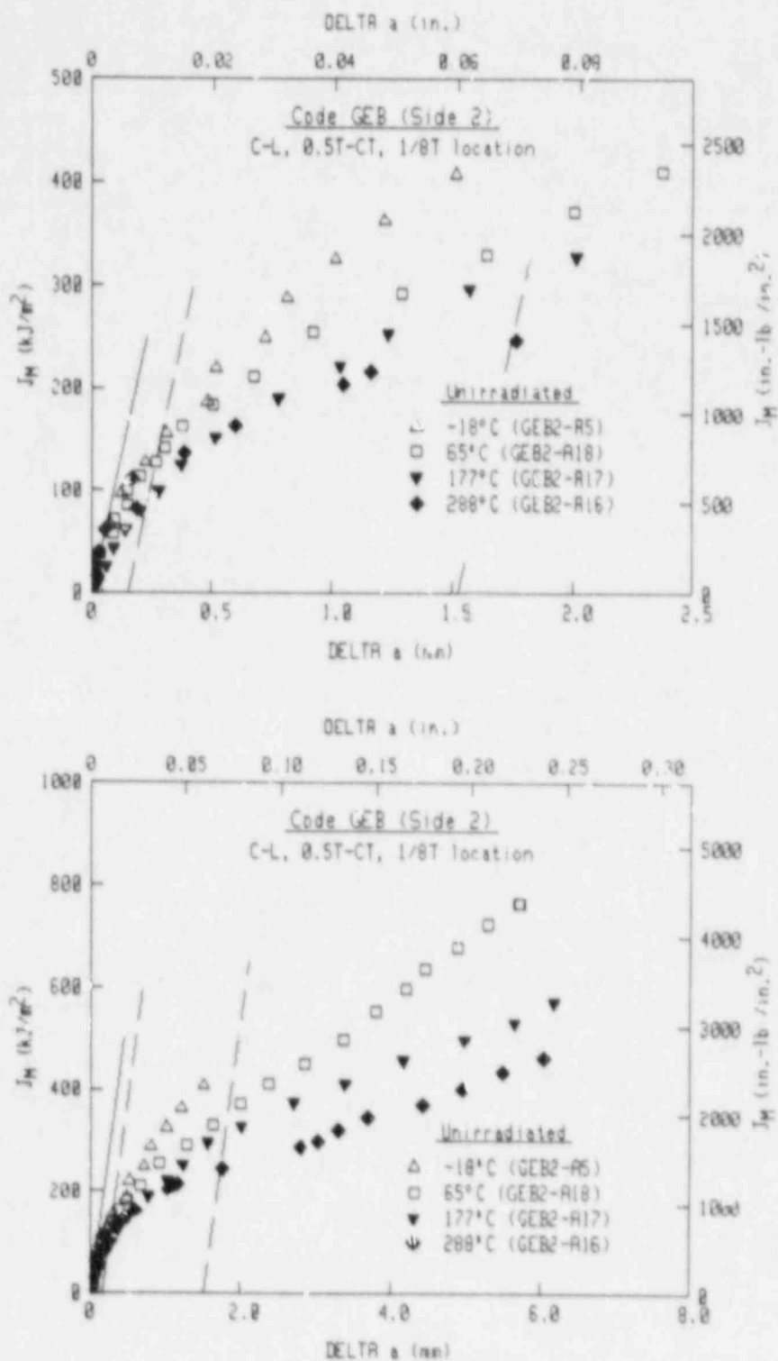
Fig. 5 J-R curves for the Code GEB-2 material showing the dependence of J-R curve level on test temperature. The J-R curve for -18°C (highest level curve) was terminated by cleavage fracture.
