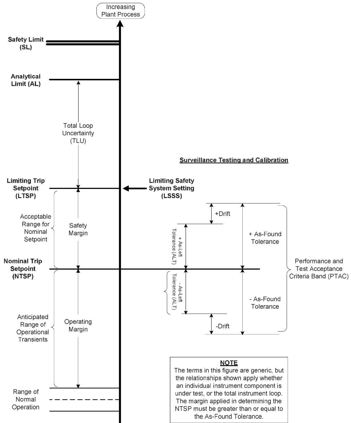
Figure 7.2.7-1: Setpoint relationships during surveillance testing and calibration 4
