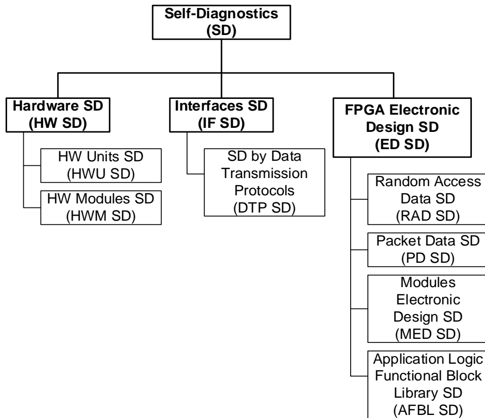
Figure 6-28: Self-Diagnostics Techniques Classification
