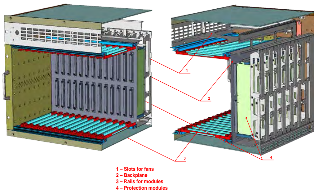
Figure 6-5: RadICS Chassis Design
