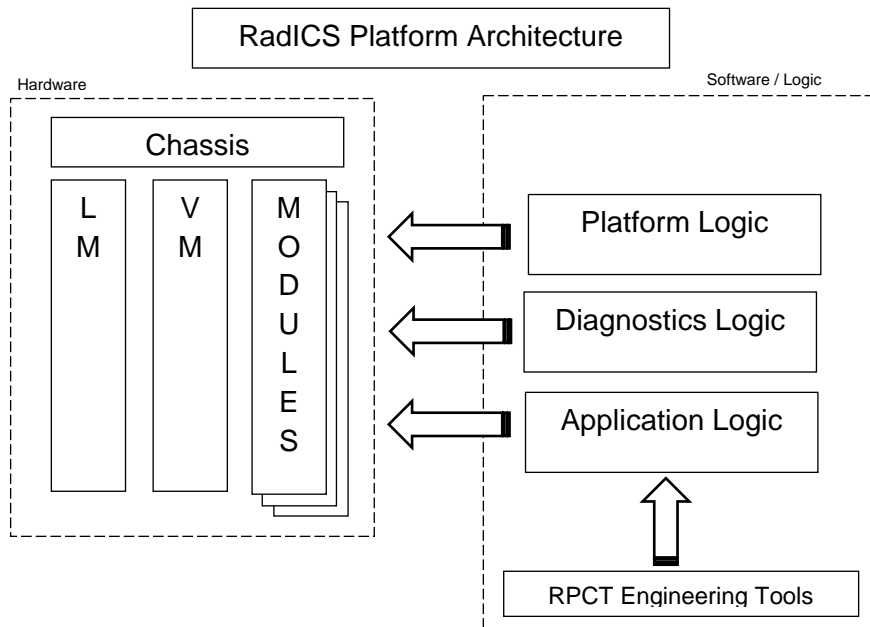
Figure 3.2.2-1: Radics LLC Subsystem Architecture Configuration (Source - Figure 2-3 of RadICS platform TR)
