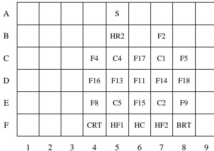
Figure 3-1 MSTR Core 128 Configuration
