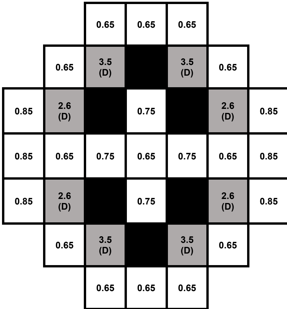
Figure 2.3-8 Loading Pattern 37E2 for MPC-37 Containing Undamaged and Damaged Fuel in DFCs/DFIs, “Long” Fuel per Cell Heat Load Limits
