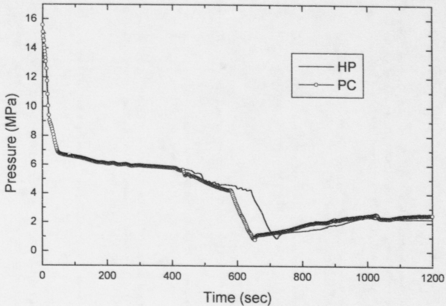
Figure 1 System Pressure
