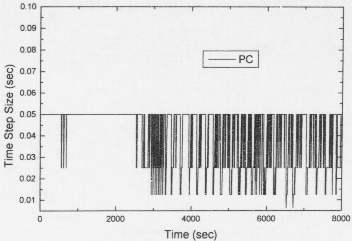
Figure 22 Time Step Size on PC
