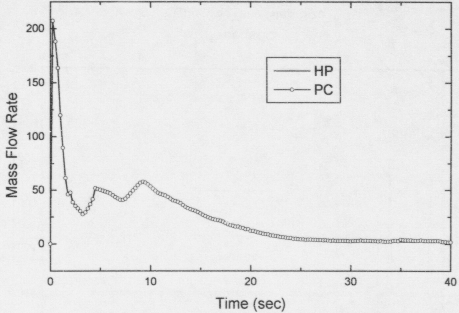
Figure 32 Mass Flow rate at Broken Loop Hot Leg
