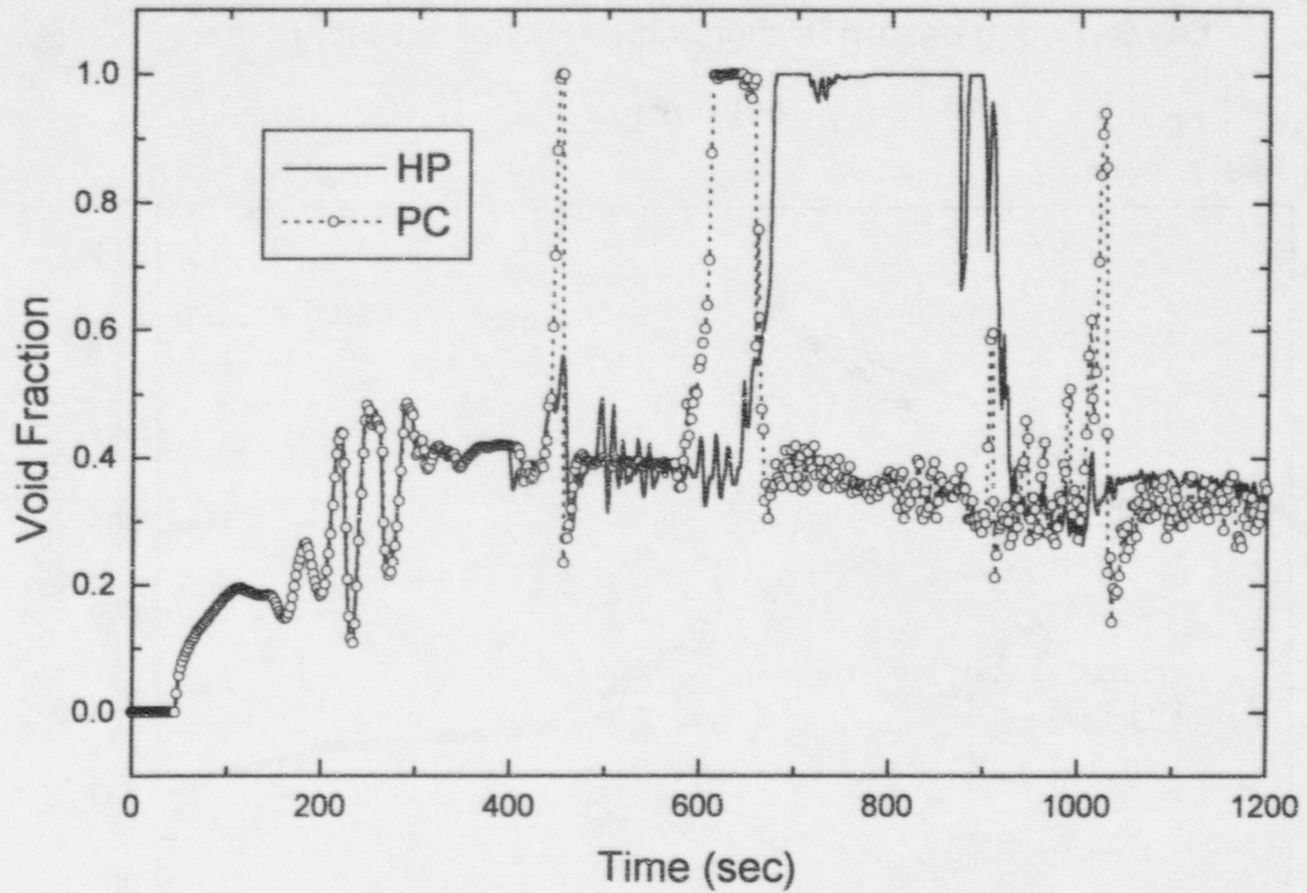
Figure 2 Void Fraction in the Core
