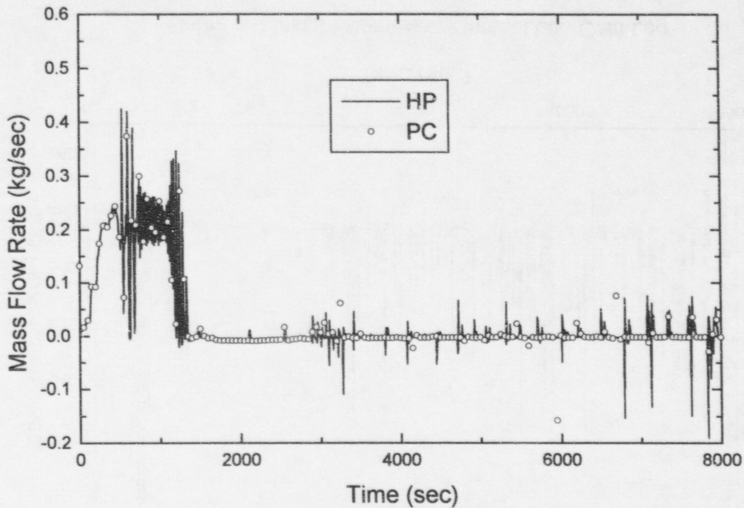
Figure 15 Mass Flow Rate at Broken Loop Cold Leg
