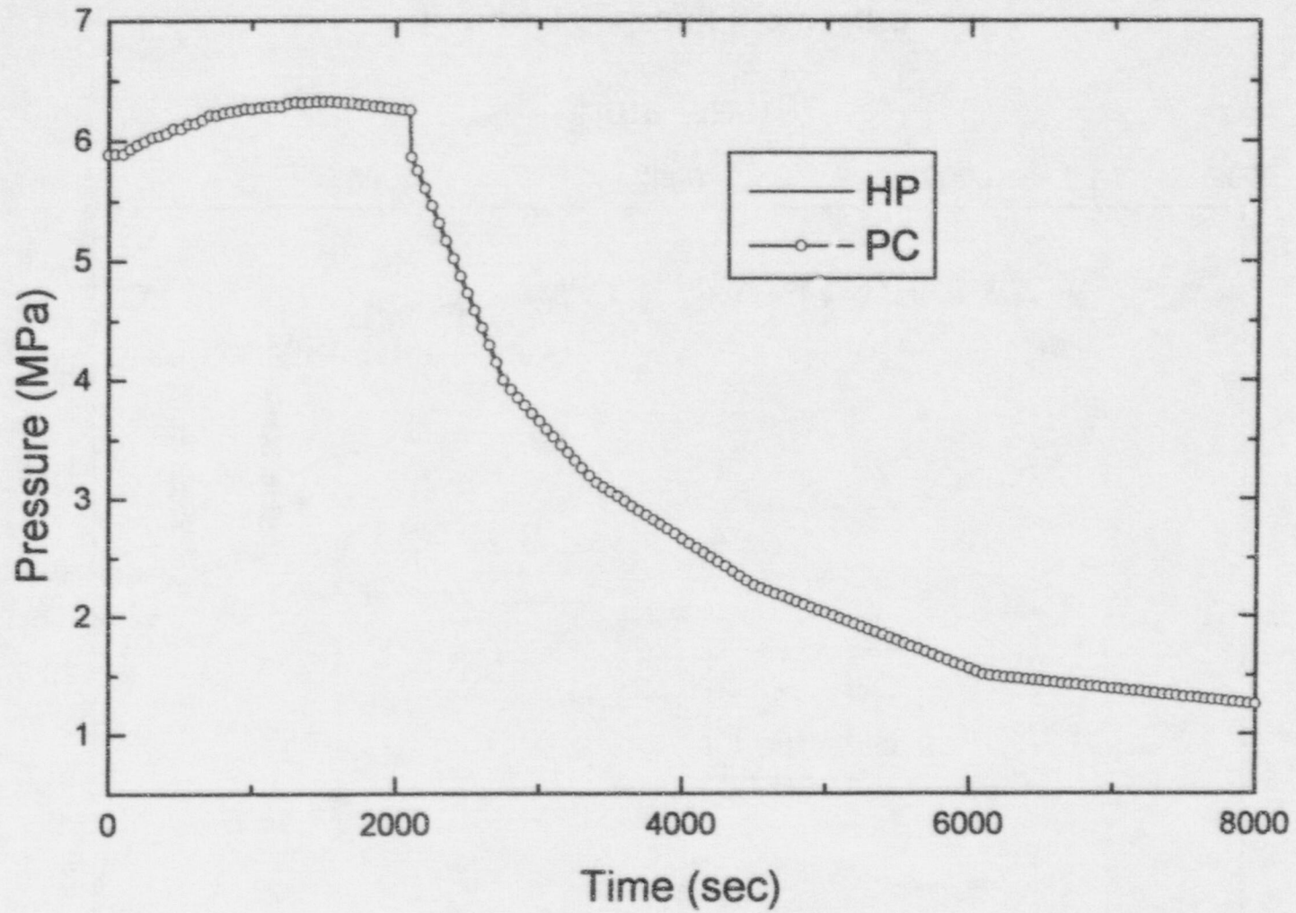
Figure 12 Pressure in Broken Loop S/G
