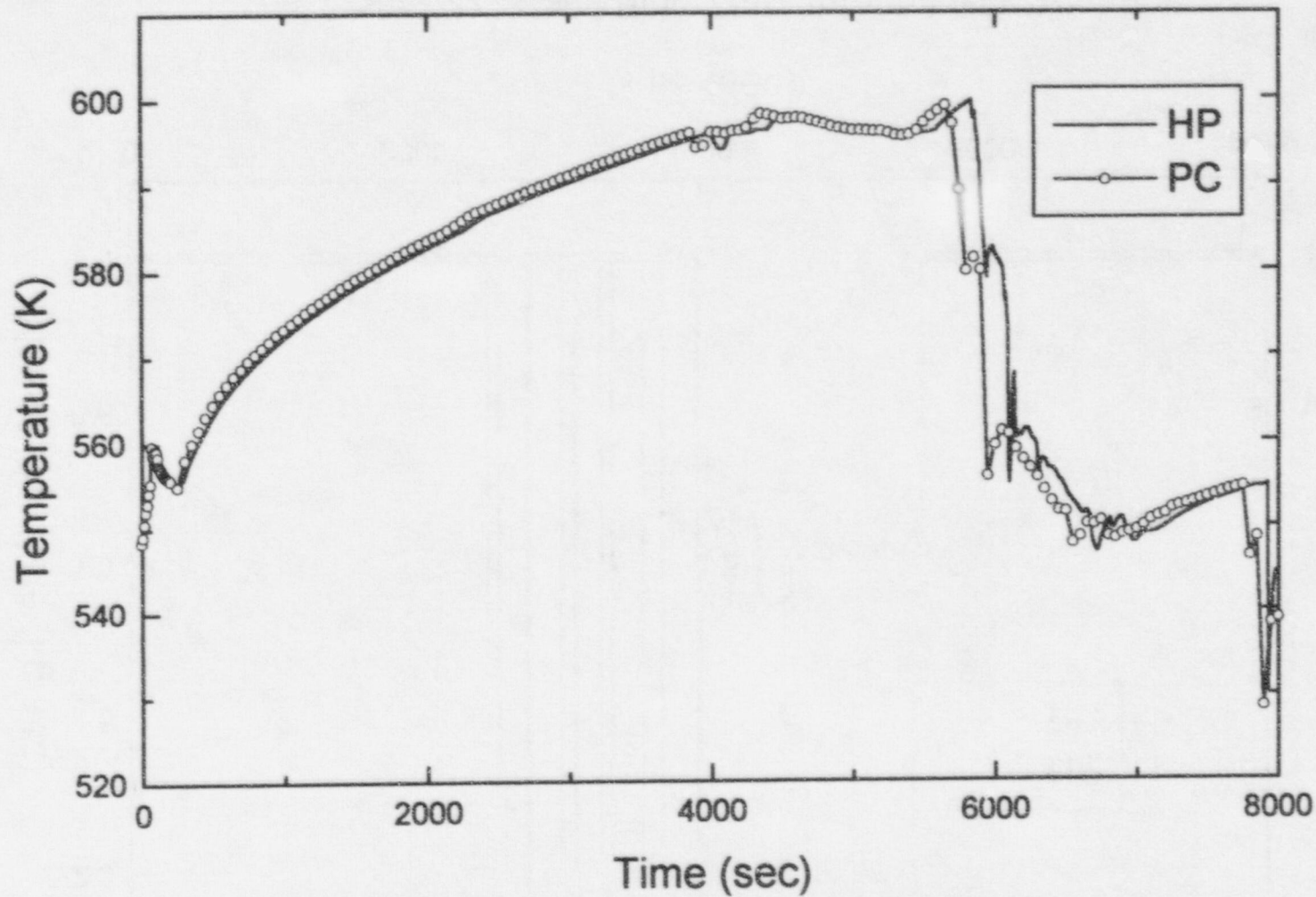
Figure 26 Fluid Temperature at S/G Secondary Side
