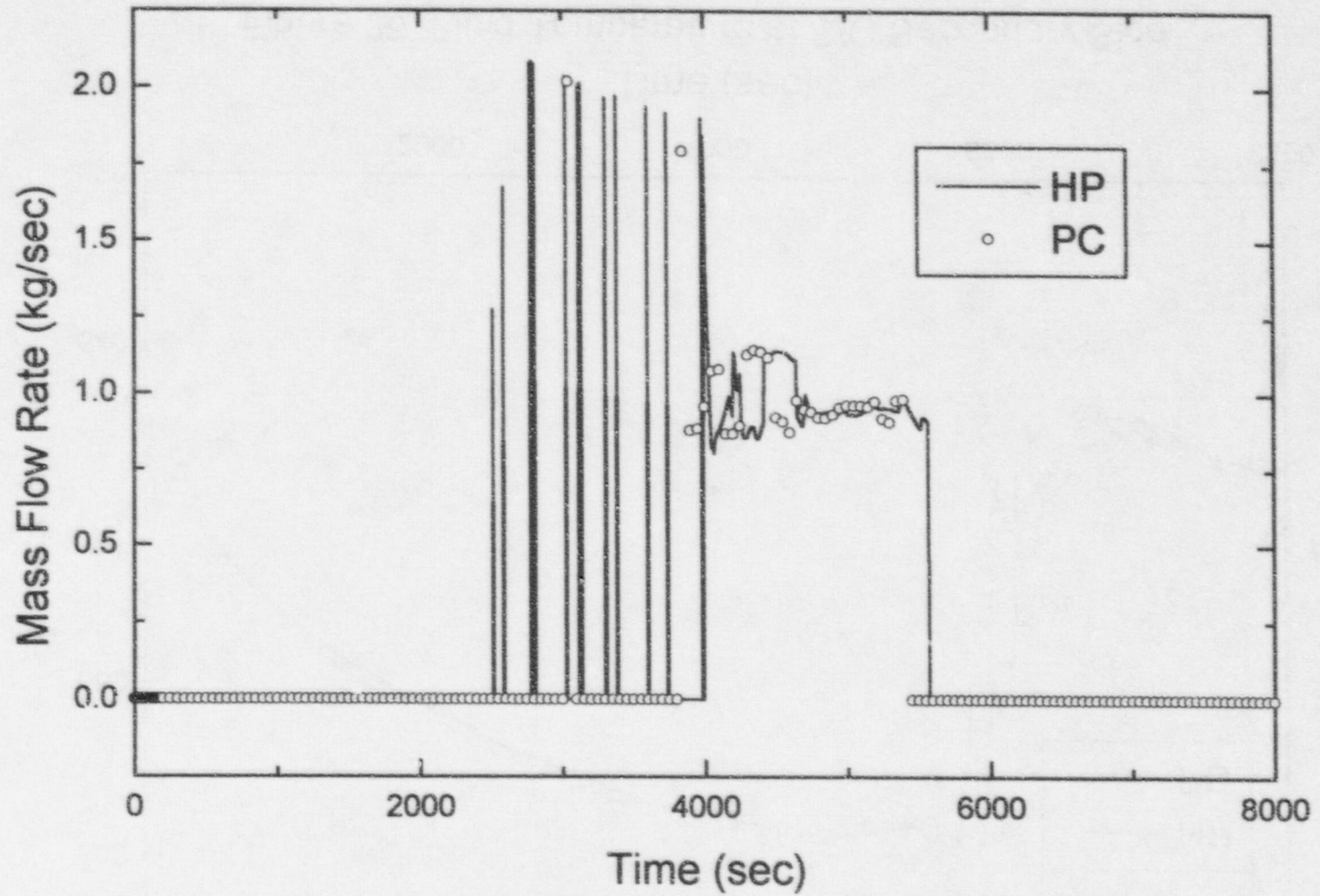
Figure 27 Mass Flow Rate through PORV
