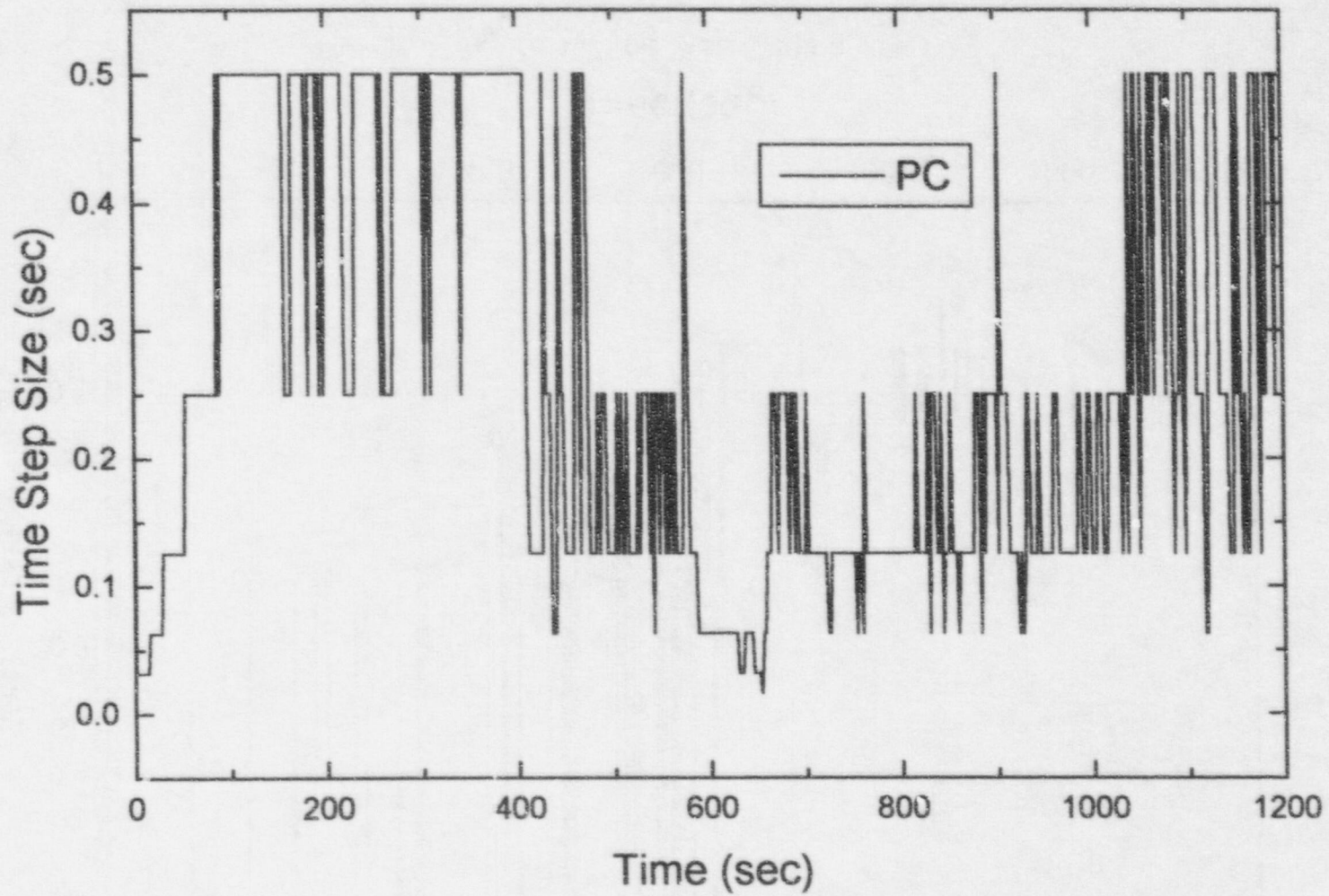
Figure 5 Time Step Size on PC
