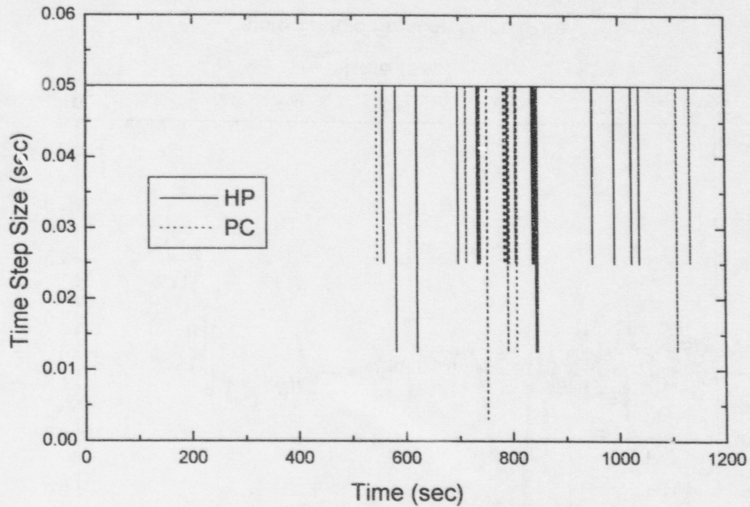
Figure 9 Time Step Size
