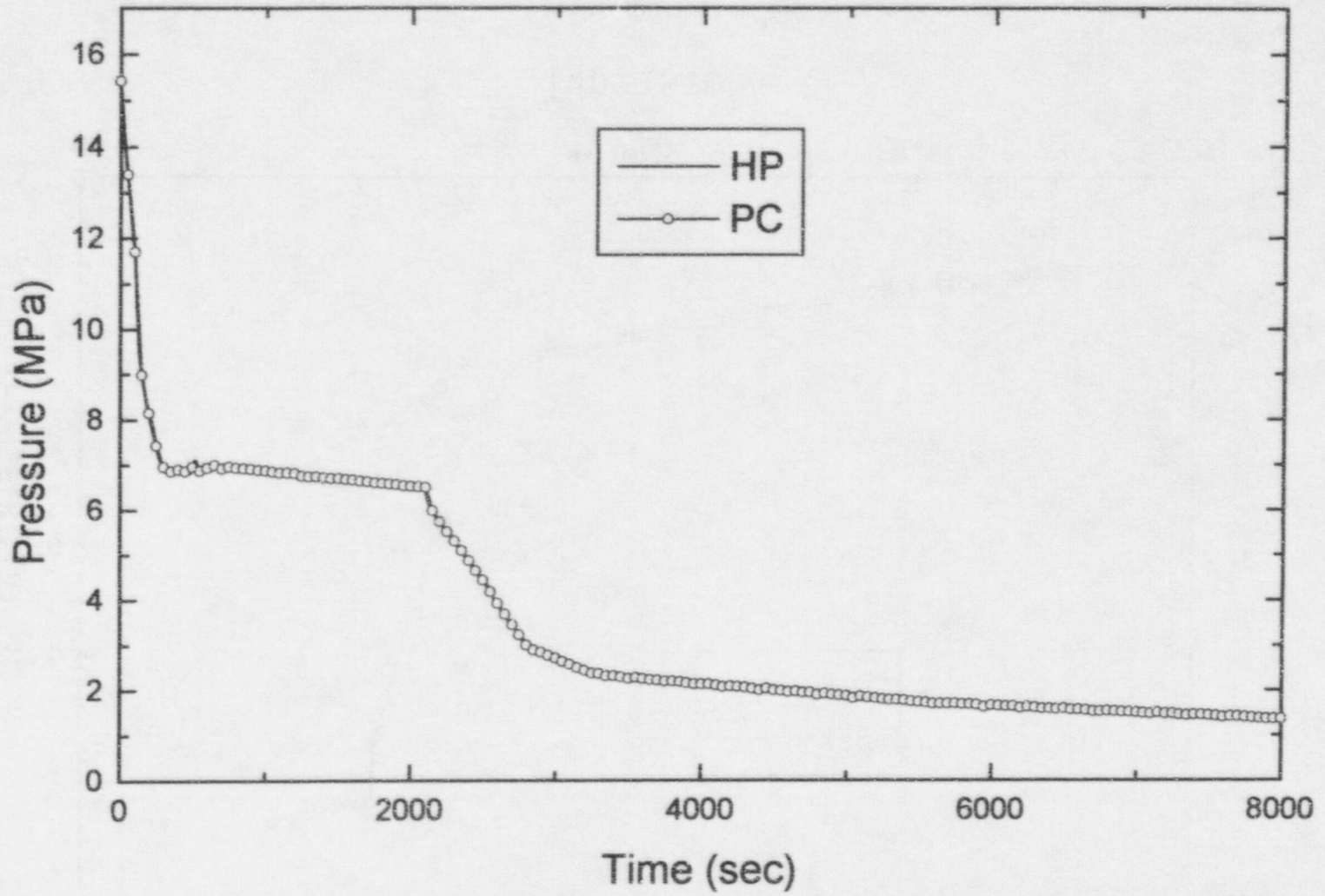
Figure 10 Primary System Pressure
