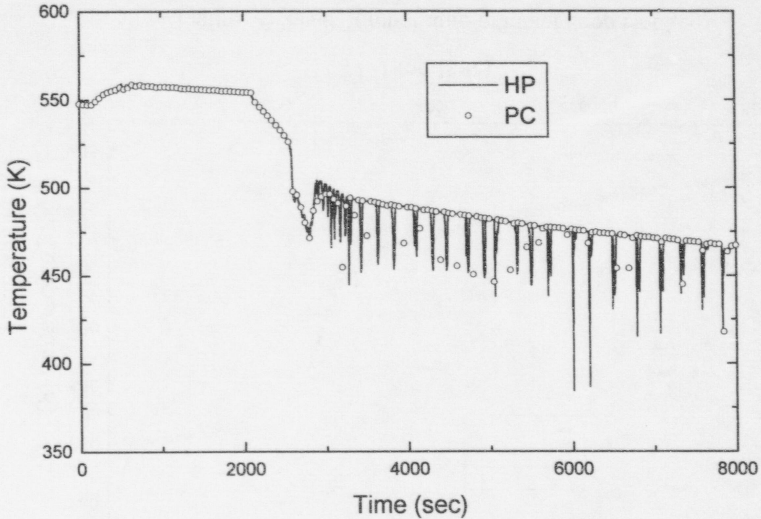
Figure 17 Fluid Temperature at Intact Loop Cold Leg
