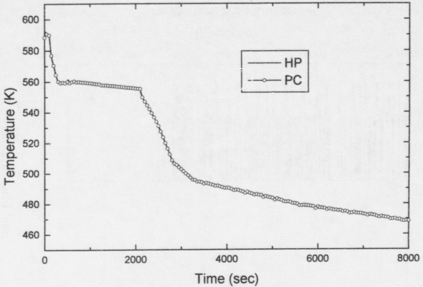
Figure 20 Cladding Temperature at Elevation 291 cm
