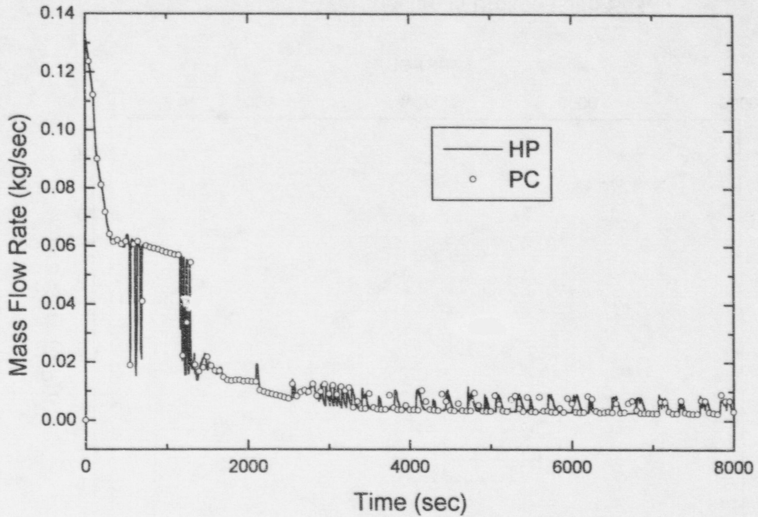
Figure 13 Break Flow Rate
