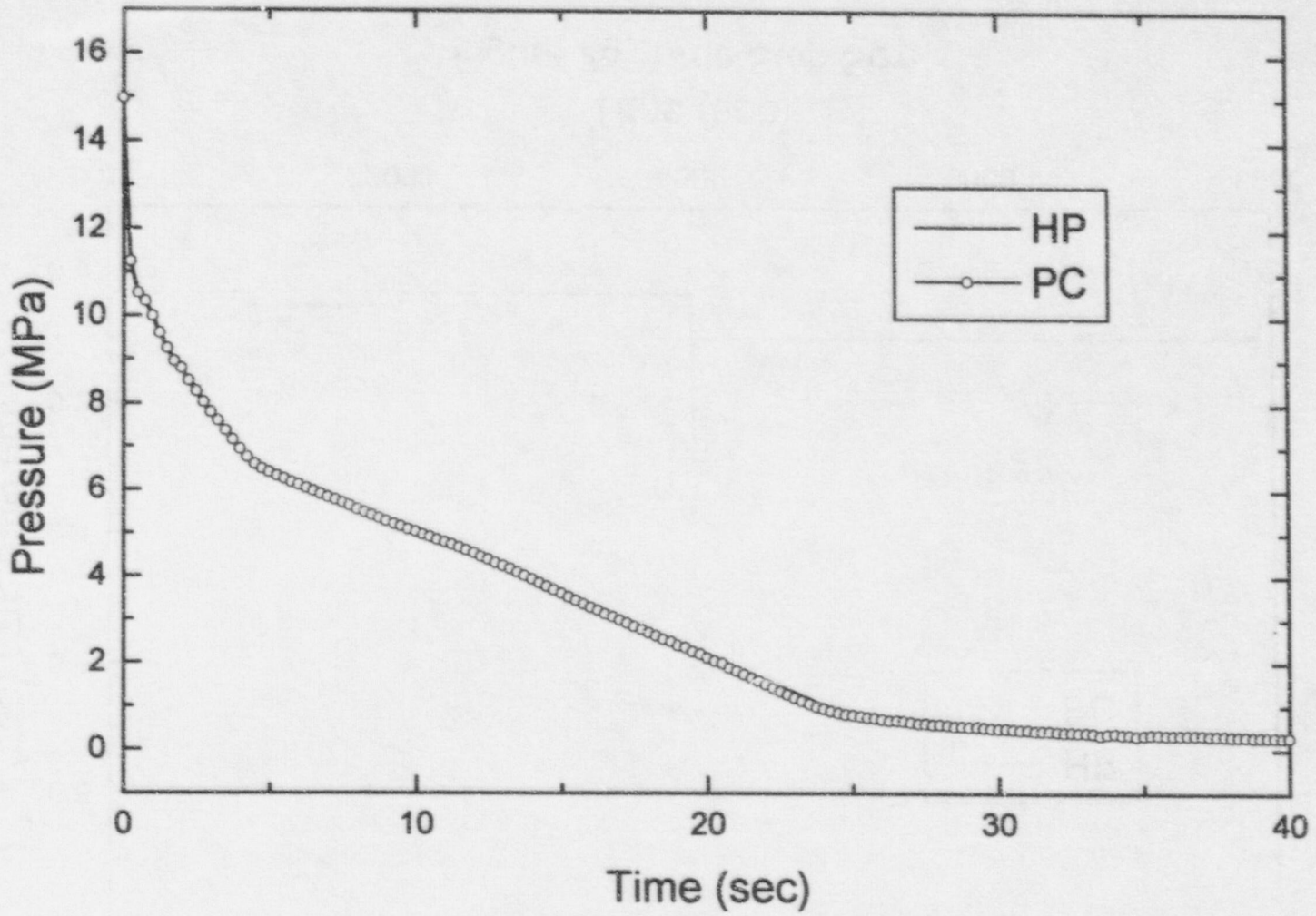
Figure 29 System Pressure
