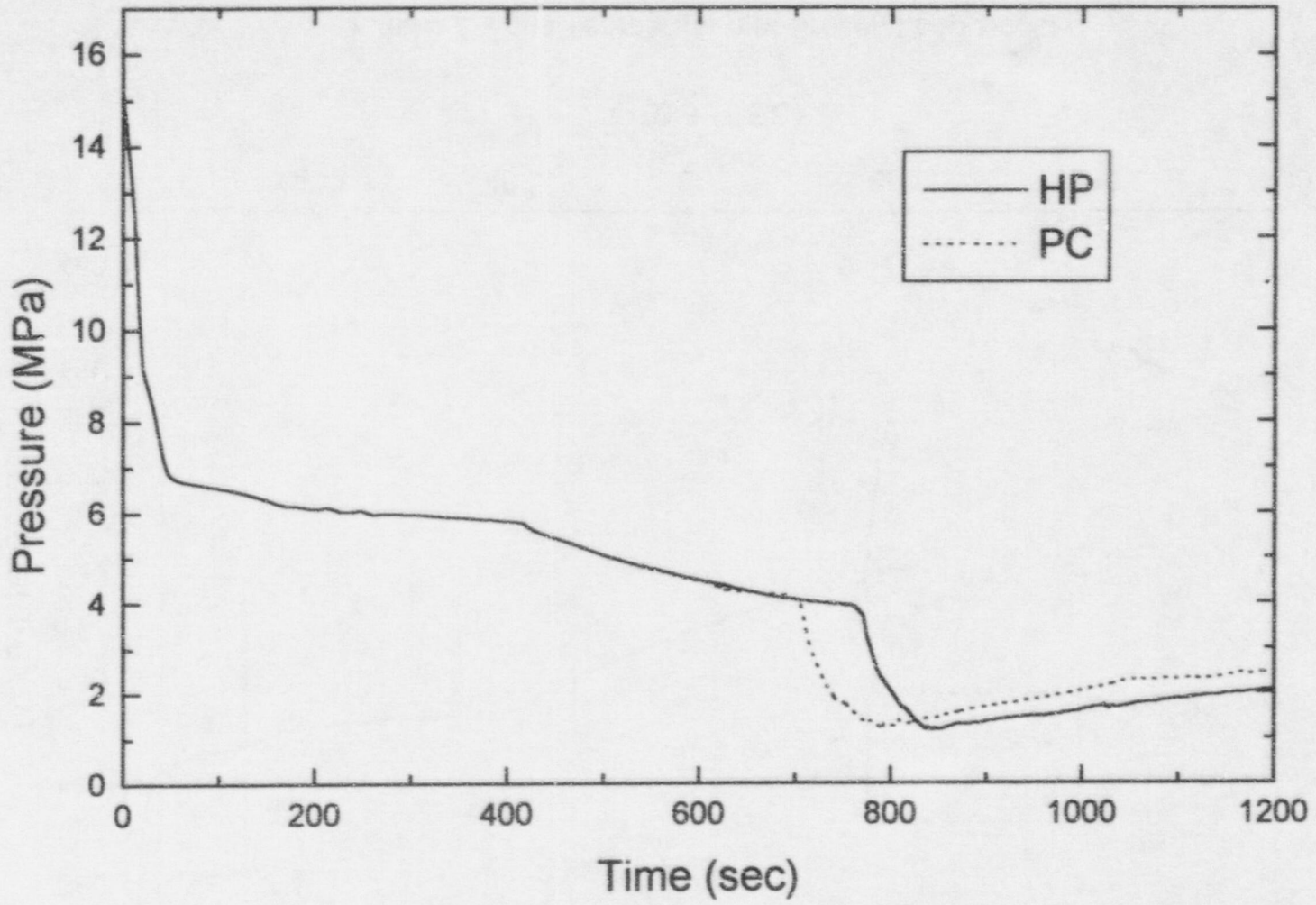
Figure 6 System Pressure
