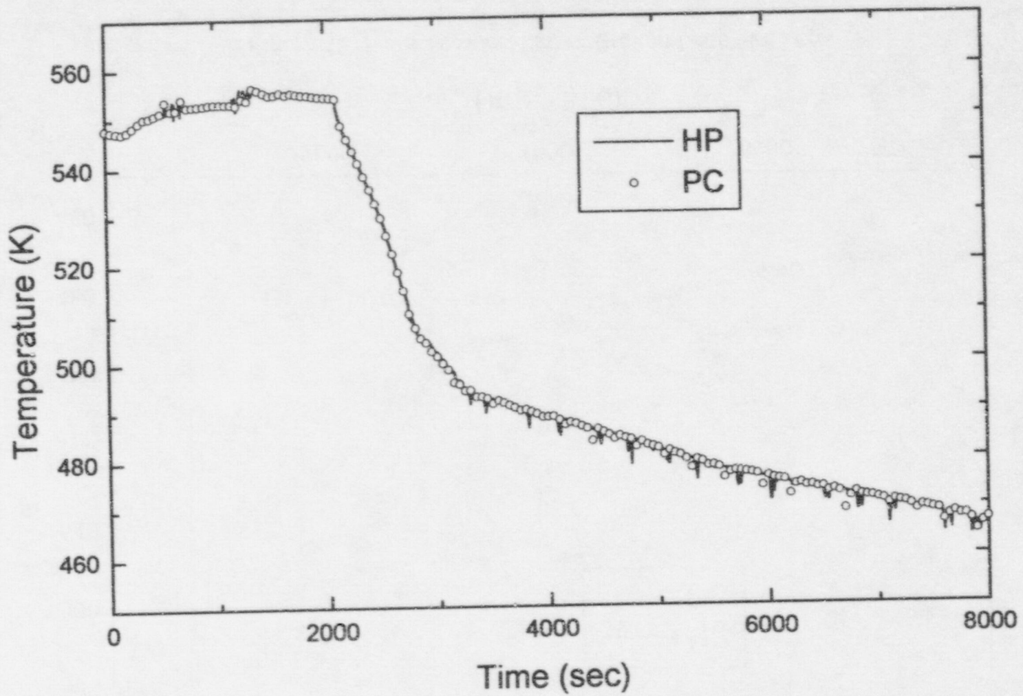
Figure 19 Fluid Temperature at Broken Loop Cold Leg
