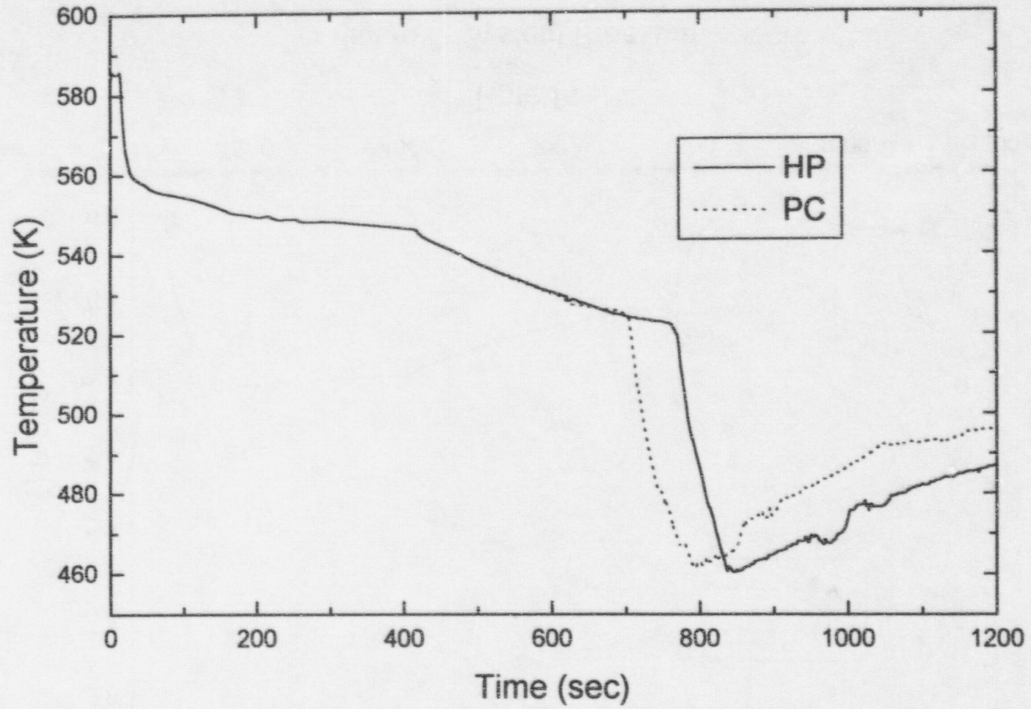
Figure 7 Fluid Temperature at Broken Loop Hot Leg
