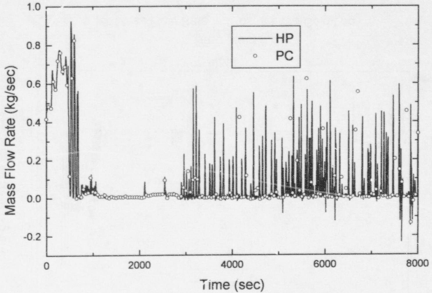
Figure 14 Mass Flow Rate at Intact Loop Cold Leg
