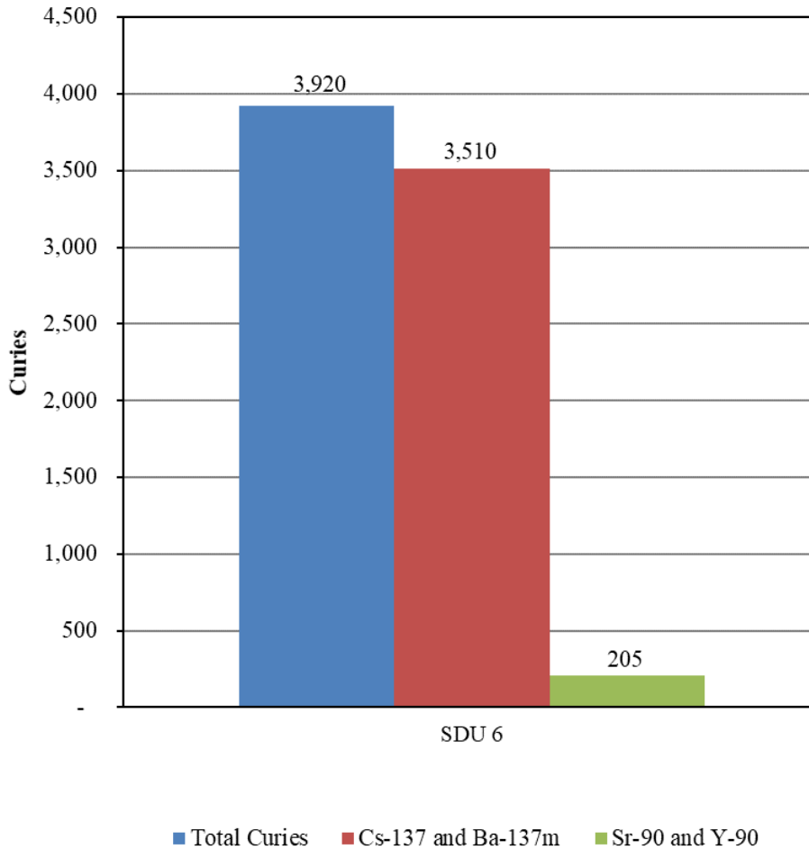
Figure 2-5: Cs-137 and Ba-137m and Sr-90 and Y-90 in Disposed Inventory during FY2019
