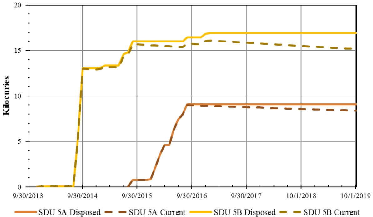
Figure 2-12: SDU 5 Disposed and Current Inventories through FY2019
