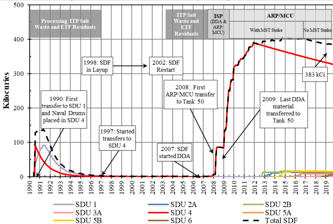
Figure 2-1: SDF Current Inventory through FY2019
