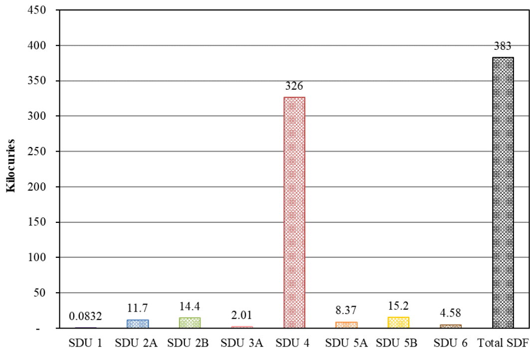
Figure 2-2: Current Inventory of SDUs on September 30, 2019
