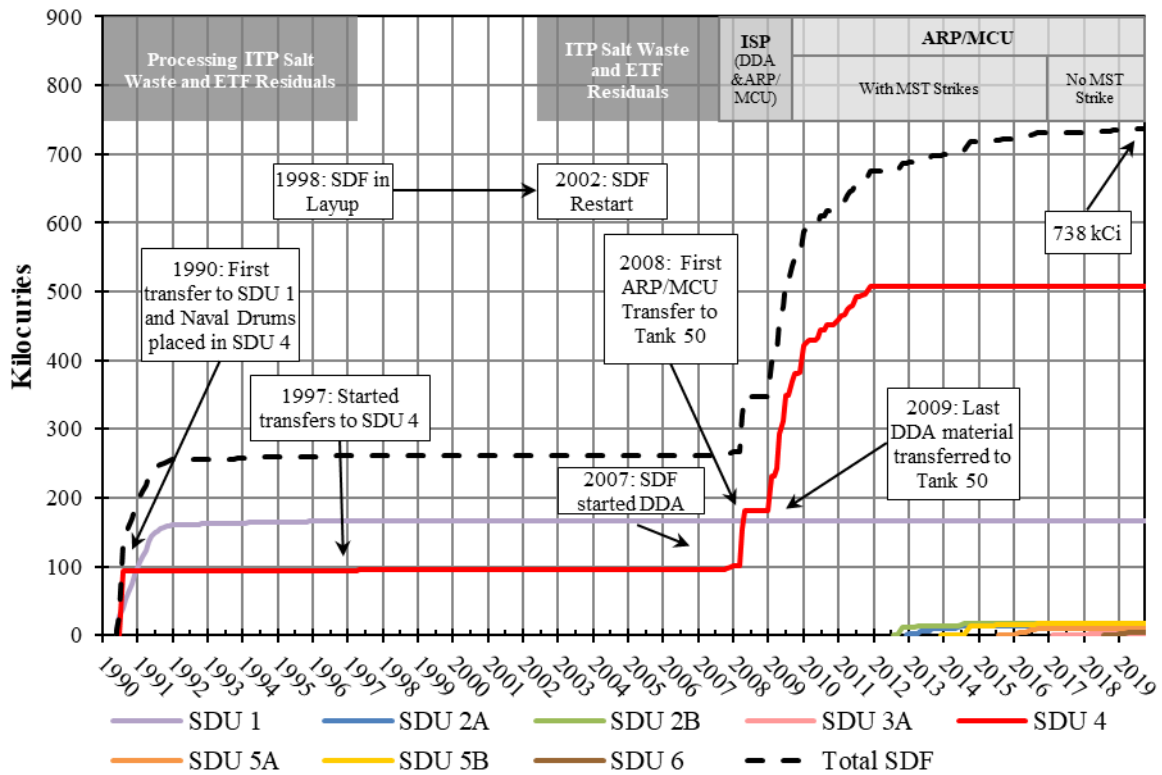
Figure 2-3: SDF Disposed Inventory through FY2019
