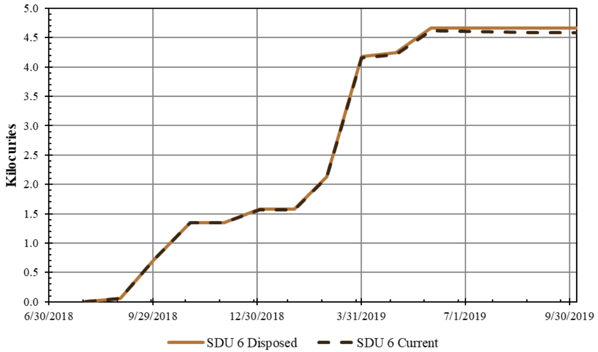
Figure 2-13: SDU 6 Disposed and Current Inventories through FY2019
