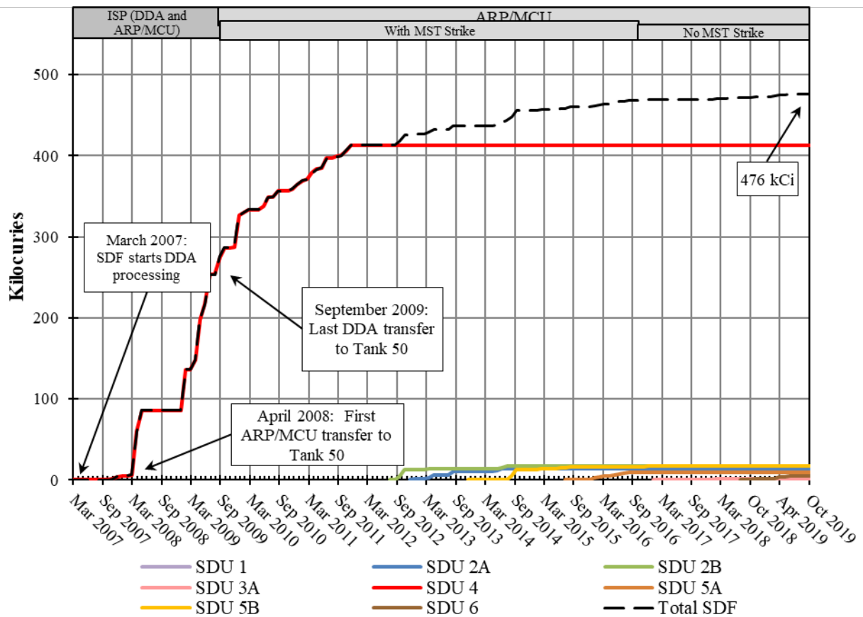
Figure 2-7: Salt Waste Disposed through FY2019 – Beginning with Start of Interim Salt Processing (DDA & ARP/MCU)
