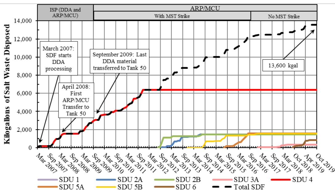
Figure 2-7: Salt Waste Disposed through FY2019 – Beginning with Start of Interim Salt Processing (DDA & ARP/MCU)
