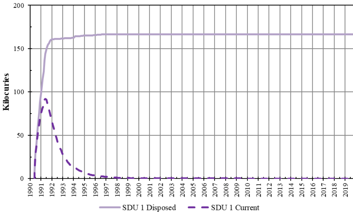
Figure 2-8: SDU 1 Disposed and Current Inventories through FY2019
