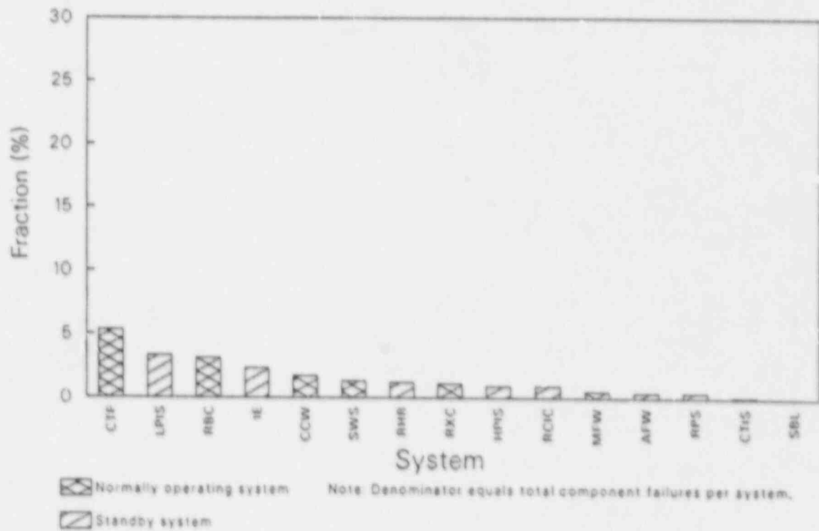
Figure 2b. Fractions of total component failures for specified systems due to aging in circuit breakers.
