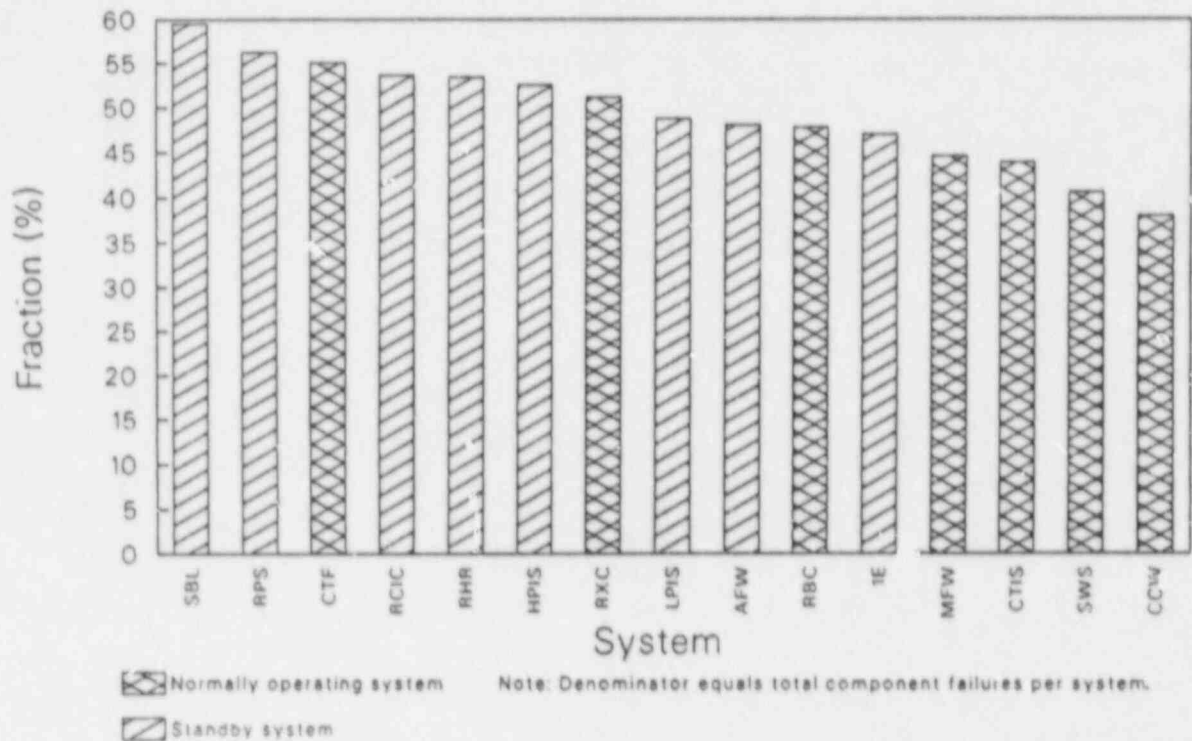
Figure 6. Fractions of the total failures within specified systems which are unknown or categorized as other.
