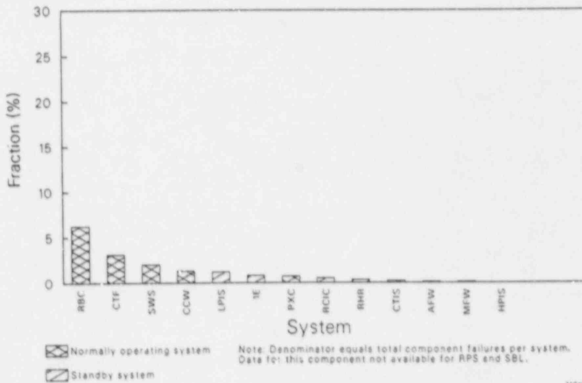
Figure 19. Fractions of total component failures for specified systems due to aging in motors.
