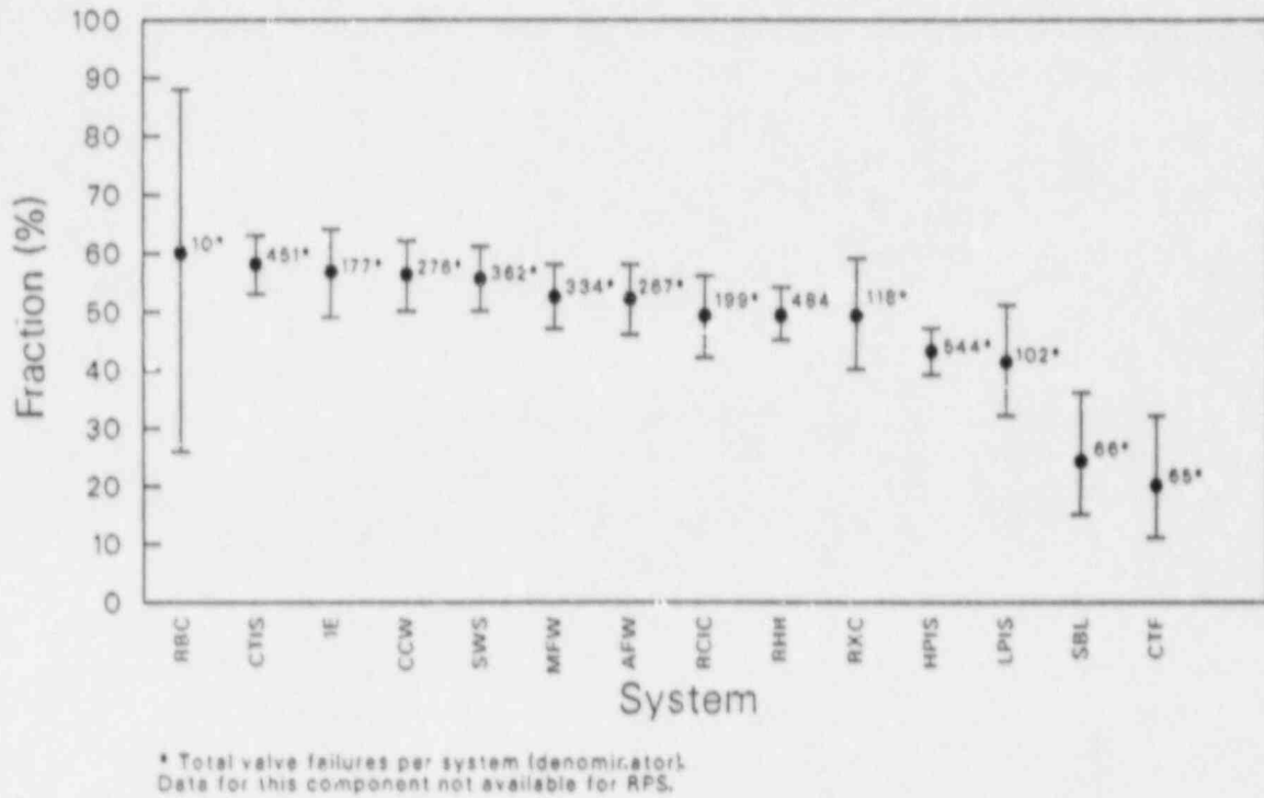
Figure 12. Fractions of valve failures within specified systems due to aging.
