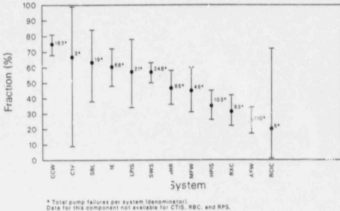
Figure 16. Fractions of pump failures within specified systems due to aging.
