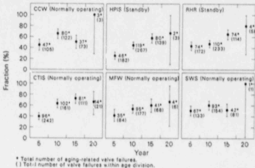
Figure 26. Time-dependent aging fractions for valves.
