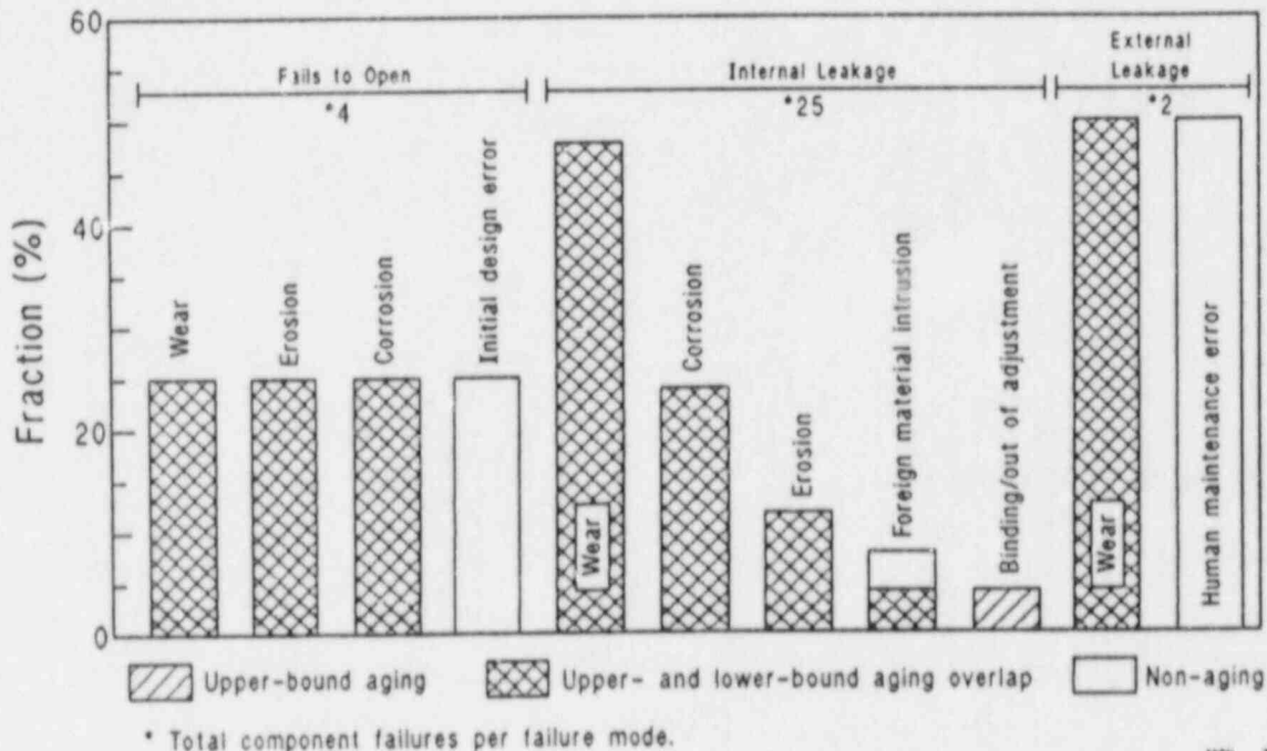
Figure 35. Failure-cause and aging fractions for service water check valves for selected failure modes.
