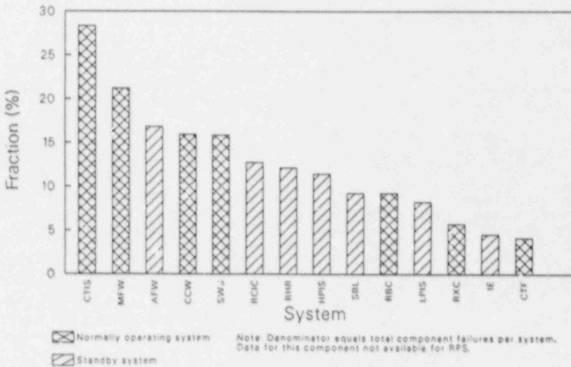
Figure 13. Fractions of total component failures for specified systems due to aging in valves.
