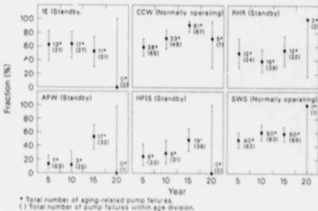
Figure 27. Time-dependent aging fractions for pumps.
