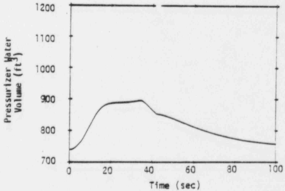
Figure 5 Turbine Trip with Pressure Control - Maximum Feedback - Pressurizer Pressure and Water Volume
