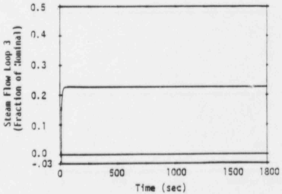
Figure 3 Turbine Trip With Pressure Control - Minimum Feedback - Steam Flow, Loops 2 and 3
