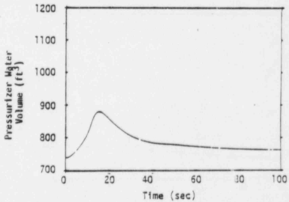
Figure 7 Turbine Trip Without Pressure Control - Minimum Feedback - Pressurizer Pressure and Water Volume
