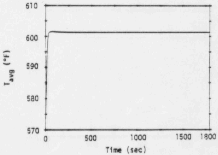
Figure 1 Turbine Trip With Pressure Control - Minimum Feedback - Nuclear Power and Core Average Temperature
