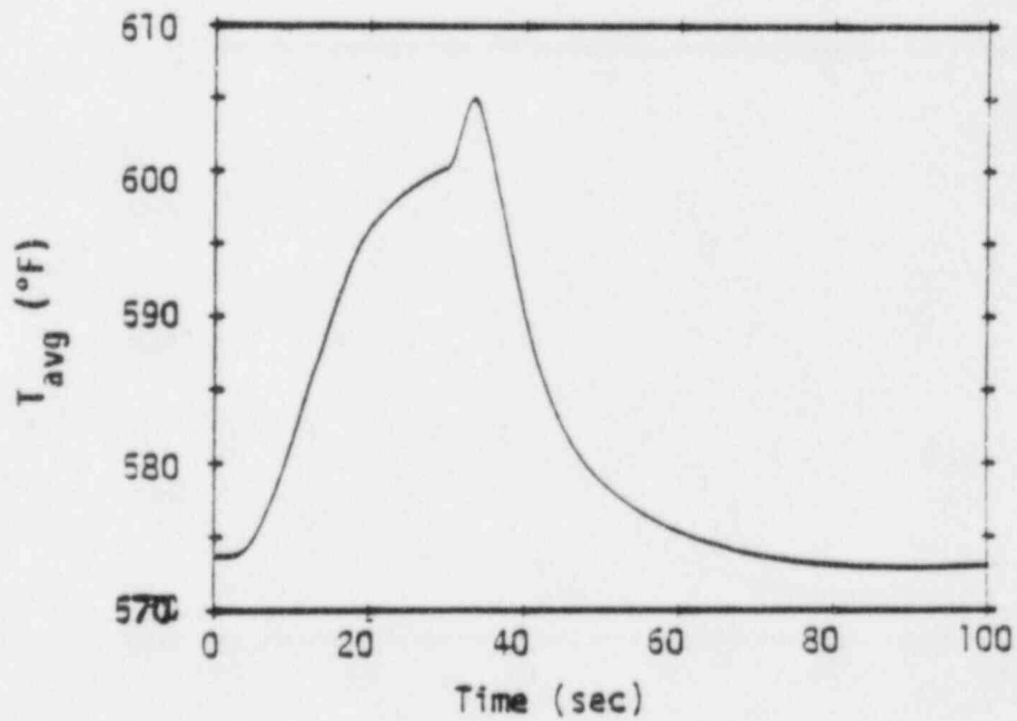
Figure 1 Turbine Trip with Pressure Control - Minimum Feedback - Nuclear Power and Reactor Coolant Average Temperature
