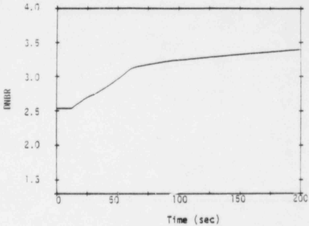
Figure 13 Turbine Trip With Pressure Control - Minimum Feedback - Steam Dump - Control Rod Insertion - No Loss of RCS Flow - DNBR
