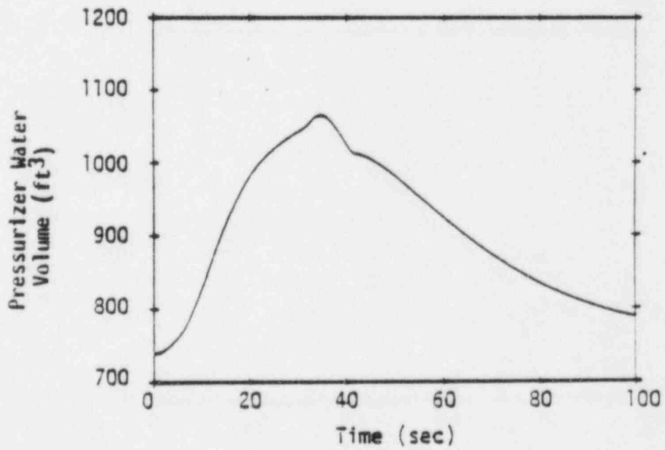
Figure 2 Turbine Trip with Pressure Control - Minimum Feedback - Pressurizer Pressure and Water Volume
