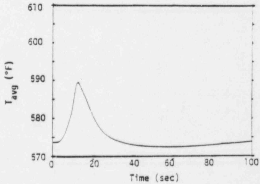
Figure 6 Turbine Trip Without Pressure Control - Minimum Feedback - Nuclear Power and Reactor Coolant Temperature
