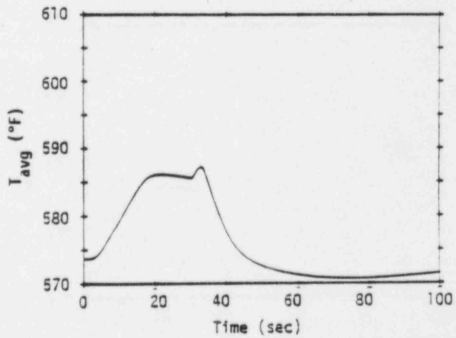
Figure 4 Turbine Trip with Pressure Control - Maximum Feedback - Nuclear Power and Reactor Coolant Average Temperature
