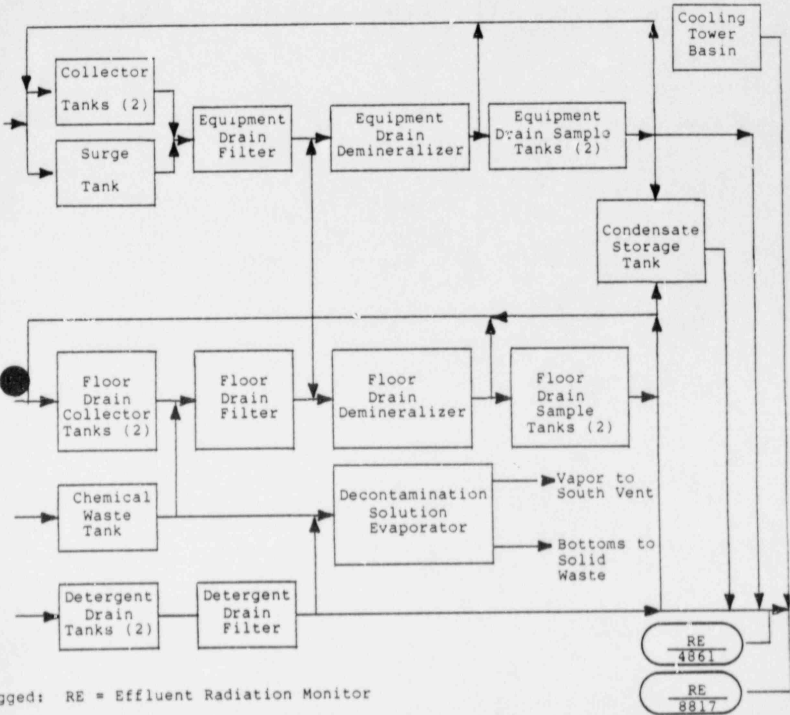
FIGURE 1-1 LIQUID RADWASTE TREATMENT SYSTEM
