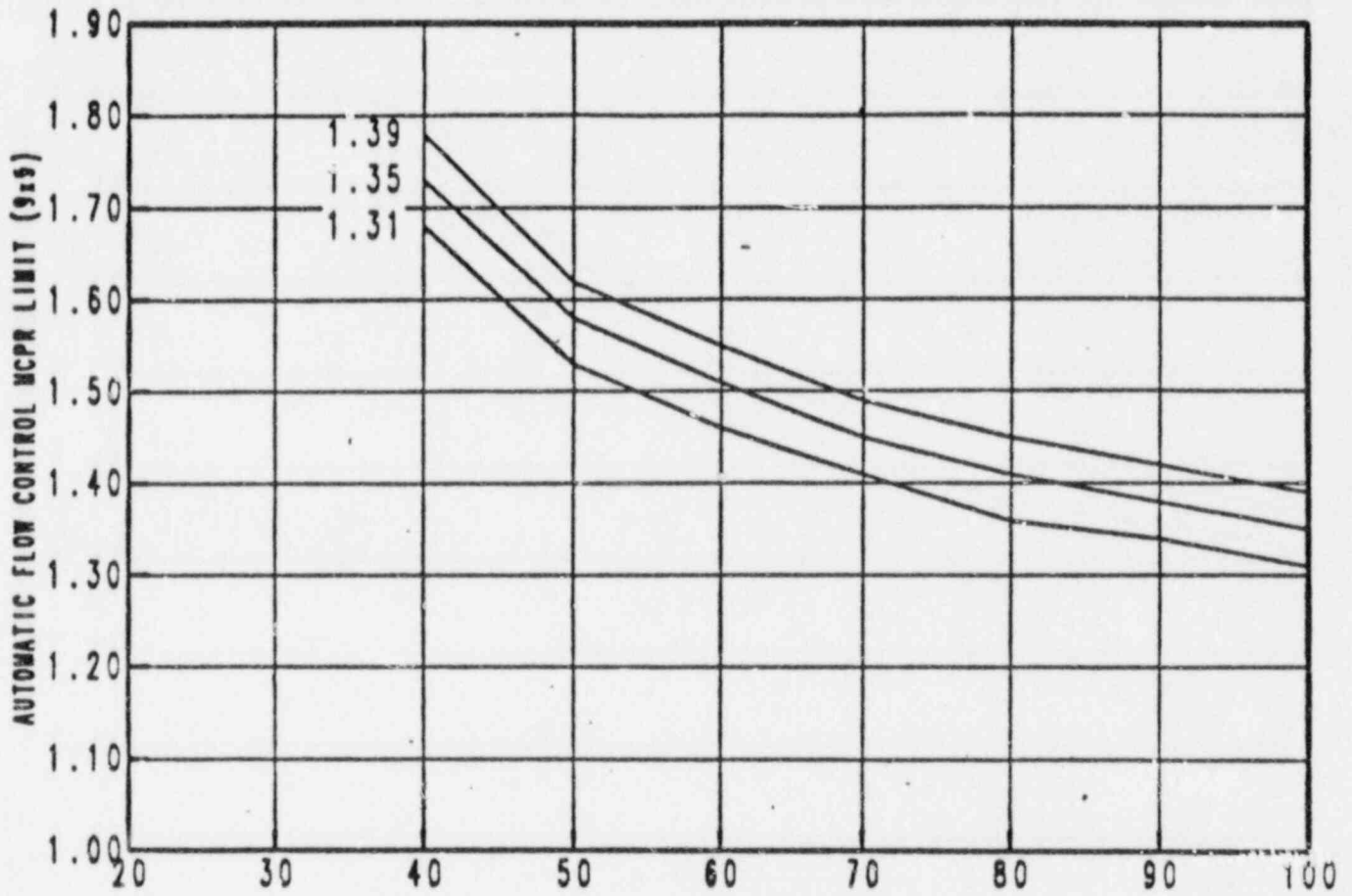
TOTAL CORE FLOW (% RATED, 98 MLB/HR)
