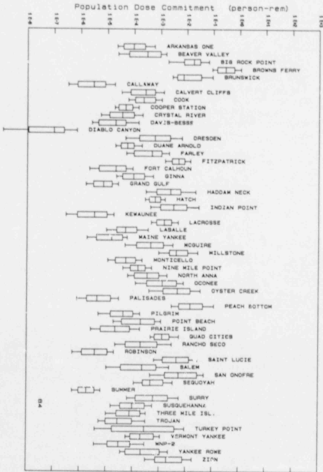
FIGURE 2. Airborne Population Dose Commitment for the Reactor Sites, 1984
