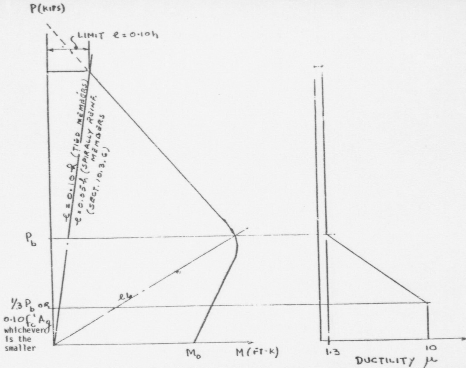
FIG 1. PROPOSED DUCTILITY RATIO FOR BEAM COLUMNS
