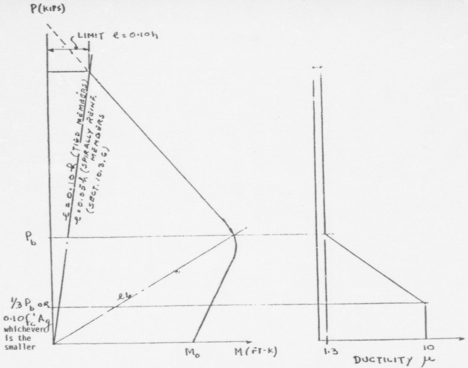
FIG 1. PROPOSED DUCTILITY RATIOS FOR BEAM COLUMNS
