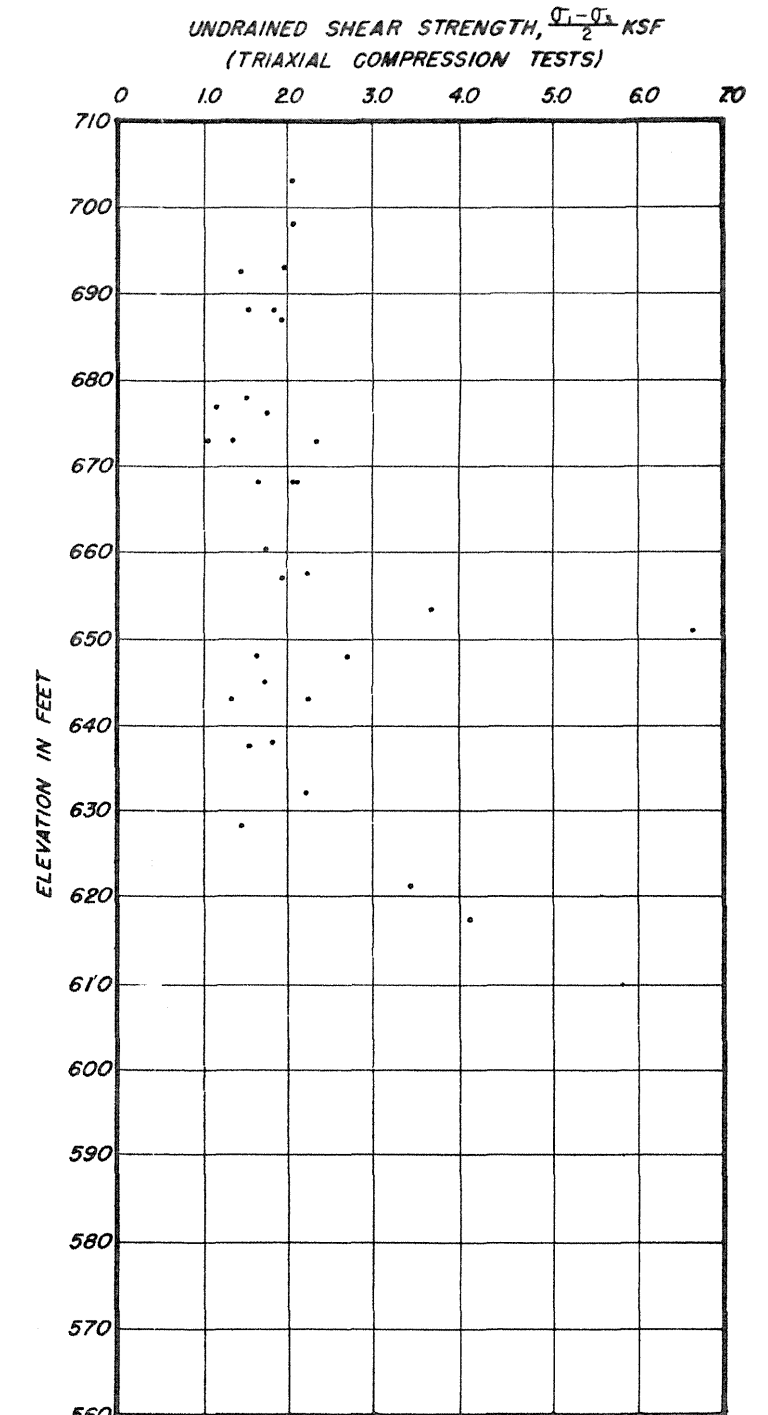
LA SALLE COUNTY STATION UPDATED FINAL SAFETY ANALYSIS REPORT FIGURE 2.5-79 UNDRAINED SHEAR STRENGTH VS. DEPTH
