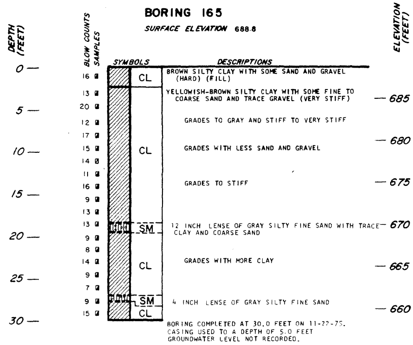
LA SALLE COUNTY STATION UPDATED FINAL SAFETY ANALYSIS REPORT FIGURE 2.5-19 LOGS OF BORINGS (SHEET 148)
