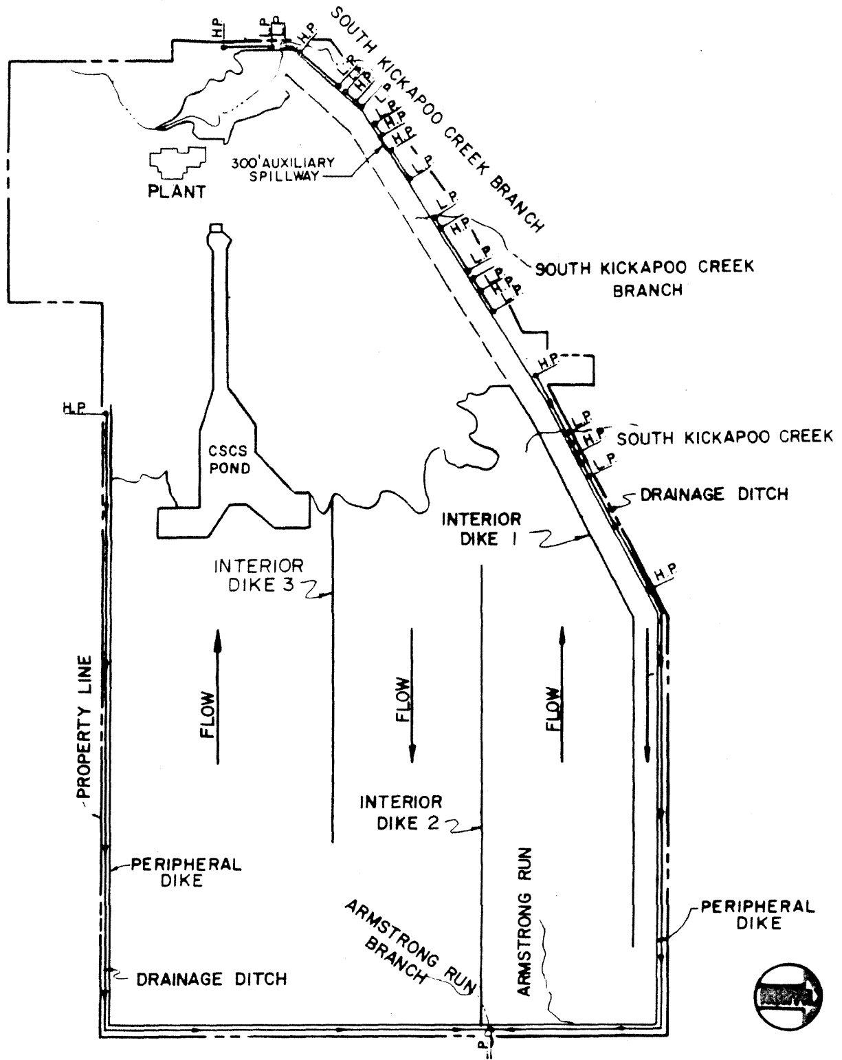
LA SALLE COUNTY STATION UPDATED FINAL SAFETY ANALYSIS REPORT FIGURE 2.5-76 PERIPHERAL DIKE DRAINAGE DITCHES
