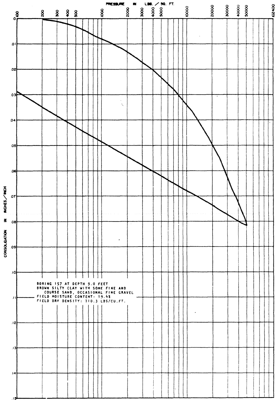
LA SALLE COUNTY STATION UPDATED FINAL SAFETY ANALYSIS REPORT FIGURE 2.5-45 CONSOLIDATION TEST DATA (SHEET 19)
