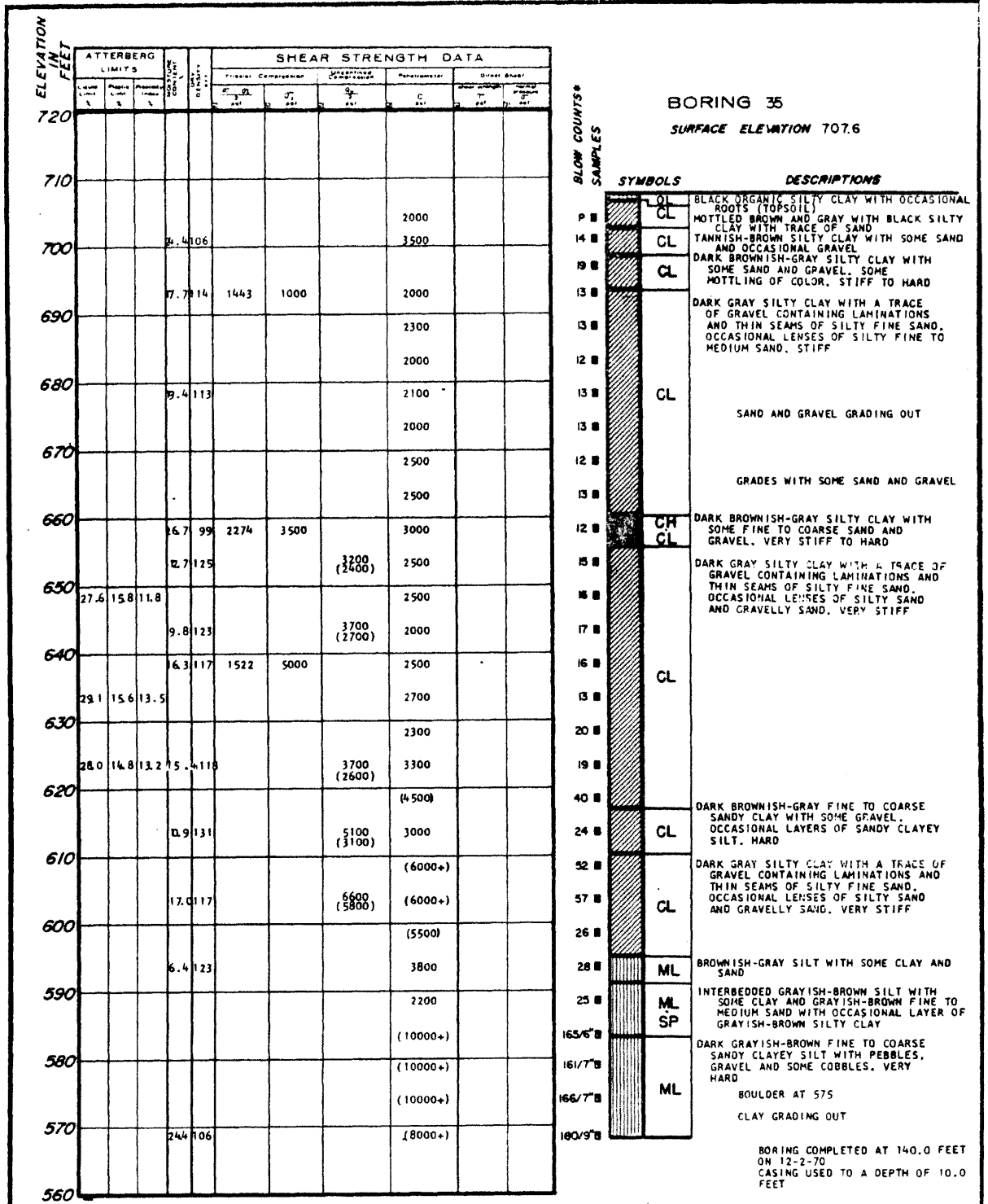
LA SALLE COUNTY STATION UPDATED FINAL SAFETY ANALYSIS REPORT FIGURE 2.5-19 LOGS OF BORINGS (SHEET 46)
