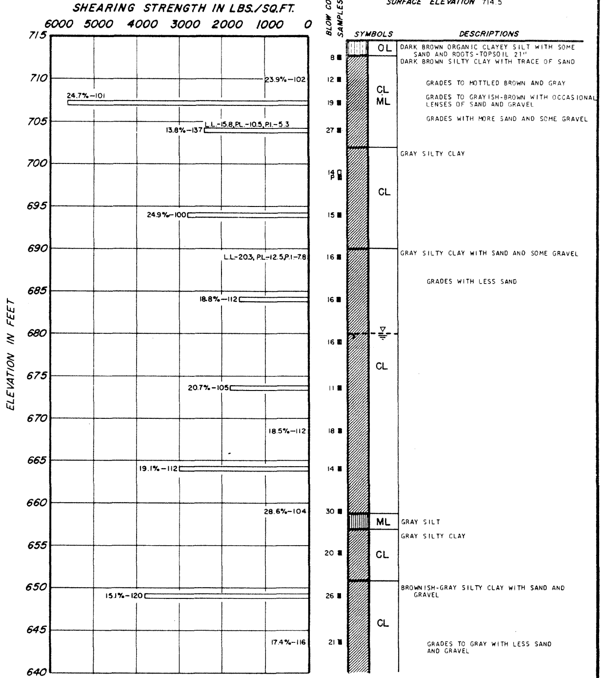
LA SALLE COUNTY STATION UPDATED FINAL SAFETY ANALYSIS REPORT FIGURE 2.5-19 LOGS OF BORINGS (SHEET 82)
