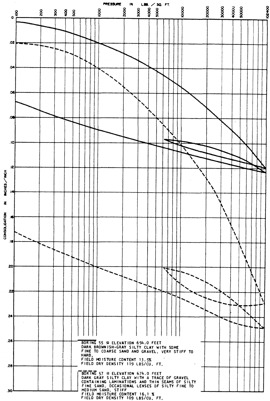
LA SALLE COUNTY STATION UPDATED FINAL SAFETY ANALYSIS REPORT FIGURE 2.5-45 CONSOLIDATION TEST DATA (SHEET 10)
