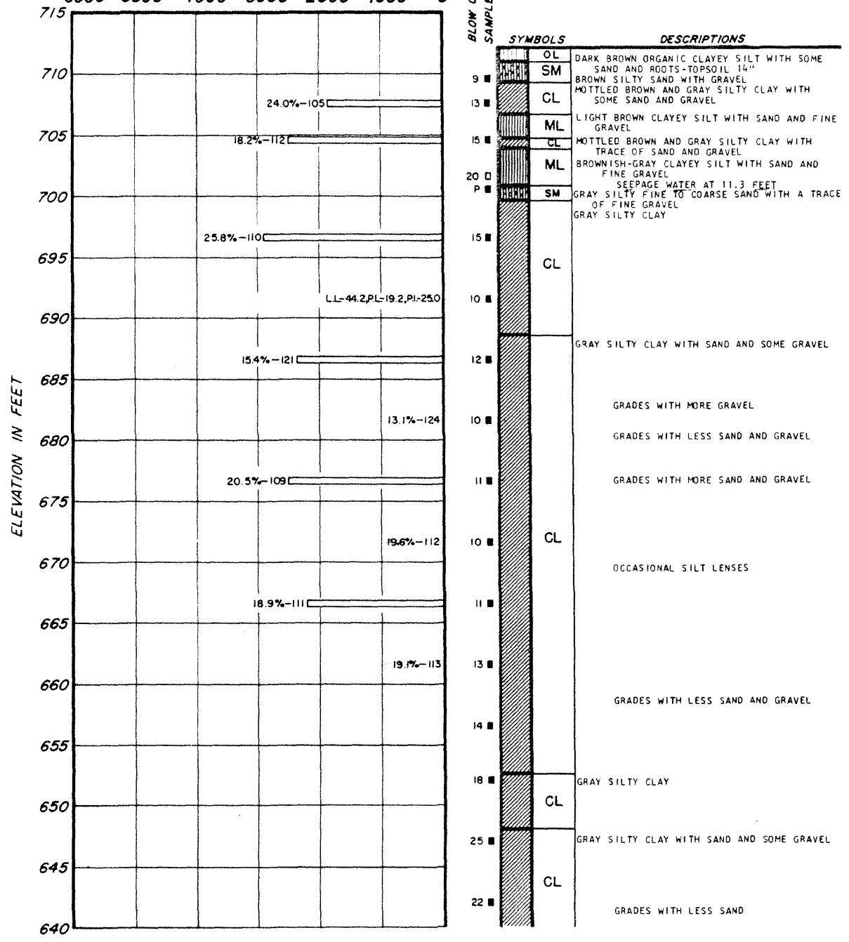
LA SALLE COUNTY STATION UPDATED FINAL SAFETY ANALYSIS REPORT FIGURE 2.5-19 LOGS OF BORINGS (SHEET 79)
