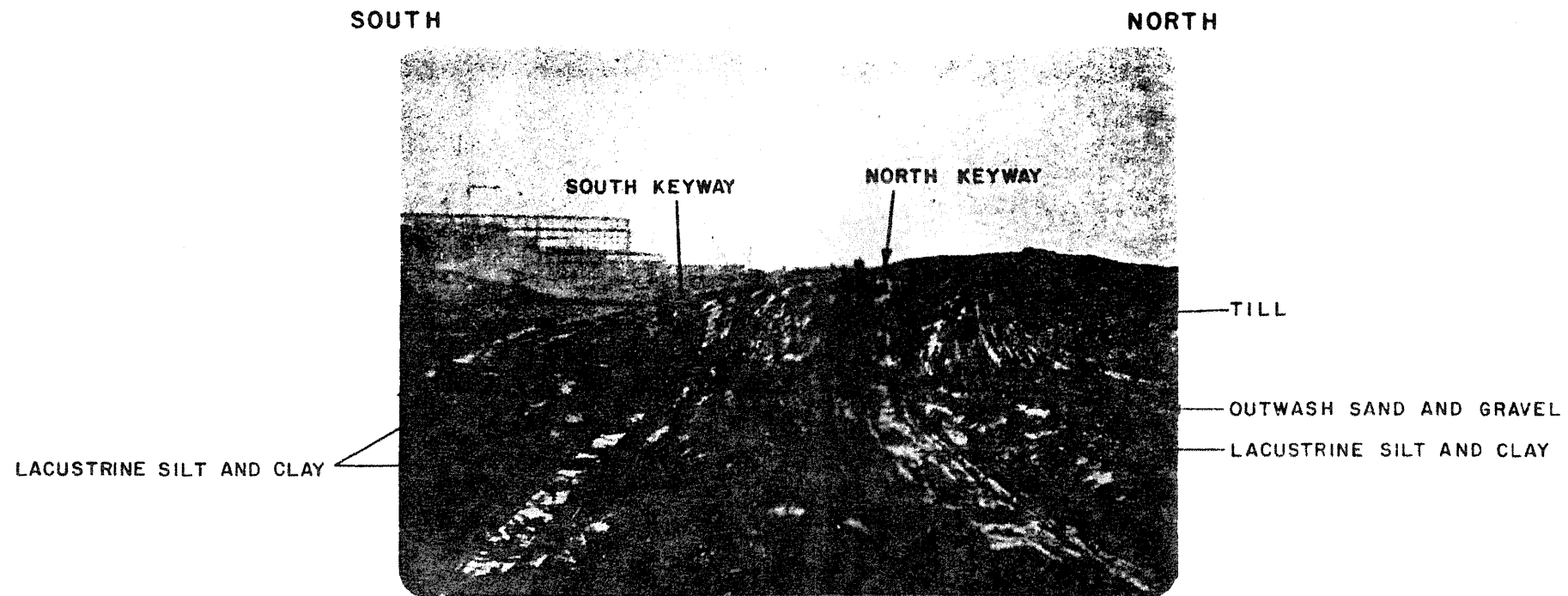
WEST WALL OF EXCAVATION (VIEW IS TO THE WEST FROM EAST WALL)
