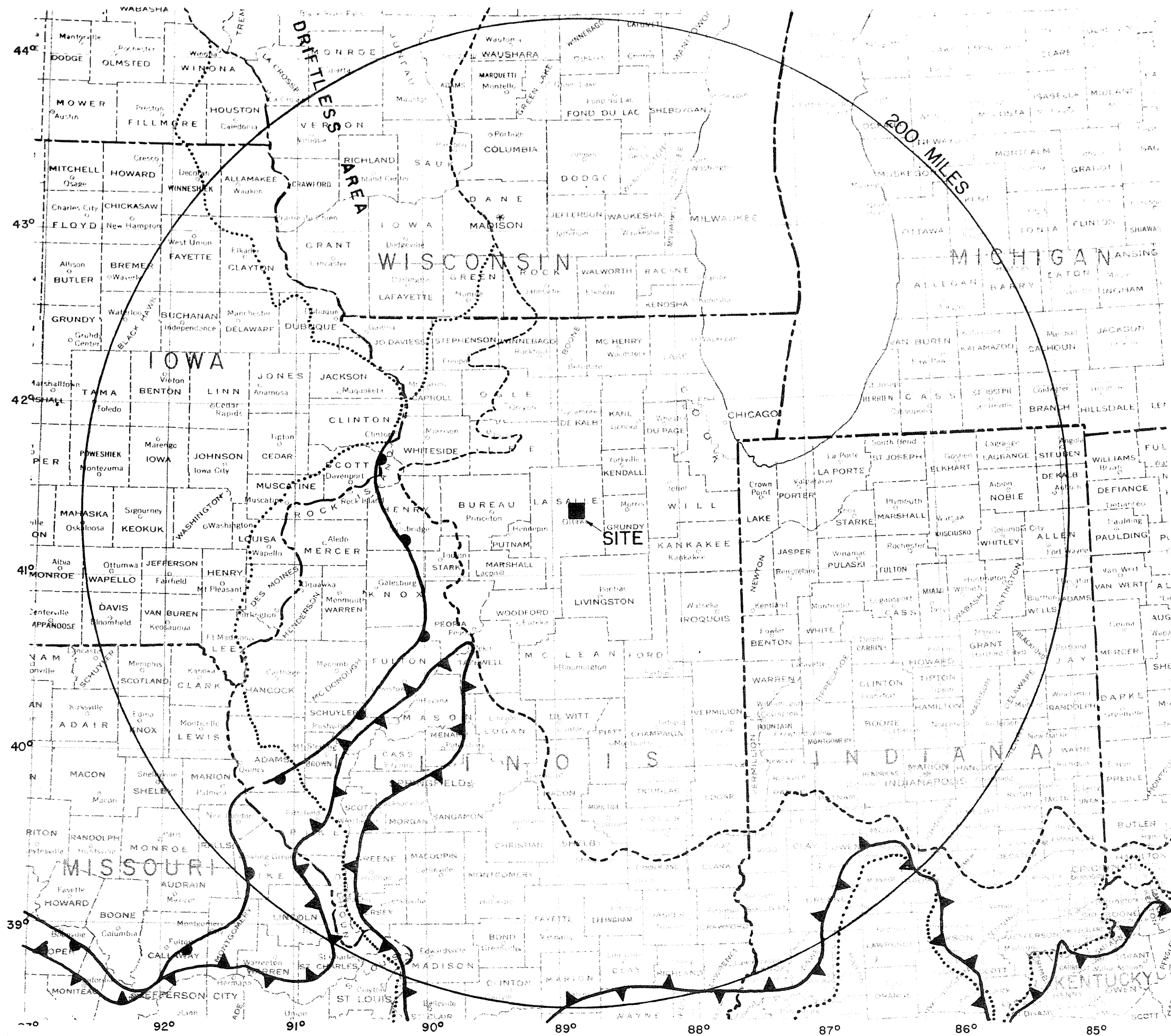
LA SALLE COUNTY STATION UPDATED FINAL SAFETY ANALYSIS REPORT FIGURE 2.5-32 LIMITS OF PLEISTOCENE GLACIATION
