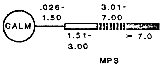
LA SALLE COUNTY STATION UPDATED FINAL SAFETY ANALYSIS REPORT FIGURE 2.3-12 JULY 1977 AND JULY 1978 WIND ROSE 375-FOOT LEVEL
