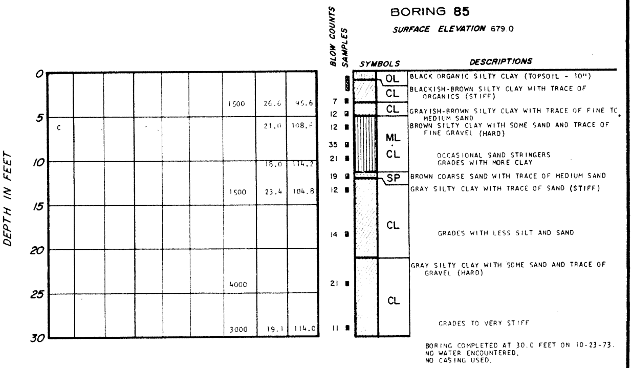
LA SALLE COUNTY STATION UPDATED FINAL SAFETY ANALYSIS REPORT FIGURE 2.5-19 LOGS OF BORINGS (SHEET 105)
