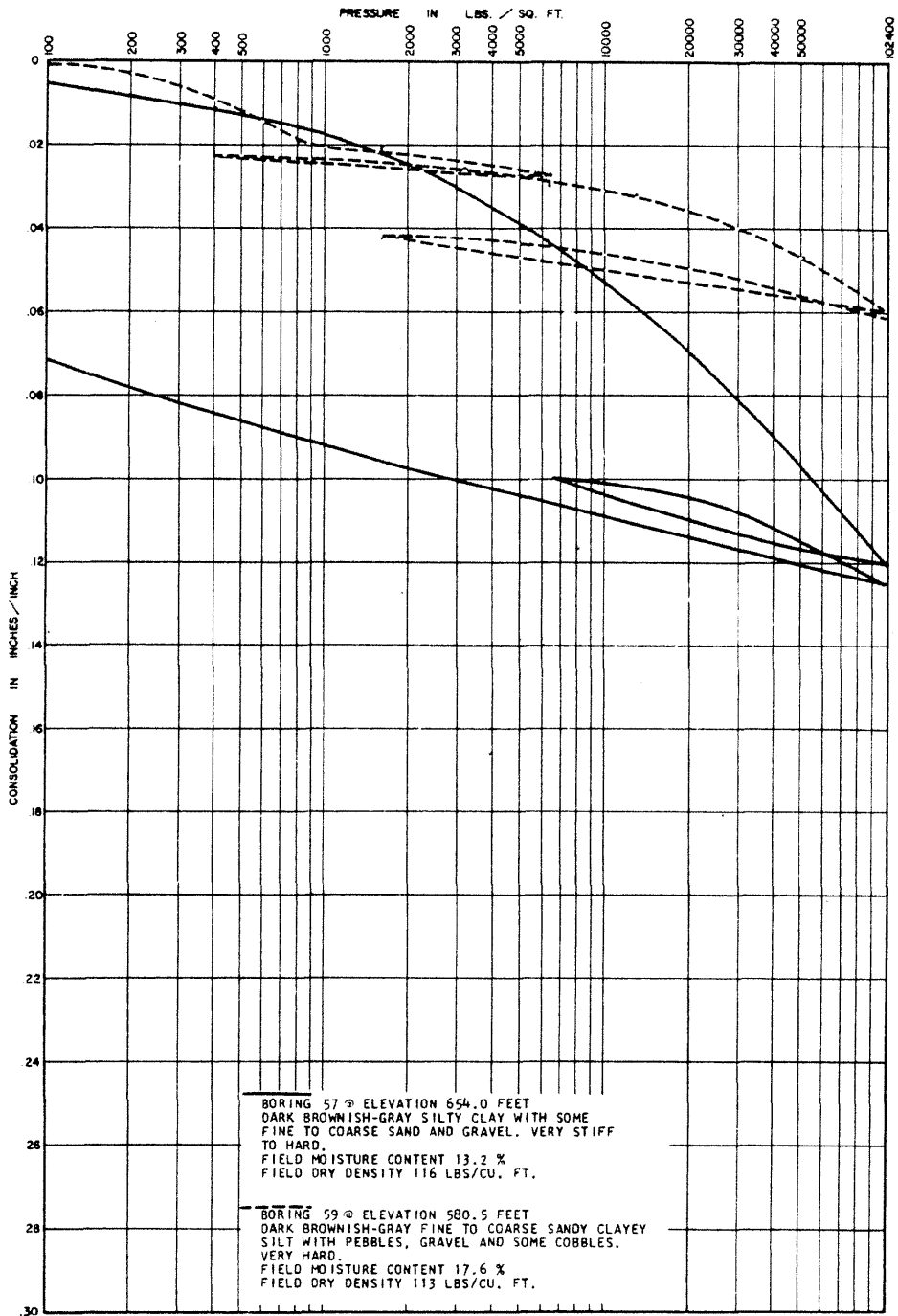
LA SALLE COUNTY STATION UPDATED FINAL SAFETY ANALYSIS REPORT FIGURE 2.5-45 CONSOLIDATION TEST DATA (SHEET 11)
