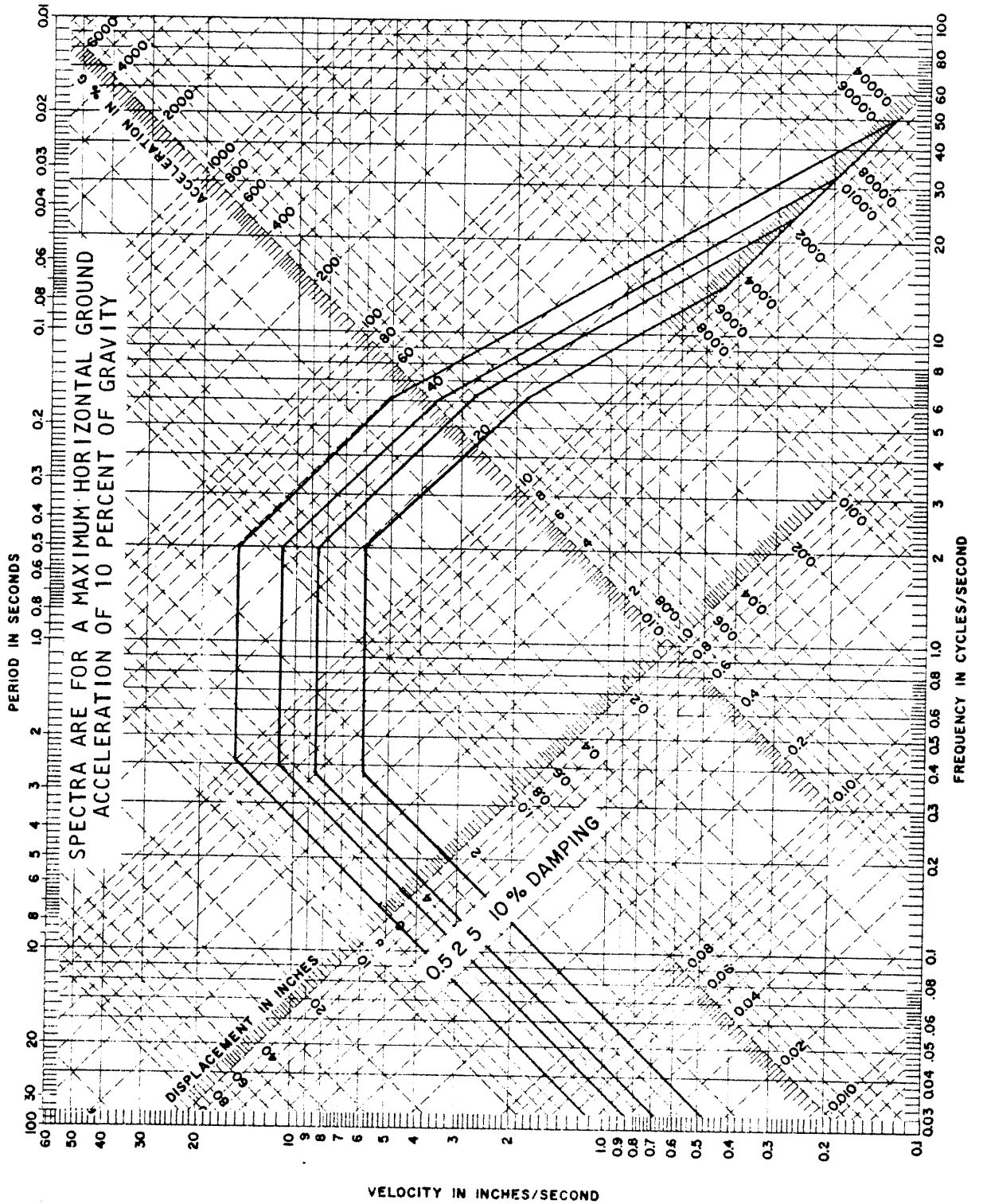
LA SALLE COUNTY STATION UPDATED FINAL SAFETY ANALYSIS REPORT FIGURE 2.5-40 RESPONSE SPECTRA - OPERATING BASIS EARTHQUAKE
