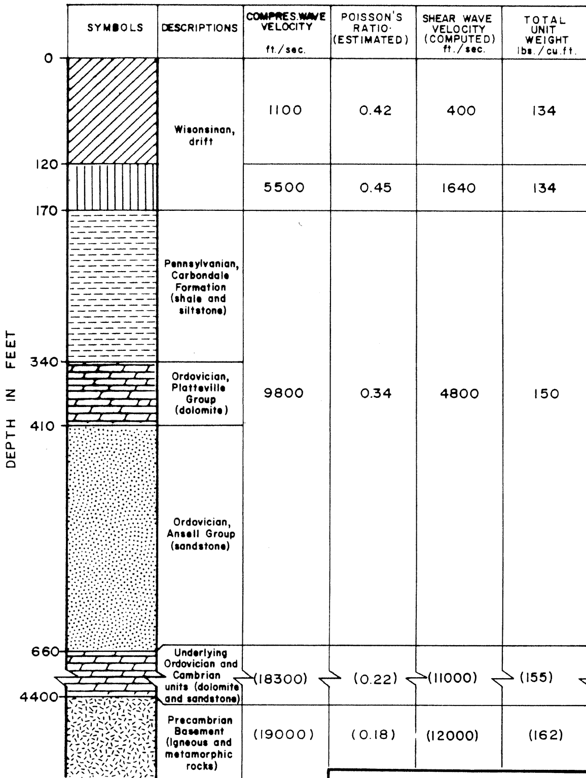
LA SALLE COUNTY STATION UPDATED FINAL SAFETY ANALYSIS REPORT. FIGURE 2.5-49 STRATIGRAPHIC COLUMN WITH GEOPHYSICAL DATA SUMMARY
