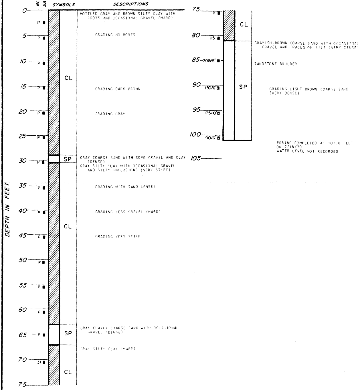
LA SALLE COUNTY STATION UPDATED FINAL SAFETY ANALYSIS REPORT FIGURE 2.5-19 LOGS OF BORINGS (SHEET 156)
