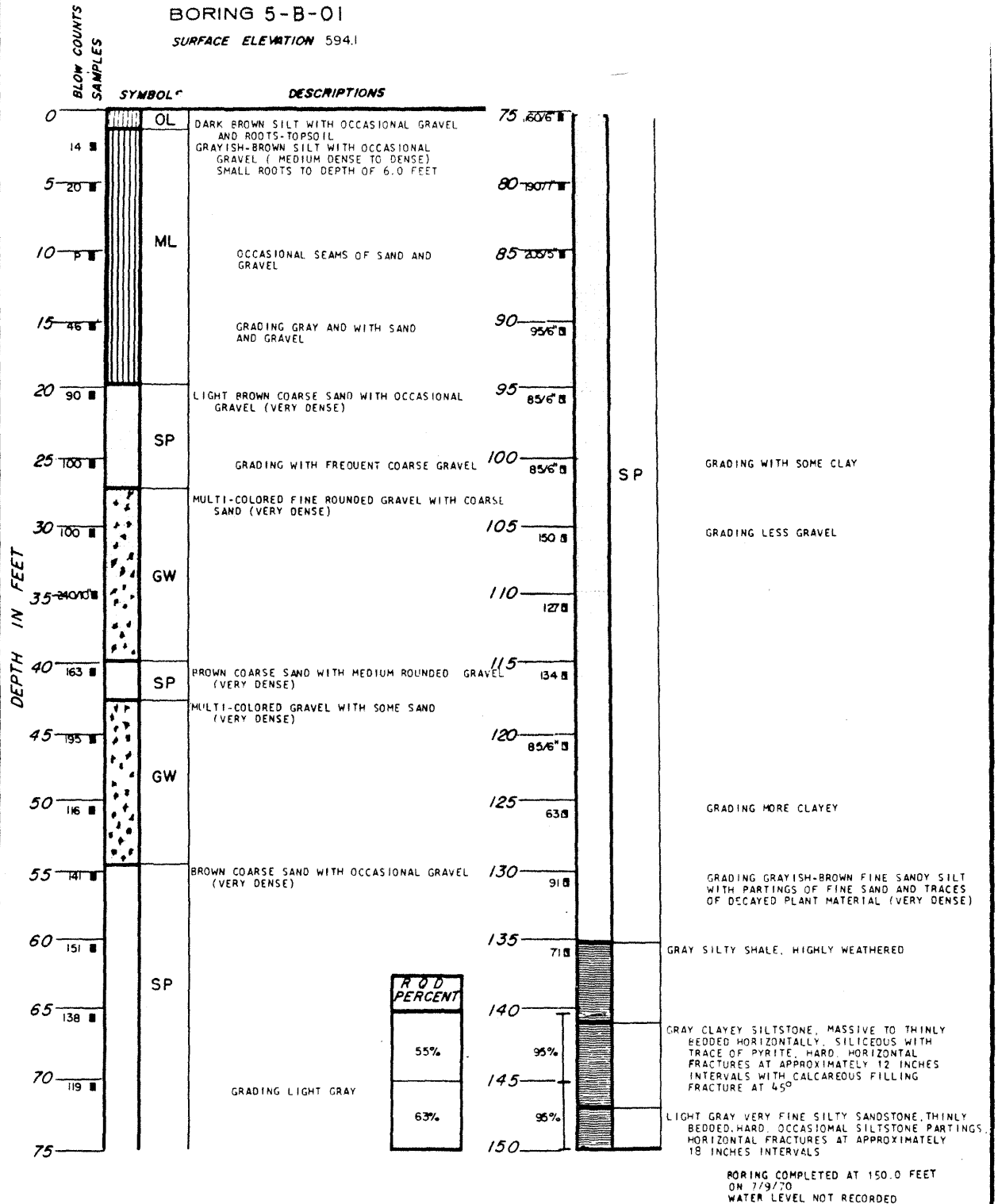
LA SALLE COUNTY STATION UPDATED FINAL SAFETY ANALYSIS REPORT FIGURE 2.5-19 LOGS OF BORINGS (SHEET 155)
