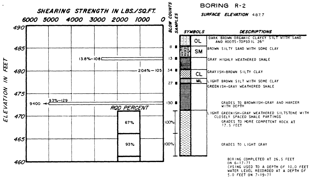
LA SALLE COUNTY STATION UPDATED FINAL SAFETY ANALYSIS REPORT FIGURE 2.5-19 LOGS OF BORINGS (SHEET 201)
