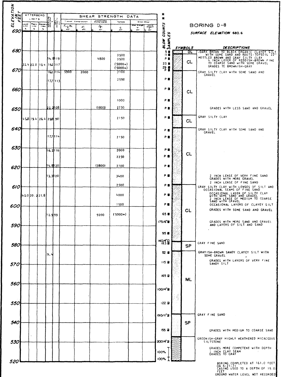
LA SALLE COUNTY STATION UPDATED FINAL SAFETY ANALYSIS REPORT FIGURE 2.5-19 LOGS OF BORINGS (SHEET 191)
