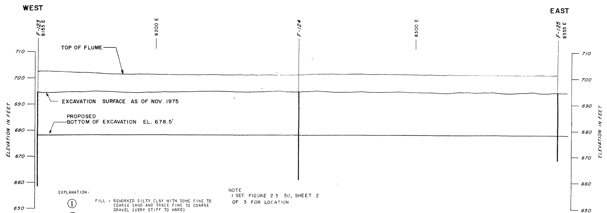
LA SALLE COUNTY STATION UPDATED FINAL SAFETY ANALYSIS REPORT FIGURE 2.5-81 GEOLOGIC MAP OF NORTH FLUME WALL (SHEET 6 of 9)
