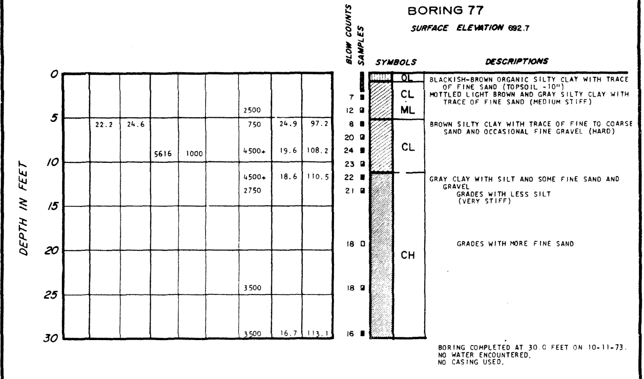
LA SALLE COUNTY STATION UPDATED FINAL SAFETY ANALYSIS REPORT FIGURE 2.5-19 LOGS OF BORINGS (SHEET 101) REV. 0 - APRIL 1984
