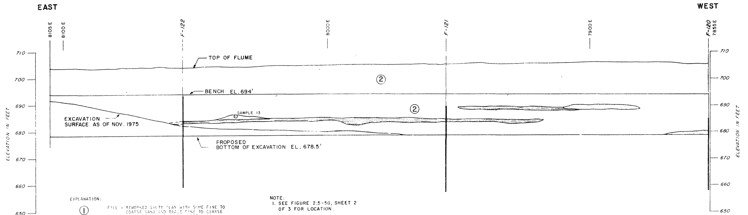
LA SALLE COUNTY STATION UPDATED FINAL SAFETY ANALYSIS REPORT FIGURE 2.5-82 GEOLOGIC MAP OF SOUTH FLUME WALL (SHEET 4 of 9)
