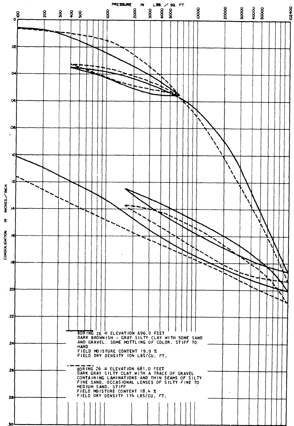
LA SALLE COUNTY STATION UPDATED FINAL SAFETY ANALYSIS REPORT FIGURE 2.5-45 CONSOLIDATION TEST DATA (SHEET 4)
