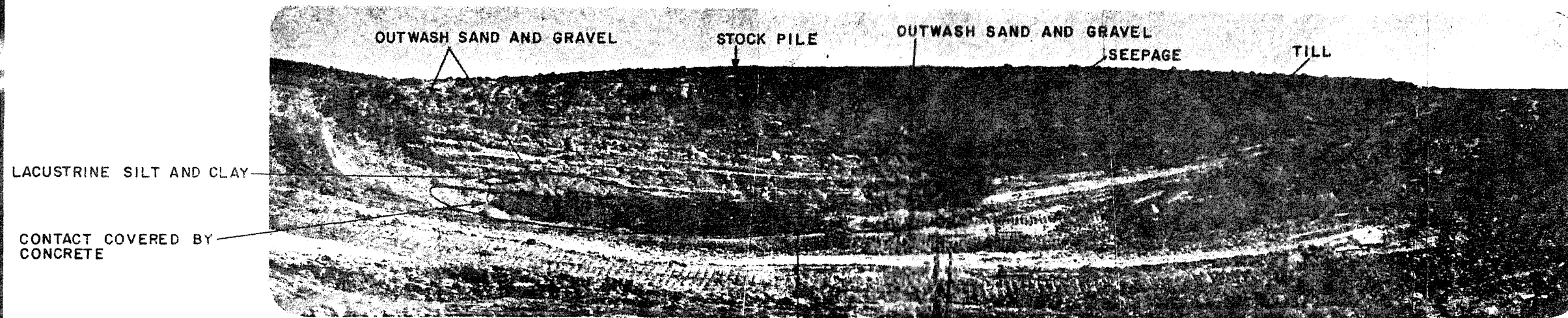
SOUTH WALL OF EXCAVATION (VIEW IS TO THE SOUTH FROM CENTER OF EXCAVATION)
