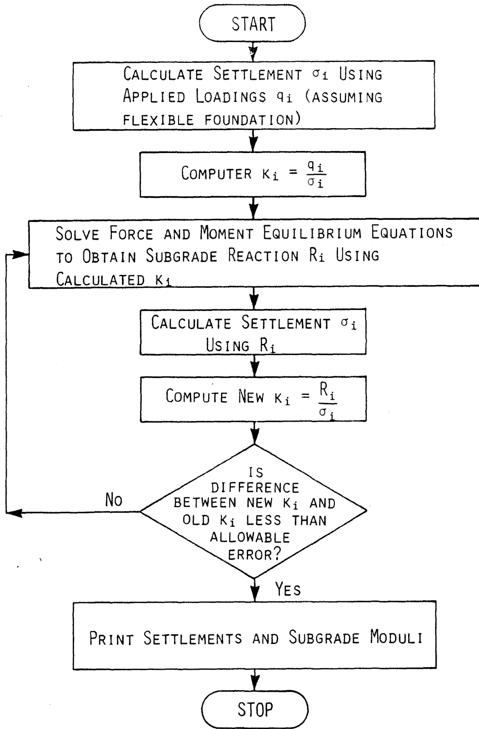
LA SALLE COUNTY STATION UPDATED FINAL SAFETY ANALYSIS REPORT FIGURE 2.5-91 FLOWCHART FOR THE SETTLEMENT CALCULATION FOR RIGID FOUNDATION
