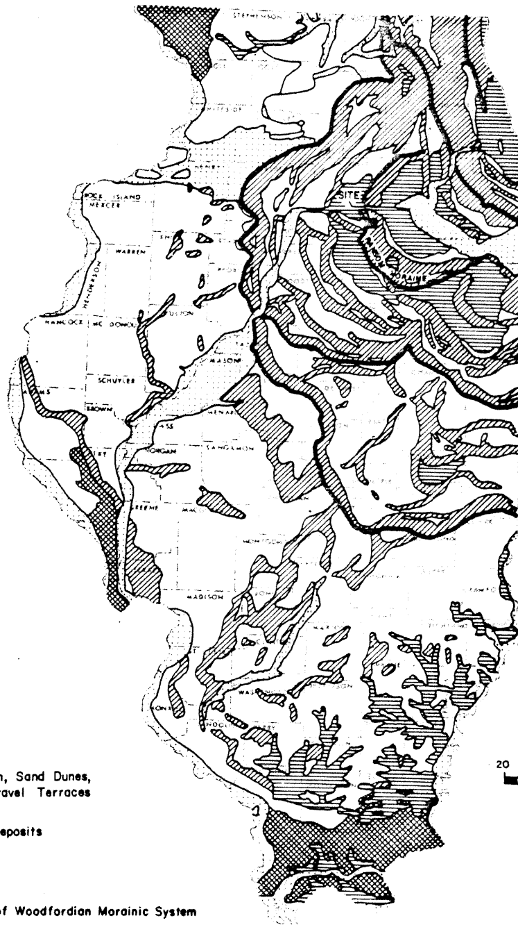
LA SALLE COUNTY STATION UPDATED FINAL SAFETY ANALYSIS REPORT FIGURE 2.5-22 GLACIAL MAP OF ILLINOIS
