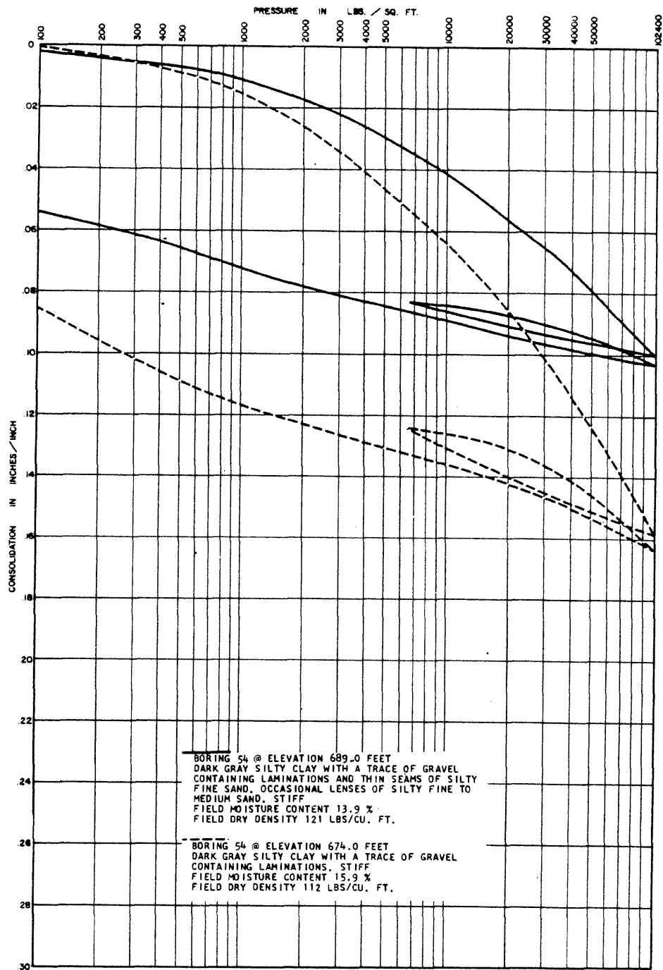
LA SALLE COUNTY STATION UPDATED FINAL SAFETY ANALYSIS REPORT FIGURE 2.5-45 CONSOLIDATION TEST DATA (SHEET 9)
