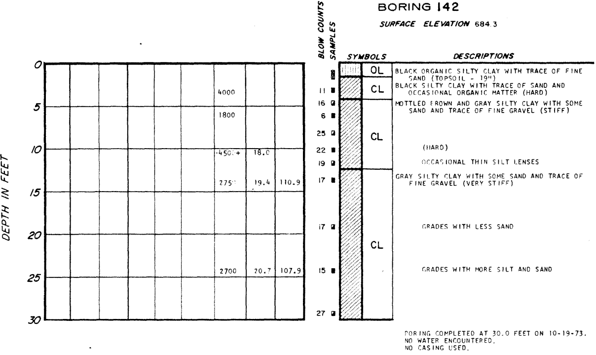
LA SALLE COUNTY STATION UPDATED FINAL SAFETY ANALYSIS REPORT FIGURE 2.5-19 LOGS OF BORINGS (SHEET 136)
