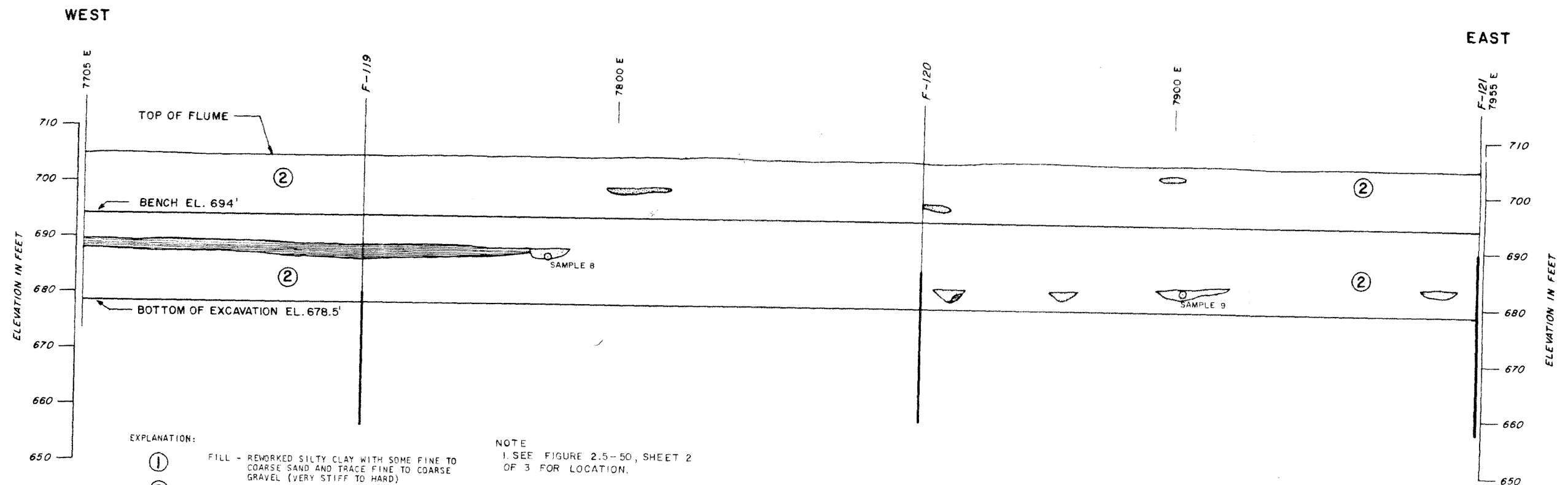
LA SALLE COUNTY STATION UPDATED FINAL SAFETY ANALYSIS REPORT FIGURE 2.5-81 GEOLOGIC MAP OF NORTH FLUME WALL (SHEET 5 of 9)
