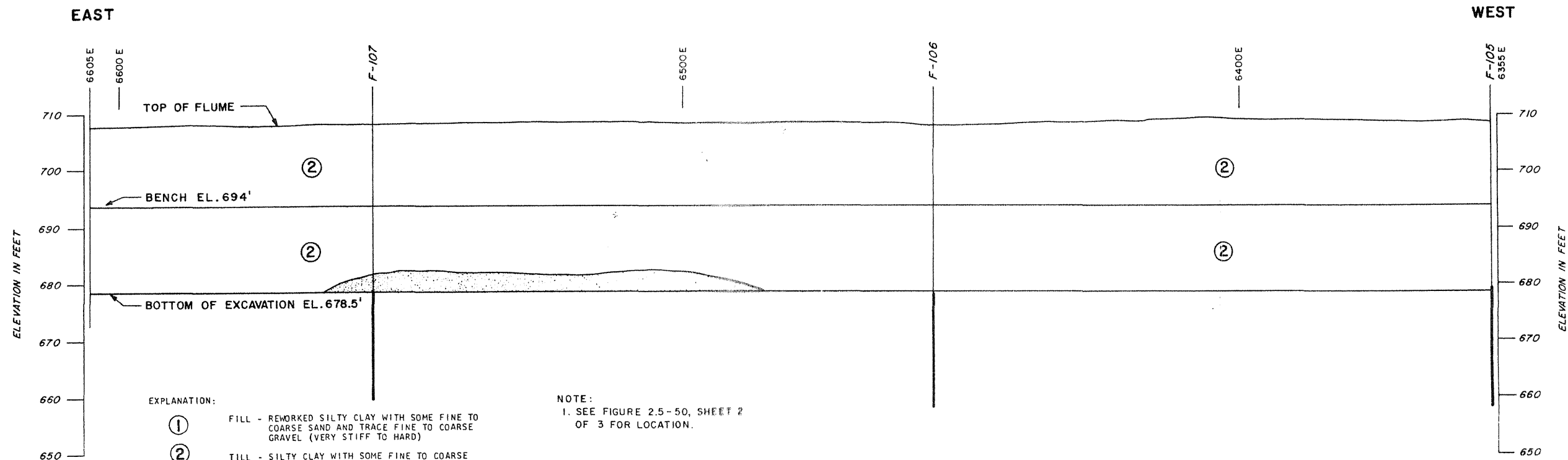
LA SALLE COUNTY STATION UPDATED FINAL SAFETY ANALYSIS REPORT FIGURE 2.5-82 GEOLOGIC MAP OF SOUTH FLUME WALL (SHEET 7 of 9)
