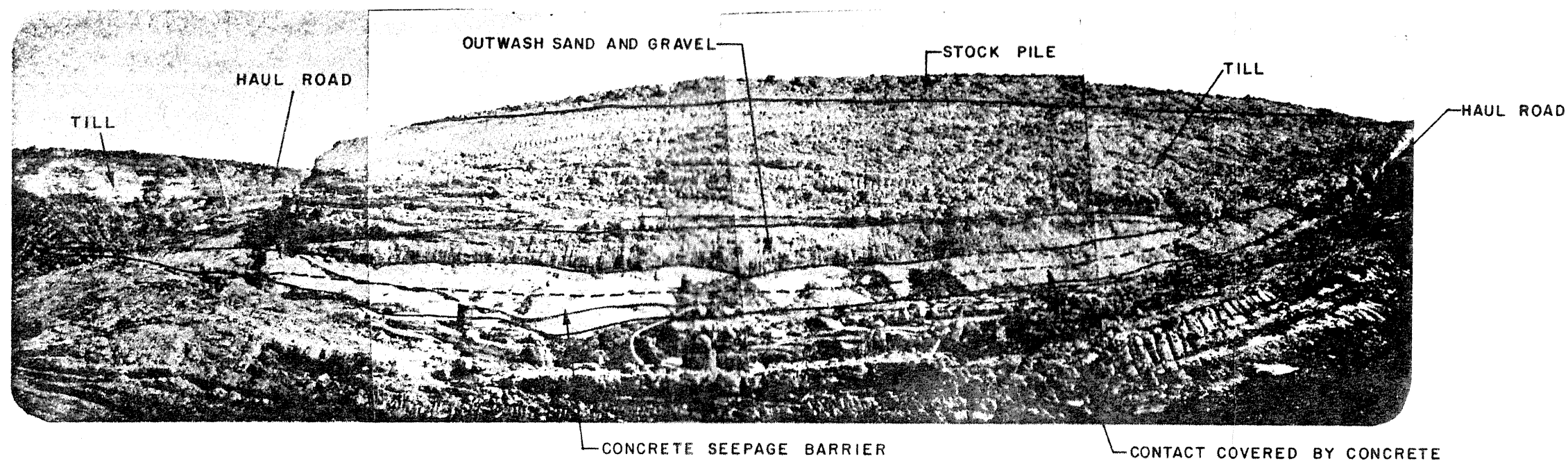
NORTH WALL OF EXCAVATION (VIEW IS TO THE NORTH FROM CENTER OF EXCAVATION)
