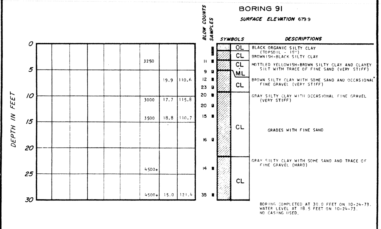
LA SALLE COUNTY STATION UPDATED FINAL SAFETY ANALYSIS REPORT FIGURE 2.5-19 LOGS OF BORINGS (SHEET 108)
