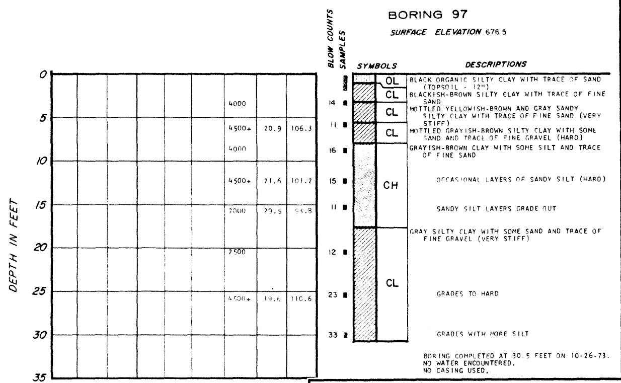
LA SALLE COUNTY STATION UPDATED FINAL SAFETY ANALYSIS REPORT FIGURE 2.5-19 LOGS OF BORINGS (SHEET 111)
