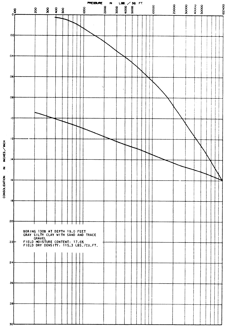
LA SALLE COUNTY STATION UPDATED FINAL SAFETY ANALYSIS REPORT FIGURE 2.5-45 CONSOLIDATION TEST DATA (SHEET 18)
