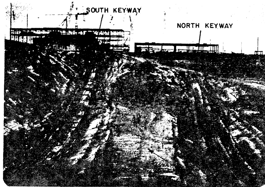
WEST WALL OF EXCAVATION (VIEW IS TO THE WEST FROM EAST WALL)
