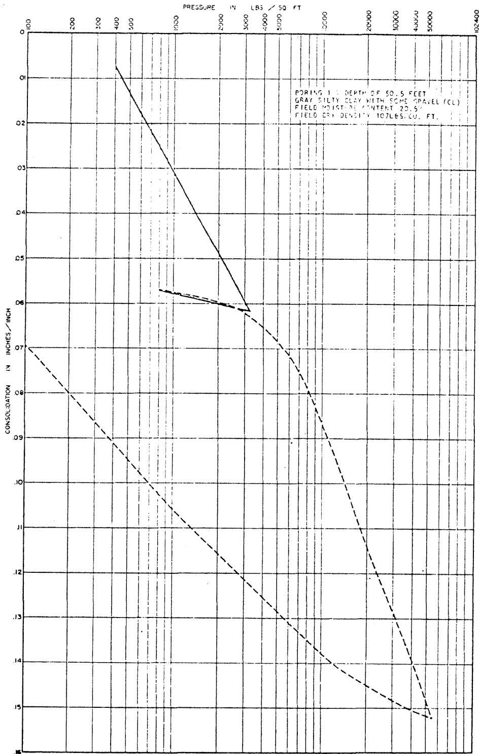
LA SALLE COUNTY STATION UPDATED FINAL SAFETY ANALYSIS REPORT FIGURE 2.5-45 CONSOLIDATION TEST DATA (SHEET 1)
