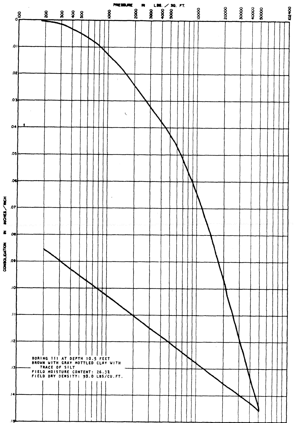
LA SALLE COUNTY STATION UPDATED FINAL SAFETY ANALYSIS REPORT FIGURE 2.5-45 CONSOLIDATION TEST DATA (SHEET 17)
