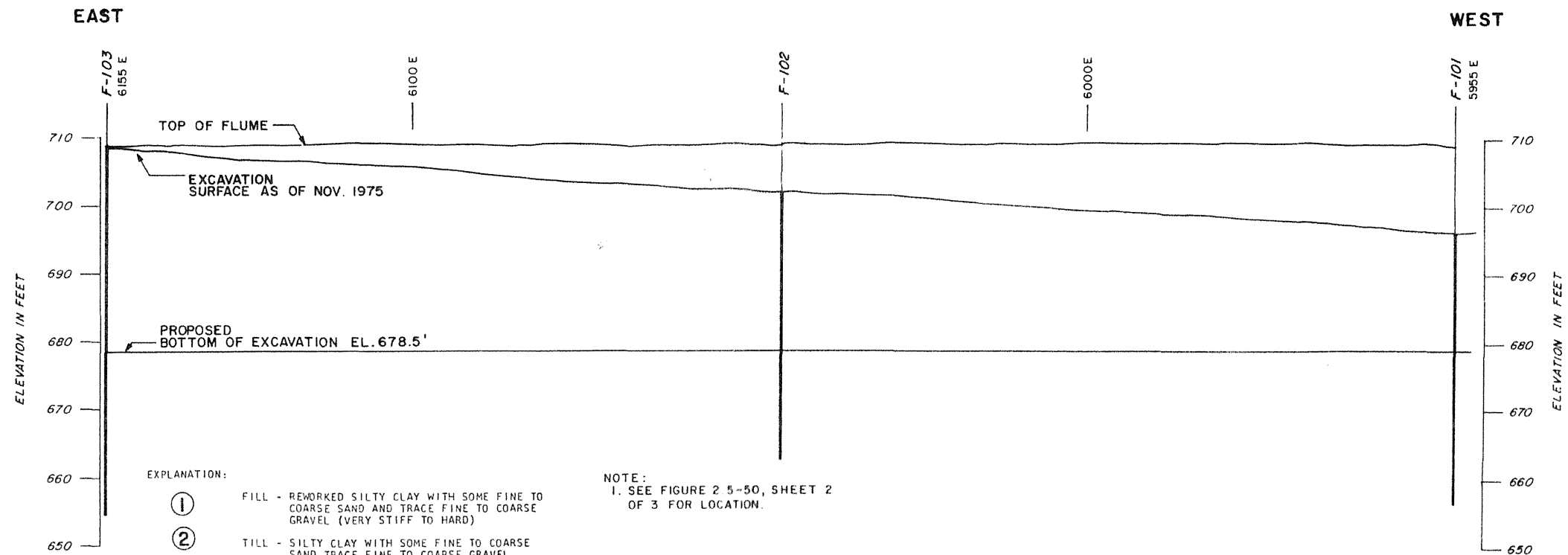
LA SALLE COUNTY STATION UPDATED FINAL SAFETY ANALYSIS REPORT FIGURE 2.5-82 GEOLOGIC MAP OF SOUTH FLUME WALL (SHEET 8 of 9)
