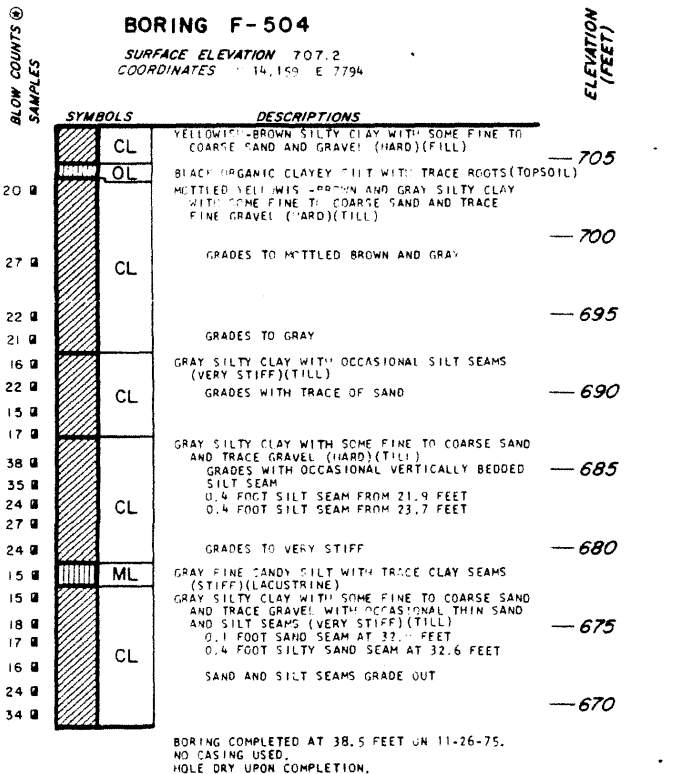
LA SALLE COUNTY STATION UPDATED FINAL SAFETY ANALYSIS REPORT FIGURE 2.5-19 LOGS OF BORINGS (SHEET 249)
