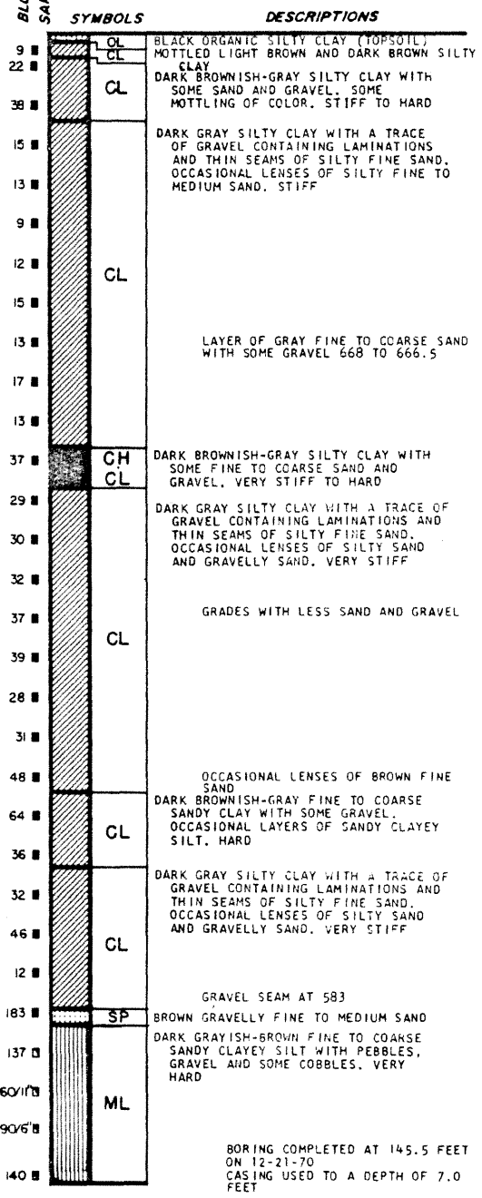
LA SALLE COUNTY STATION UPDATED FINAL SAFETY ANALYSIS REPORT FIGURE 2.5-19 LOGS OF BORINGS (SHEET 64)
