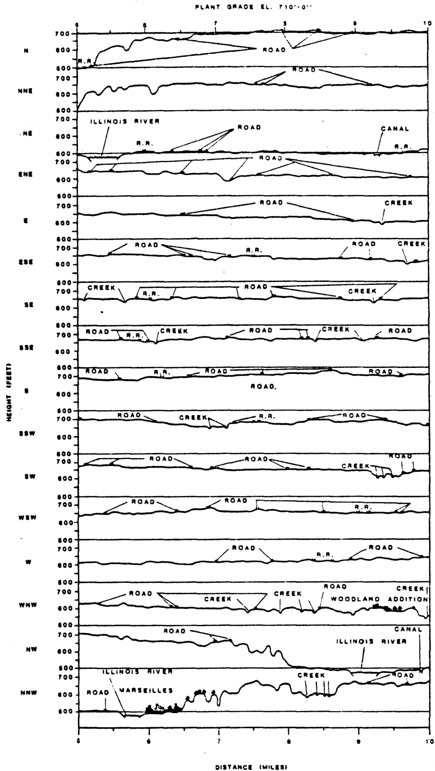
LA SALLE COUNTY STATION UPDATED FINAL SAFETY ANALYSIS REPORT FIGURE 2.3-16 TOPOGRAPHIC PROFILES OF THE AREA 5 TO 10 MILES FROM THE LA SALLE COUNTY STATION
