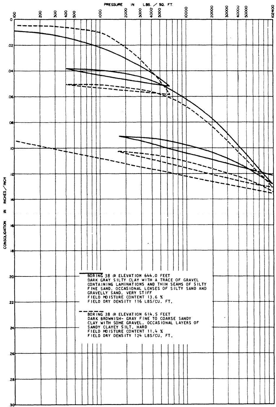
LA SALLE COUNTY STATION UPDATED FINAL SAFETY ANALYSIS REPORT FIGURE 2.5-45 CONSOLIDATION TEST DATA (SHEET 7)
