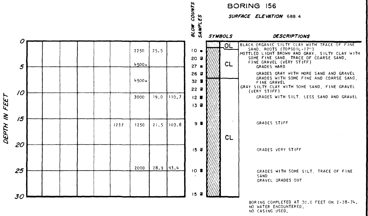
LA SALLE COUNTY STATION UPDATED FINAL SAFETY ANALYSIS REPORT FIGURE 2.5-19 LOGS OF BORINGS (SHEET 143)
