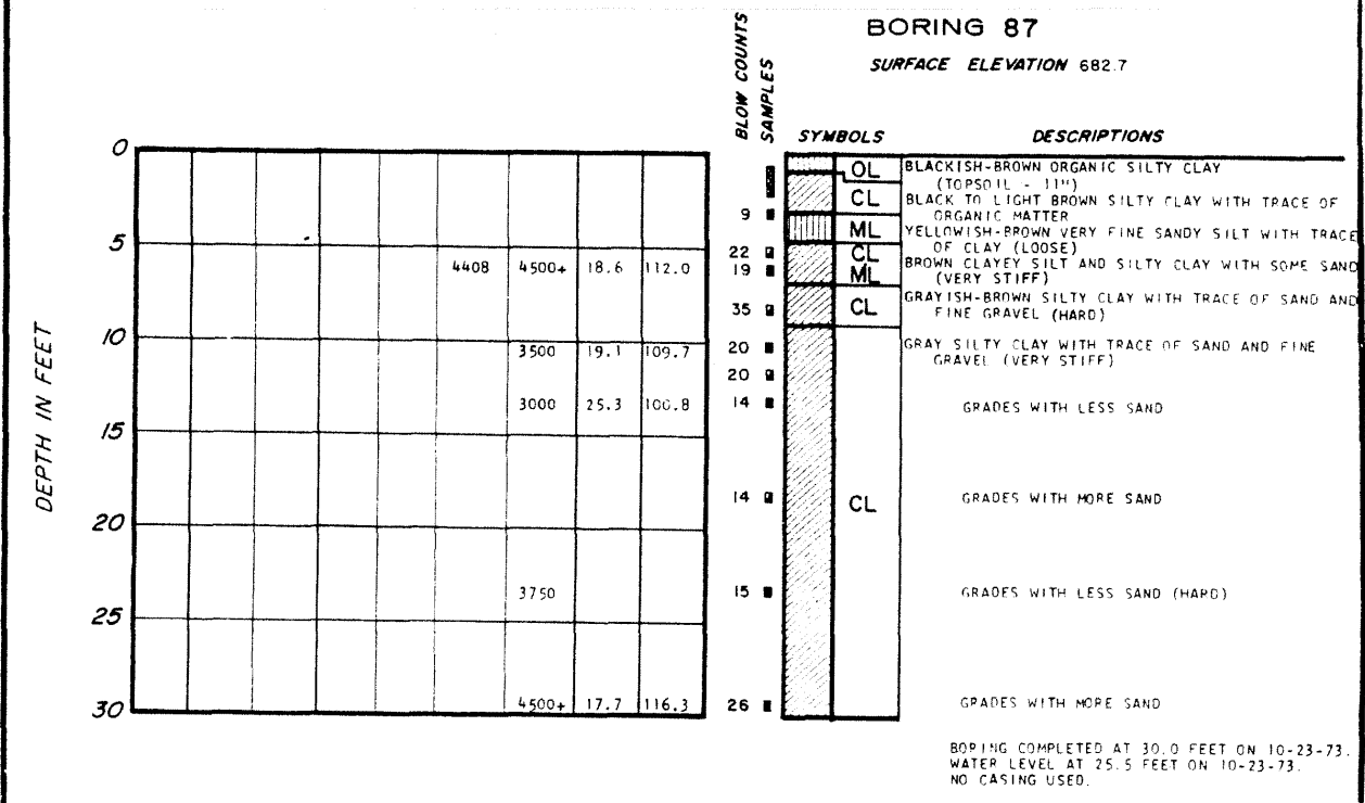
LA SALLE COUNTY STATION UPDATED FINAL SAFETY ANALYSIS REPORT FIGURE 2.5-19 LOGS OF BORINGS (SHEET 106) REV. 0 - APRIL 1984
