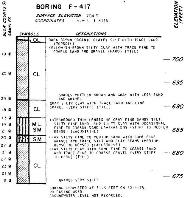
LA SALLE COUNTY STATION UPDATED FINAL SAFETY ANALYSIS REPORT FIGURE 2.5-19 LOGS OF BORINGS (SHEET 247)
