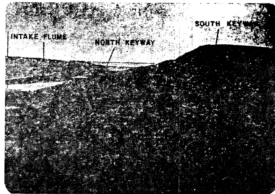
EAST WALL OF EXCAVATION (VIEW IS TO THE EAST FROM WEST WALL)
