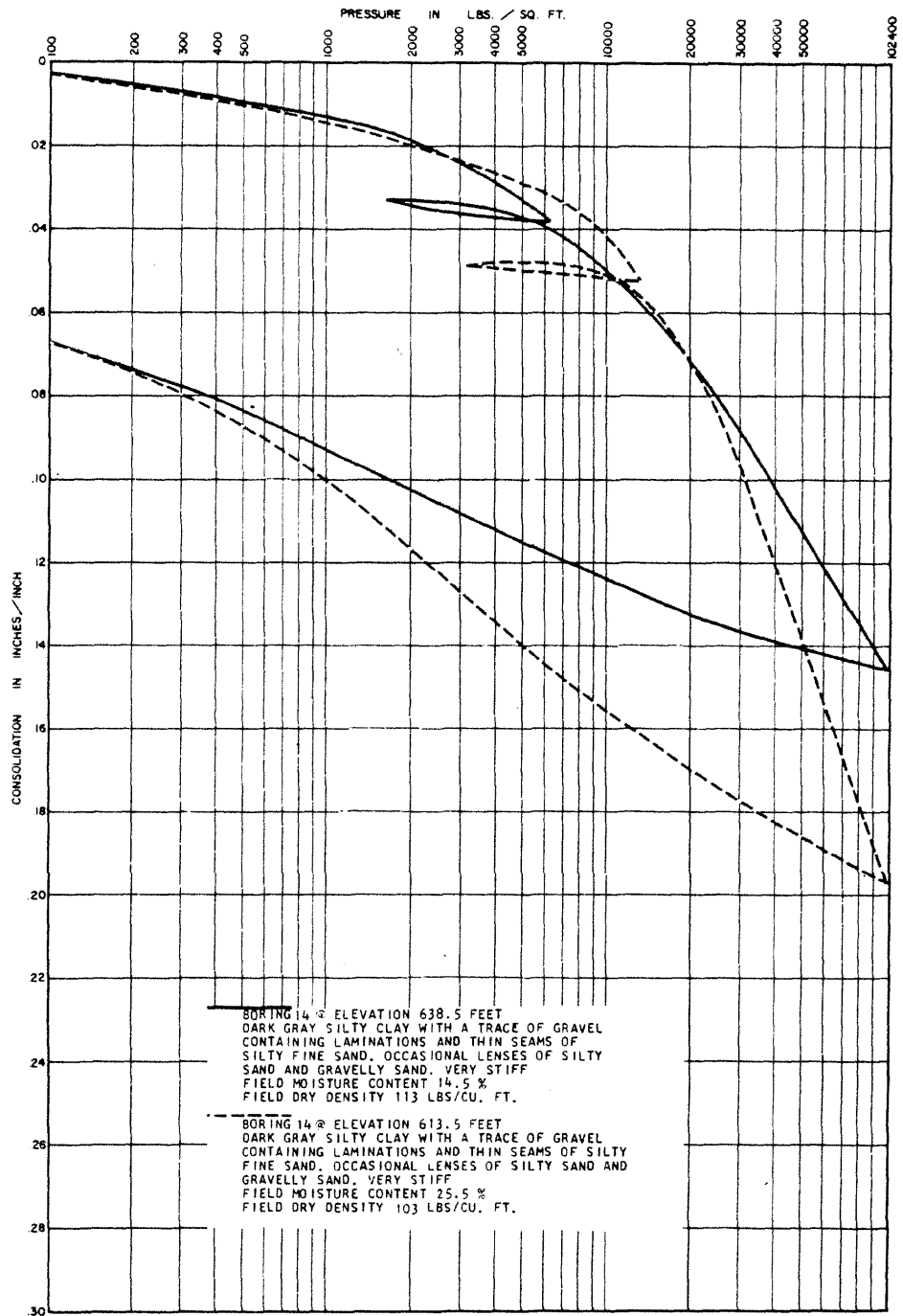
LA SALLE COUNTY STATION UPDATED FINAL SAFETY ANALYSIS REPORT FIGURE 2.5-45 CONSOLIDATION TEST DATA (SHEET 3)
