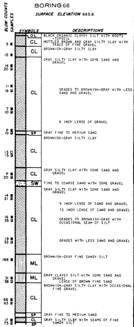
LA SALLE COUNTY STATION UPDATED FINAL SAFETY ANALYSIS REPORT FIGURE 2.5-19 LOGS OF BORINGS (SHEET 90)
