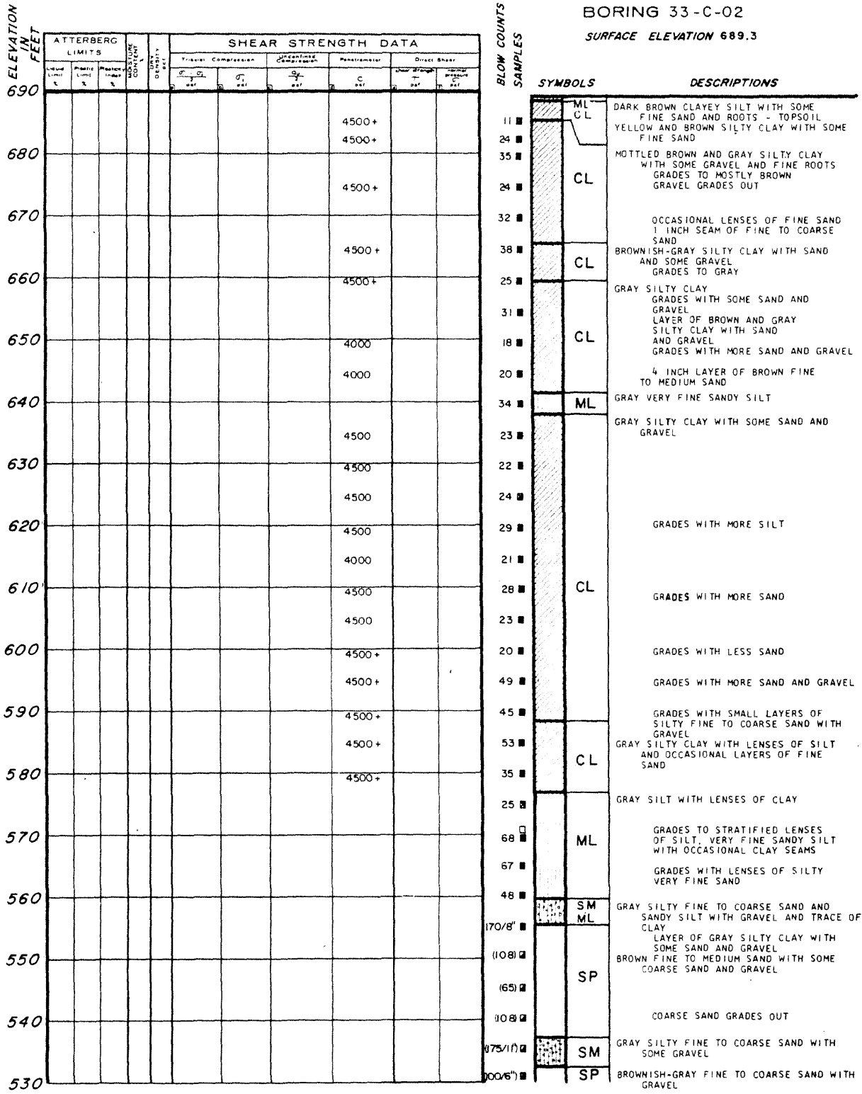
LA SALLE COUNTY STATION UPDATED FINAL SAFETY ANALYSIS REPORT FIGURE 2.5-19 LOGS OF BORINGS (SHEET 178)
