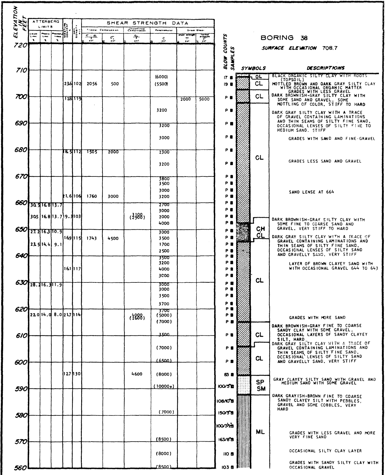
LA SALLE COUNTY STATION UPDATED FINAL SAFETY ANALYSIS REPORT FIGURE 2.5-19 LOGS OF BORINGS (SHEET 50)
