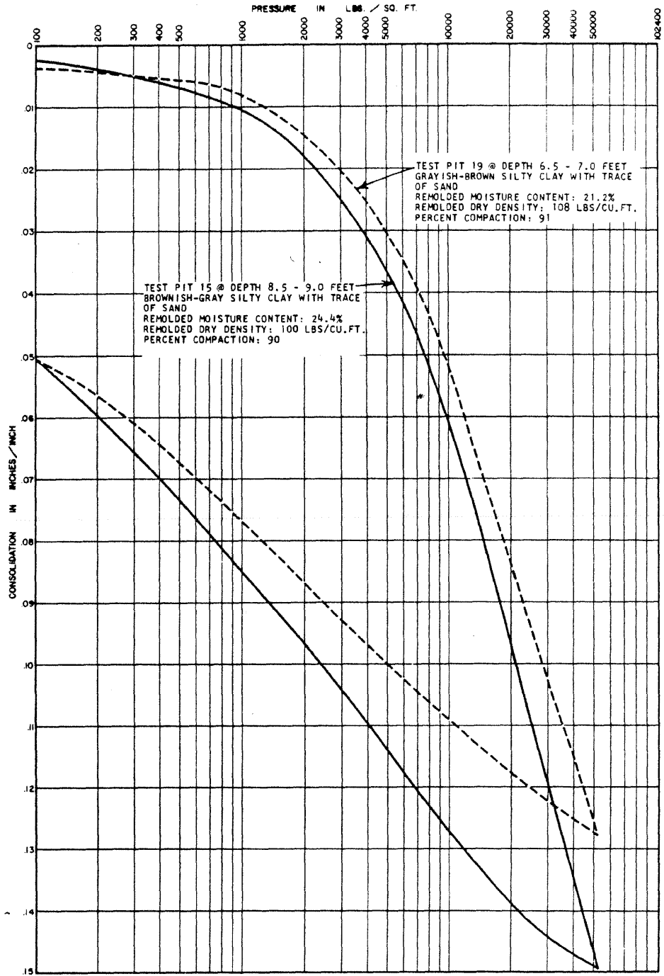
LA SALLE COUNTY STATION UPDATED FINAL SAFETY ANALYSIS REPORT FIGURE 2.5-45 CONSOLIDATION TEST DATA (SHEET 24)
