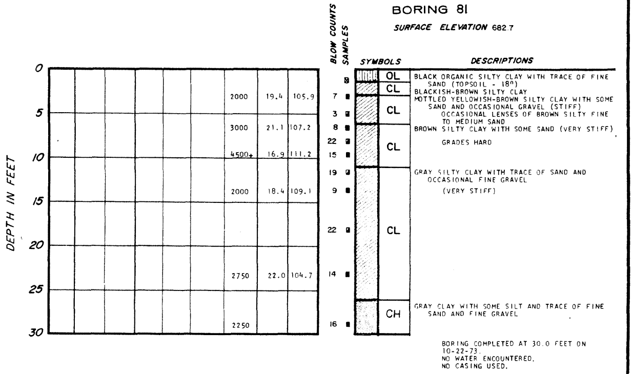
LA SALLE COUNTY STATION UPDATED FINAL SAFETY ANALYSIS REPORT FIGURE 2.5-19 LOGS OF BORINGS (SHEET 103)
