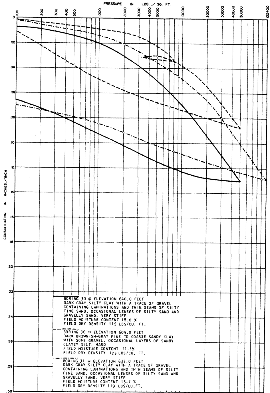
LA SALLE COUNTY STATION UPDATED FINAL SAFETY ANALYSIS REPORT FIGURE 2.5-45 CONSOLIDATION TEST DATA (SHEET 5)
