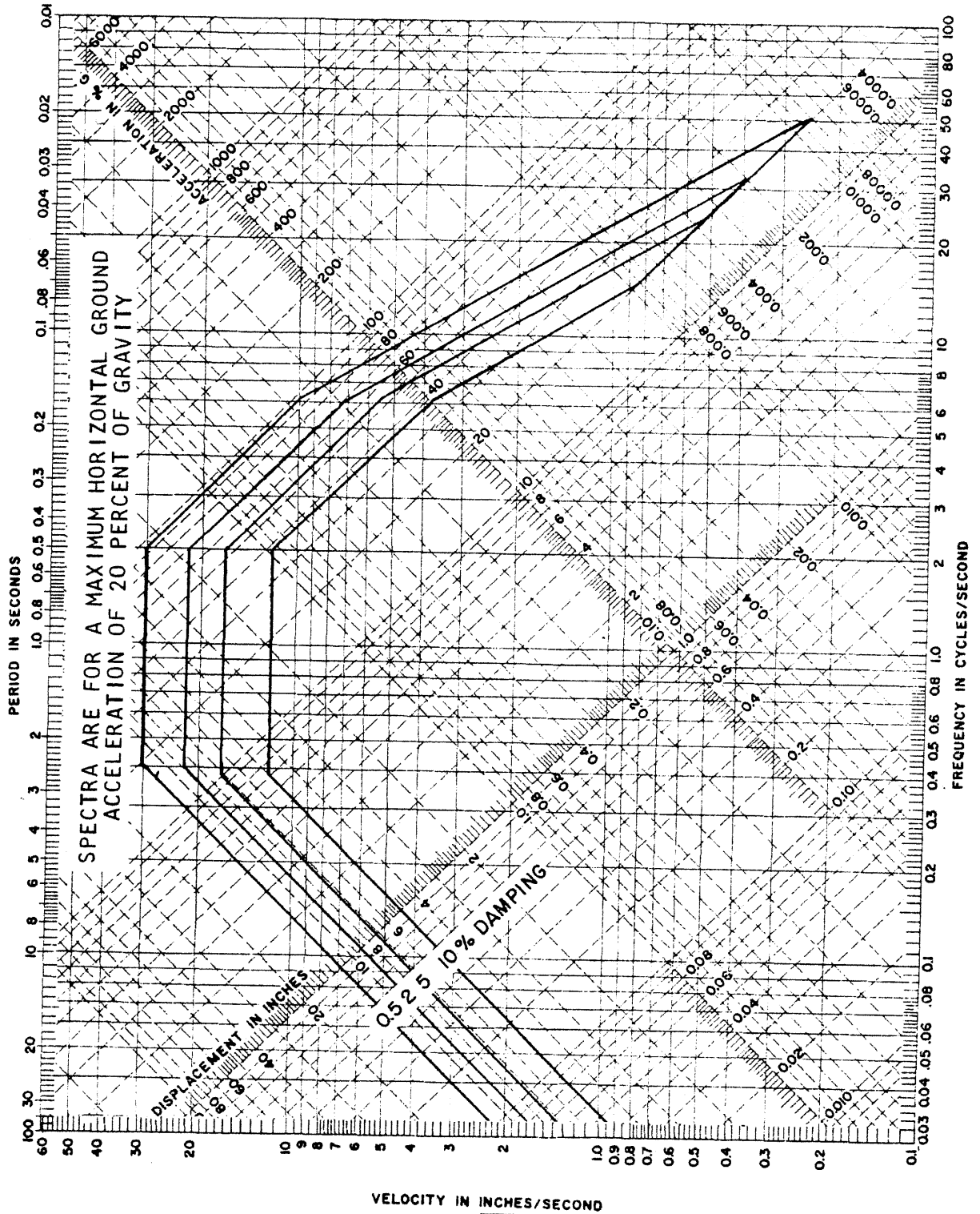
LA SALLE COUNTY STATION UPDATED FINAL SAFETY ANALYSIS REPORT FIGURE 2.5-39 RESPONSE SPECTRA - SAFE SHUTDOWN EARTHQUAKE
