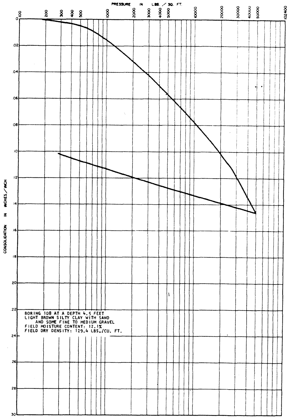
LA SALLE COUNTY STATION UPDATED FINAL SAFETY ANALYSIS REPORT FIGURE 2.5-45 CONSOLIDATION TEST DATA (SHEET 16)
