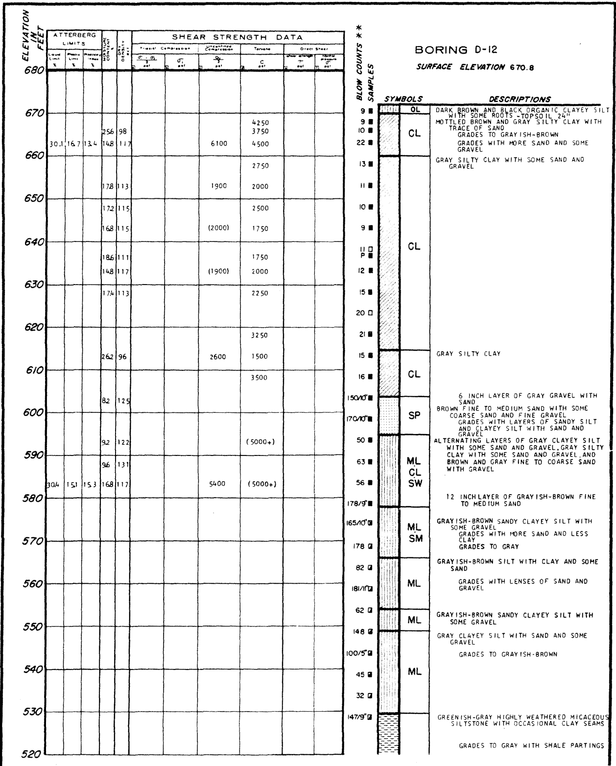
LA SALLE COUNTY STATION UPDATED FINAL SAFETY ANALYSIS REPORT FIGURE 2.5-19 LOGS OF BORINGS REV. 0 - APRIL 1984 (SHEET 196)
