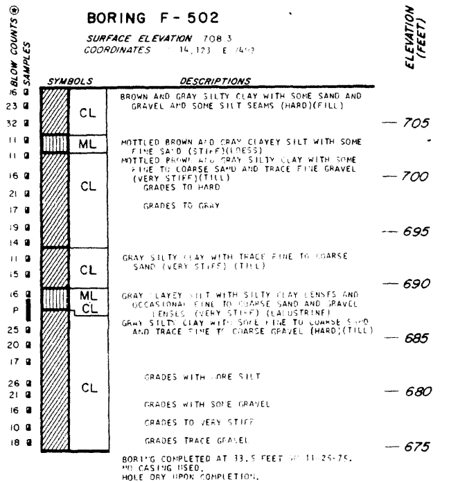
LA SALLE COUNTY STATION UPDATED FINAL SAFETY ANALYSIS REPORT FIGURE 2.5-19 LOGS OF BORINGS (SHEET 248)
