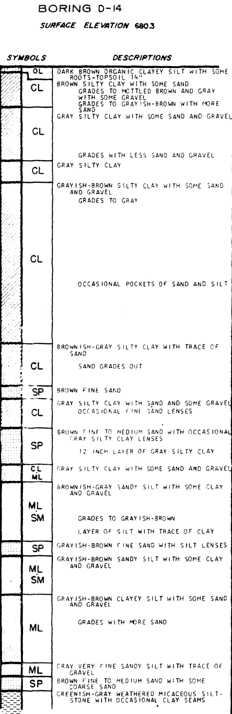
LA SALLE COUNTY STATION UPDATED FINAL SAFETY ANALYSIS REPORT FIGURE 2.5-19 LOGS OF BORINGS (SHEET 199)
