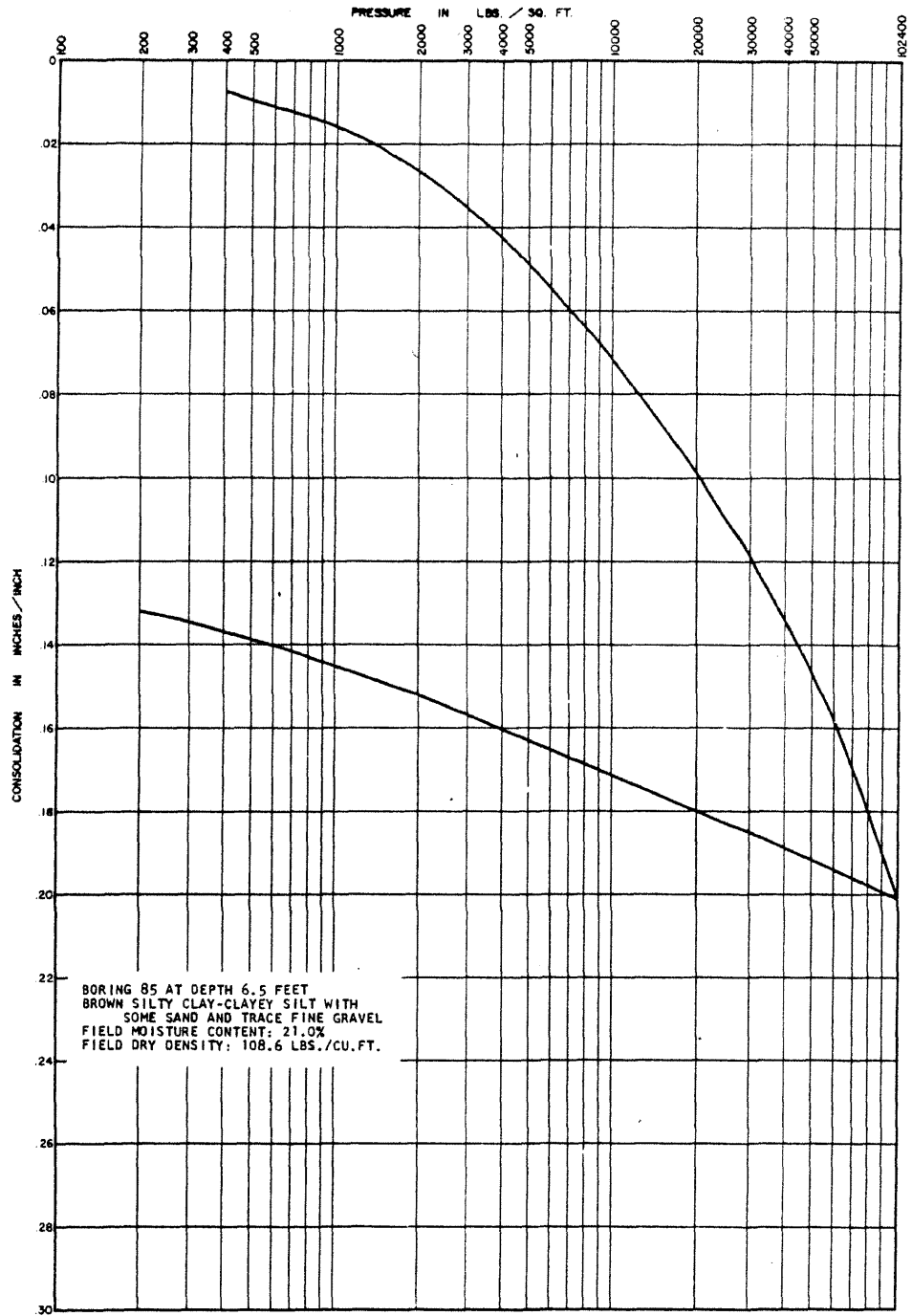
LA SALLE COUNTY STATION UPDATED FINAL SAFETY ANALYSIS REPORT FIGURE 2.5-45 CONSOLIDATION TEST DATA (SHEET 13)
