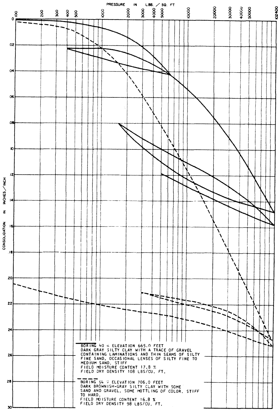
LA SALLE COUNTY STATION UPDATED FINAL SAFETY ANALYSIS REPORT FIGURE 2.5-45 CONSOLIDATION TEST DATA (SHEET 8)
