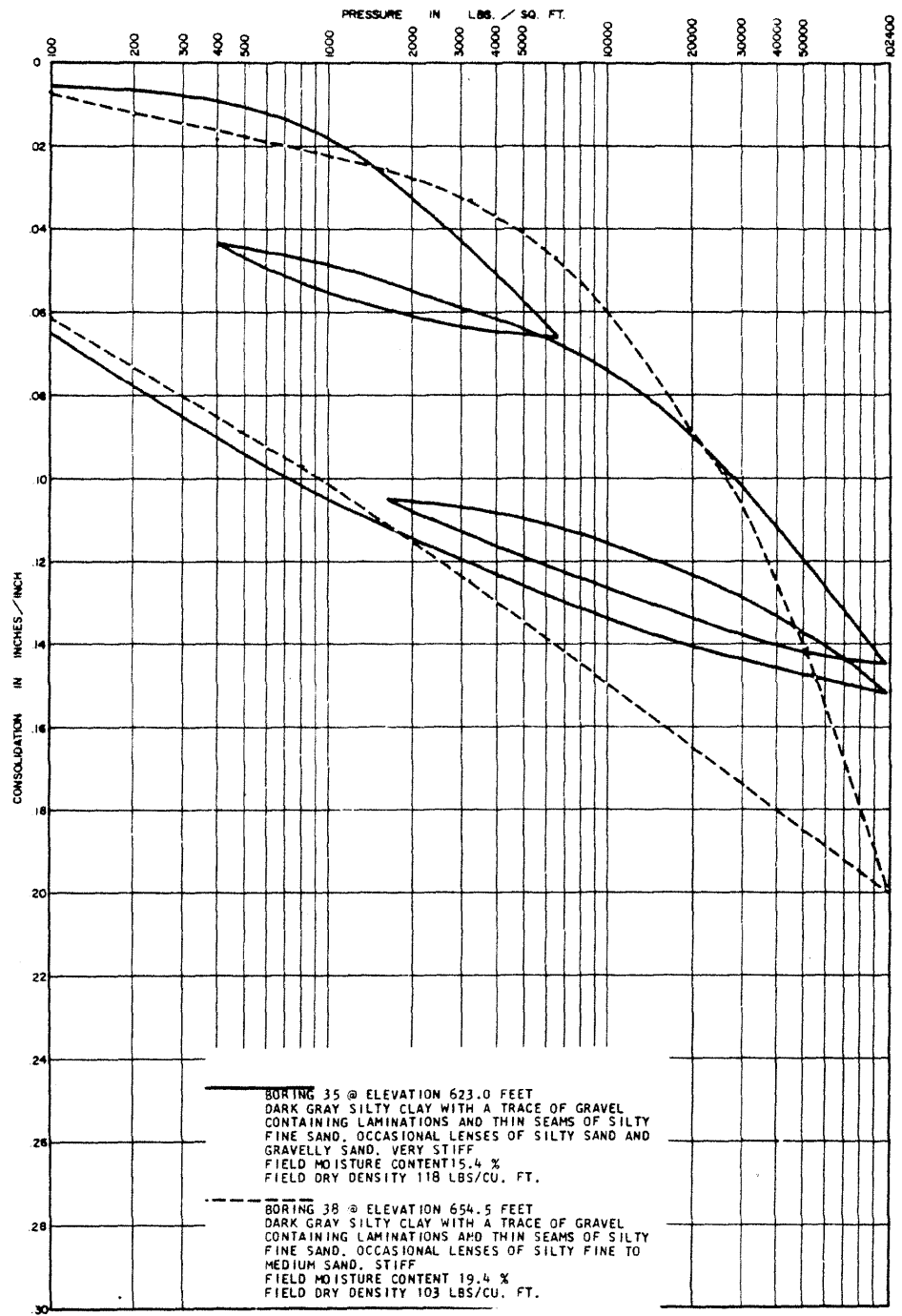
LA SALLE COUNTY STATION UPDATED FINAL SAFETY ANALYSIS REPORT FIGURE 2.5-45 CONSOLIDATION TEST DATA (SHEET 6)
