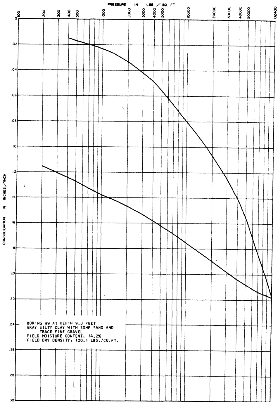
LA SALLE COUNTY STATION UPDATED FINAL SAFETY ANALYSIS REPORT FIGURE 2.5-45 CONSOLIDATION TEST DATA (SHEET 14)
