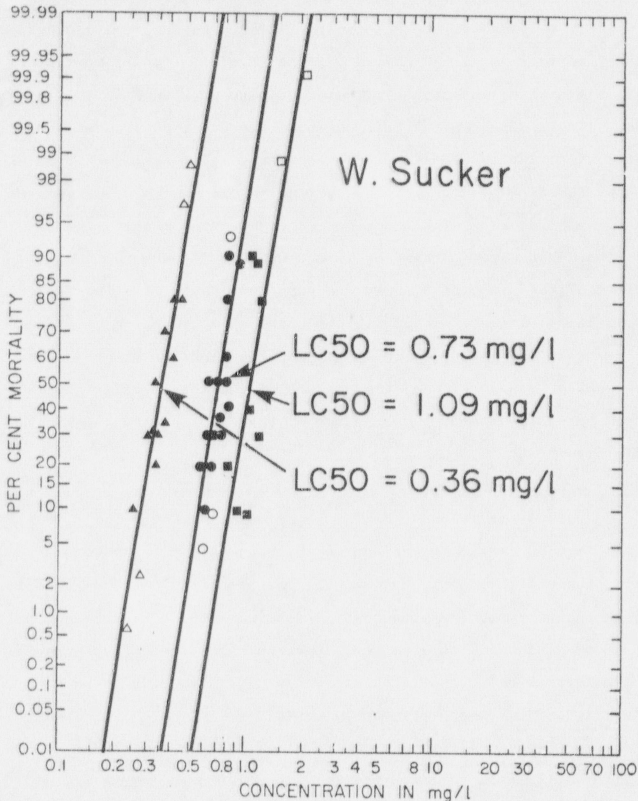
Figure 12. Results of quadruple 40-minute exposures of W. Sucker at 10 (squares), 20C (circles) and 27C (triangles) to residual chlorine. Mortality determined 48 hours later in unchlorinated water. Solid symbols represent observed mortalities; open symbols represent concentrations where 0 and 100% mortality data were transformed.
