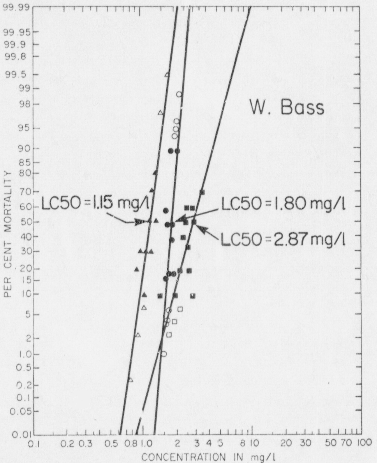
Figure 8. Results of quadruple 40-minute exposures of W. Bass at 10 (squares), 20 (circles), and 30 (triangles) to residual chlorine. Mortality determined 48 hours later in unchlorinated water. Solid symbols represent observed mortalities; open symbols represent concentrations where 0% or 100% mortality data were transformed.
