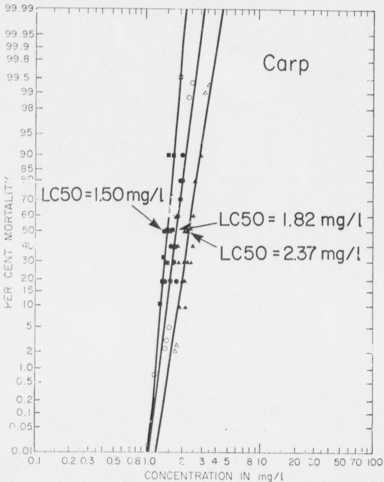
Figure 7. Results of quadruple 40-minute exposures of carp at 10 (triangles), 20 (circles), and 30C (squares) to residual chlorine. Mortality determined 48 hours later in unchlorinated water. Solid symbols represent observed mortalities; open symbols represent concentrations where 0% and 100% mortality data were transformed.
