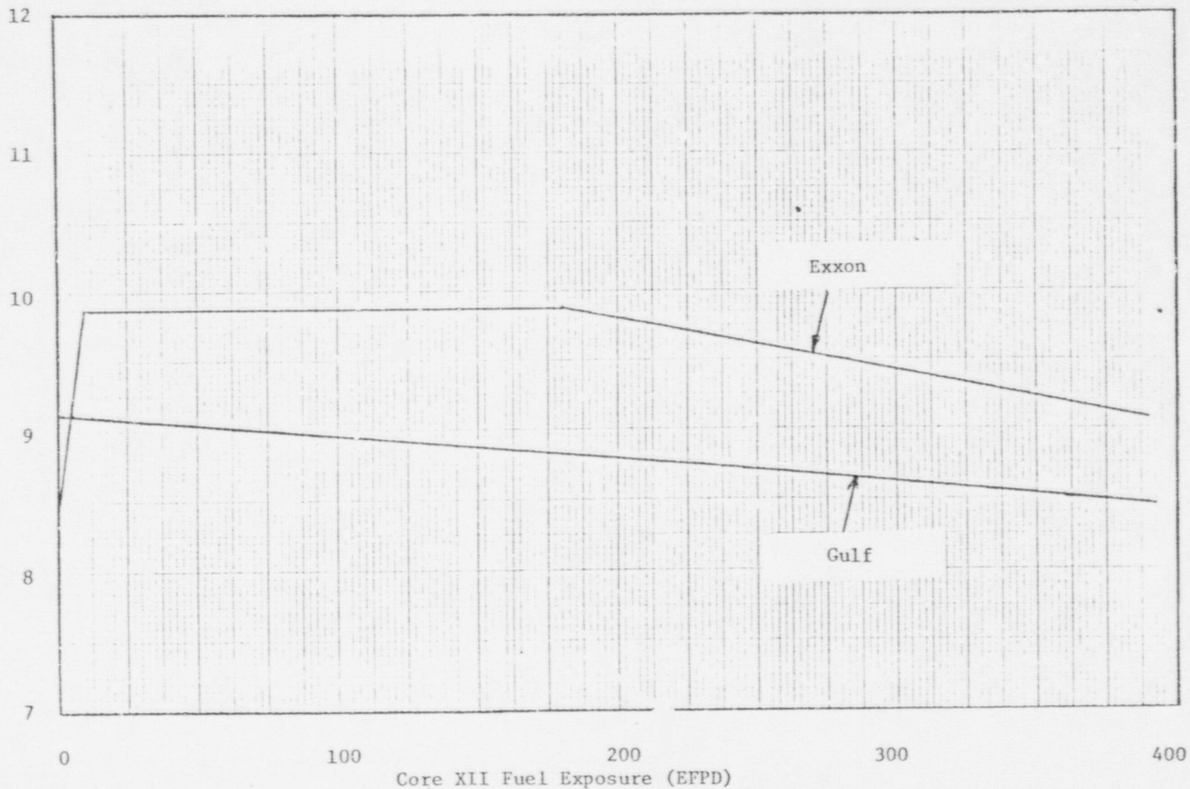
Figure 3.2-1 Core XII Allowable Peak Rod LHGR versus Exposure
