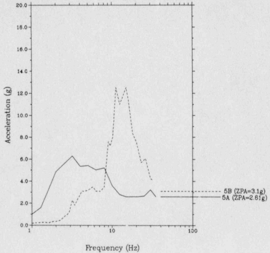
Fig. 3-5a Horizontal TRS @ 5% Damping - MCC Starter Auxiliary Contact
