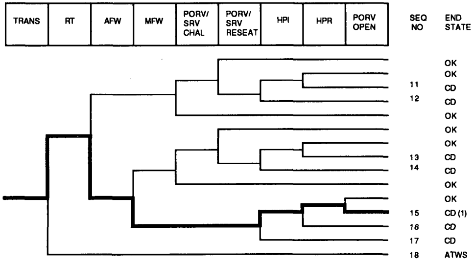
Dominant core damage sequence for LER 400/89-017
