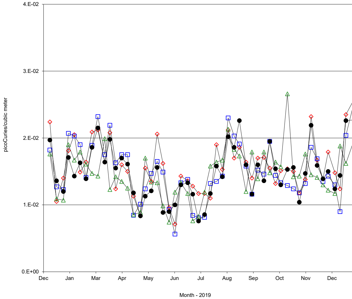
Figure 2.5-2 Airborne Gross-Beta Radioactivity Levels: Property Line Monitors
