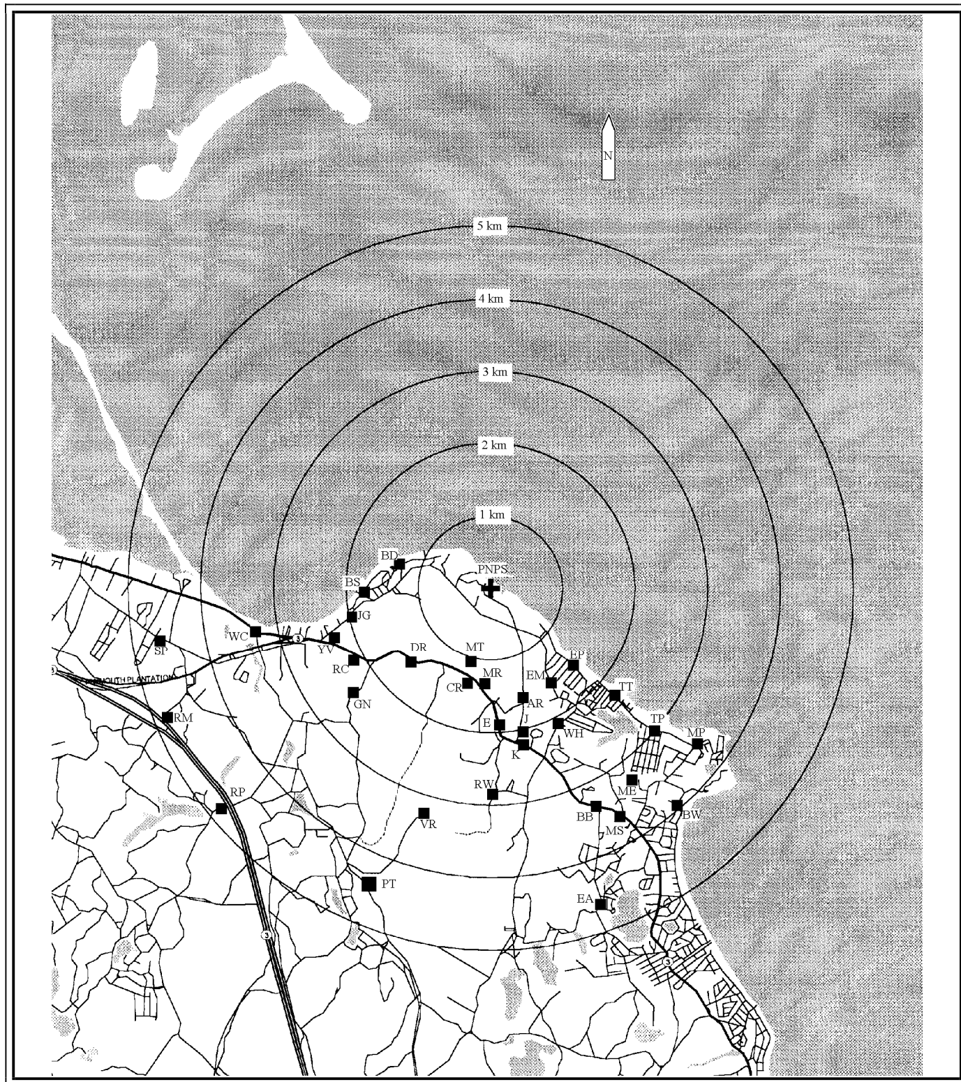
TLD and Air Sampling Locations: 1 to 5 Kilometers
