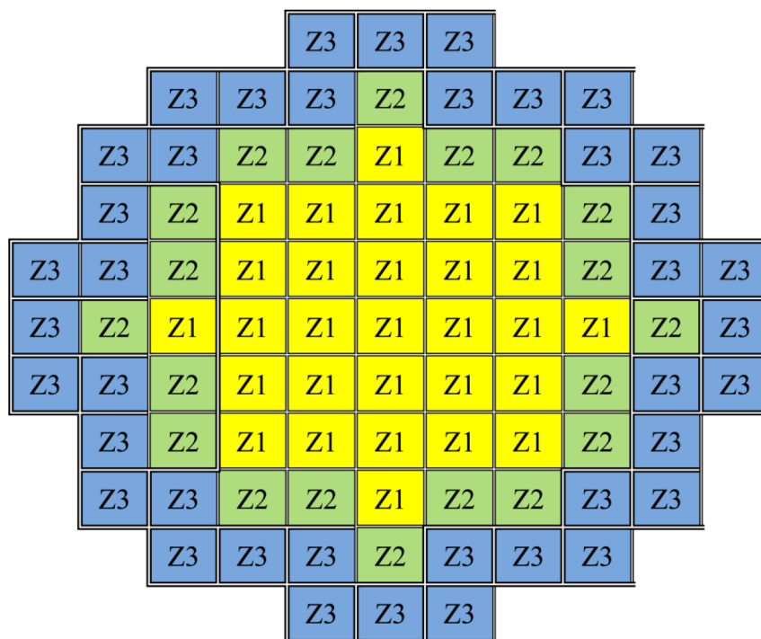
Heat Load Zone Configuration 1 for the EOS-89BTH DSC in the EOS-TC125 Stored in the EOS-HSM
