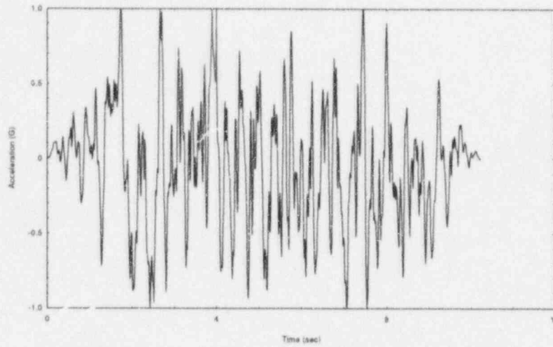
Figure 4a. Time History corresponding to 1.0g Reg Guide 1.60 response spectrum
