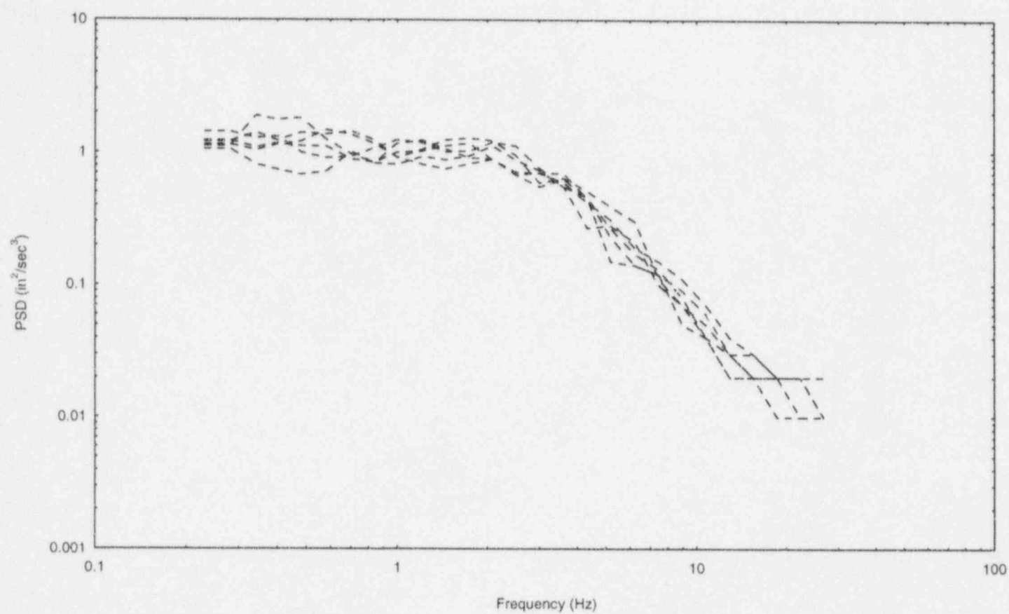
Figure 5. PSDs of the Time Histories in Figures 1a through 1f
