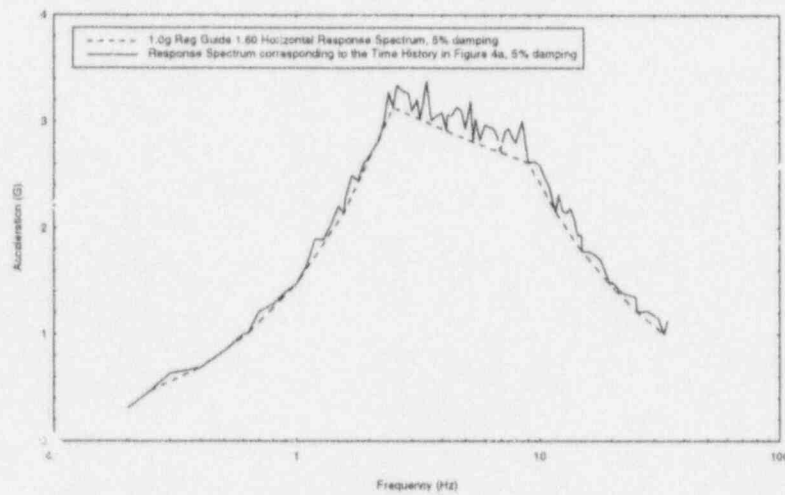
Figure 4b. Comparison of Response Spectra
