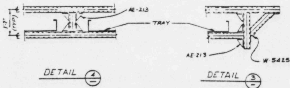
DETAILS OF RIGID SUPPORT
