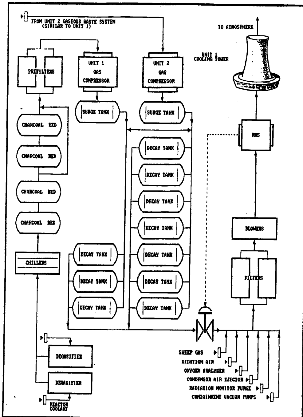
BV-1 AND 2 GASEOUS RADWASTE SYSTEM
