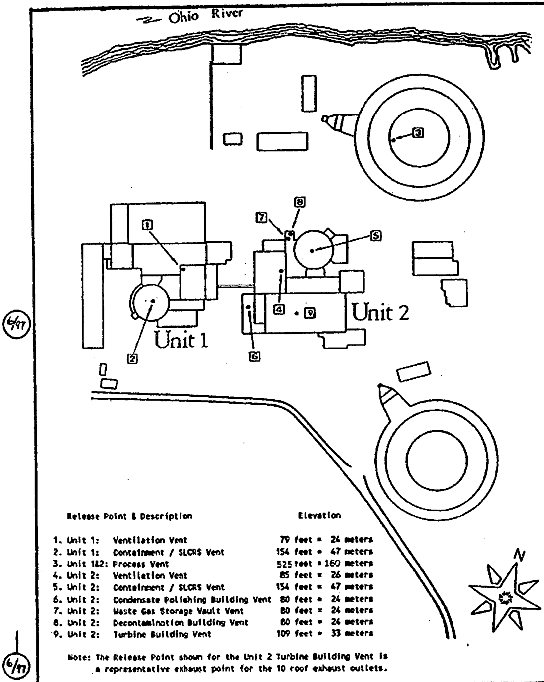
BV-1 AND 2 GASEOUS EFFLUENT RELEASE POINTS
