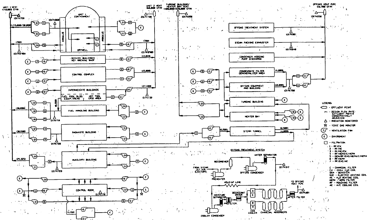
Figure 3.0-1 Gaseous Effluent System Flow Diagram
