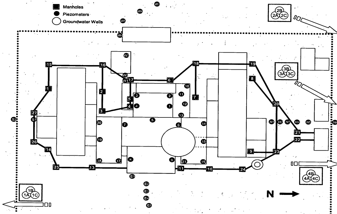
Figure 2: Underdrain System and Groundwater Monitoring Wells
