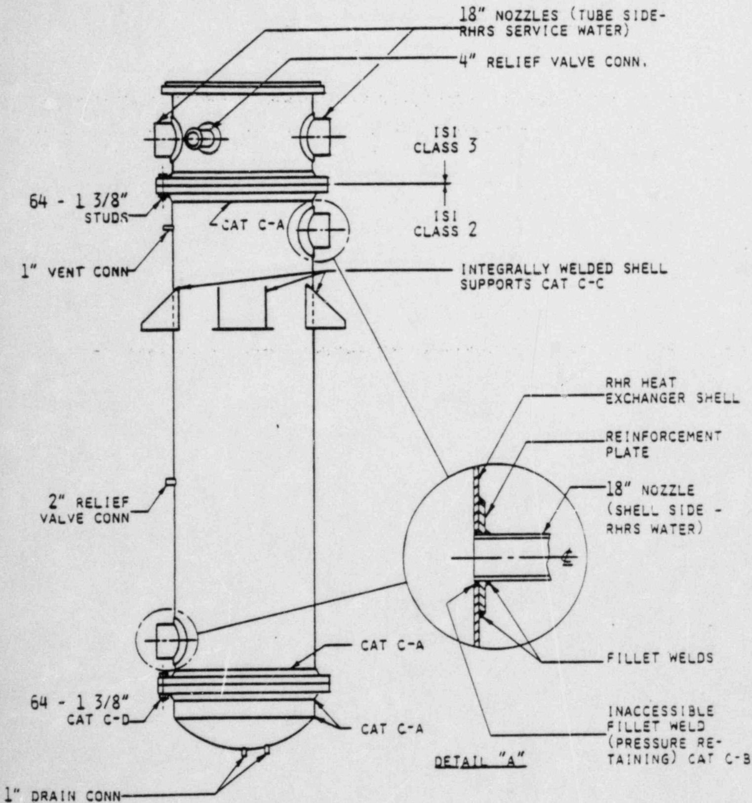
FIGURE 5 RHR HEAT EXCHANGERS
