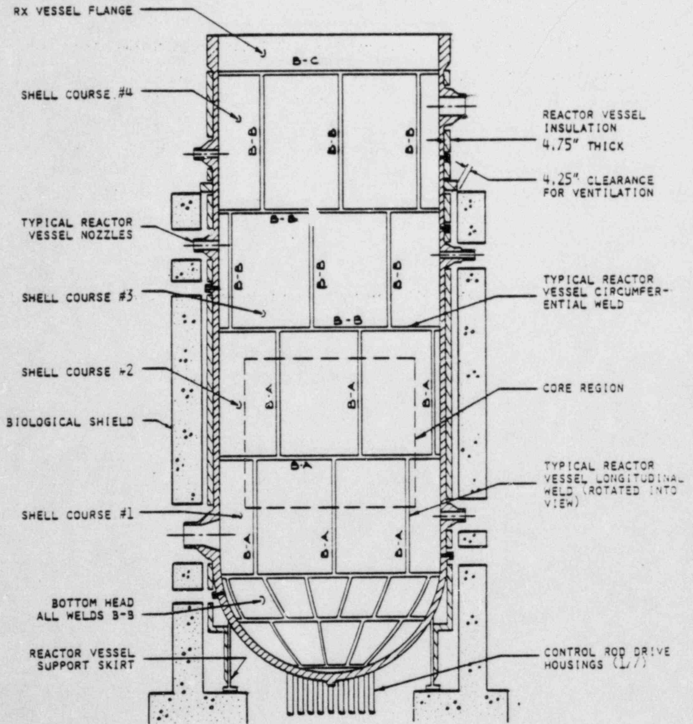
FIGURE 1.a REACTOR VESSEL WELD IDENTIFICATION
