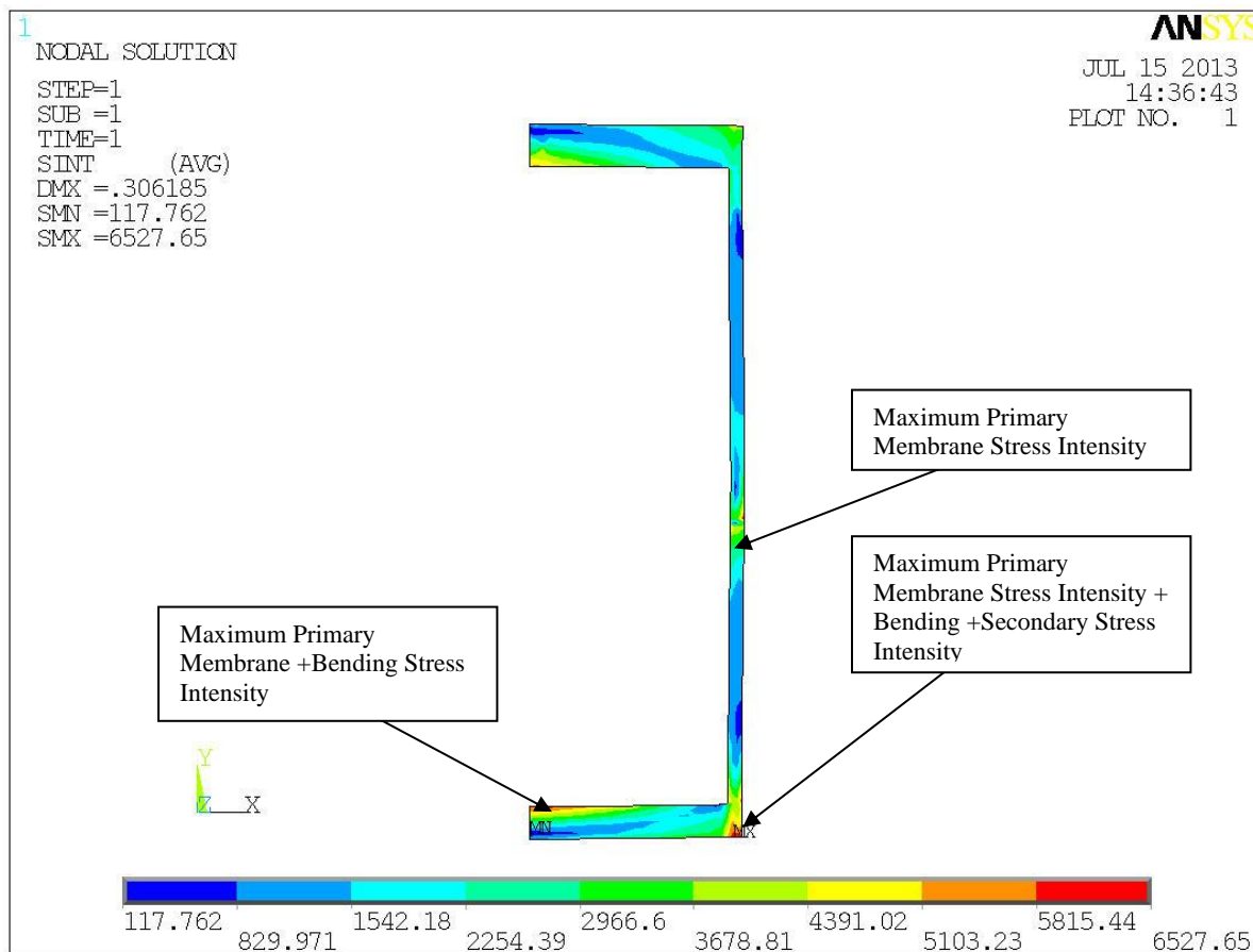
Figure 2.6.4: Results for Stress Intensity for Load Combination N1
