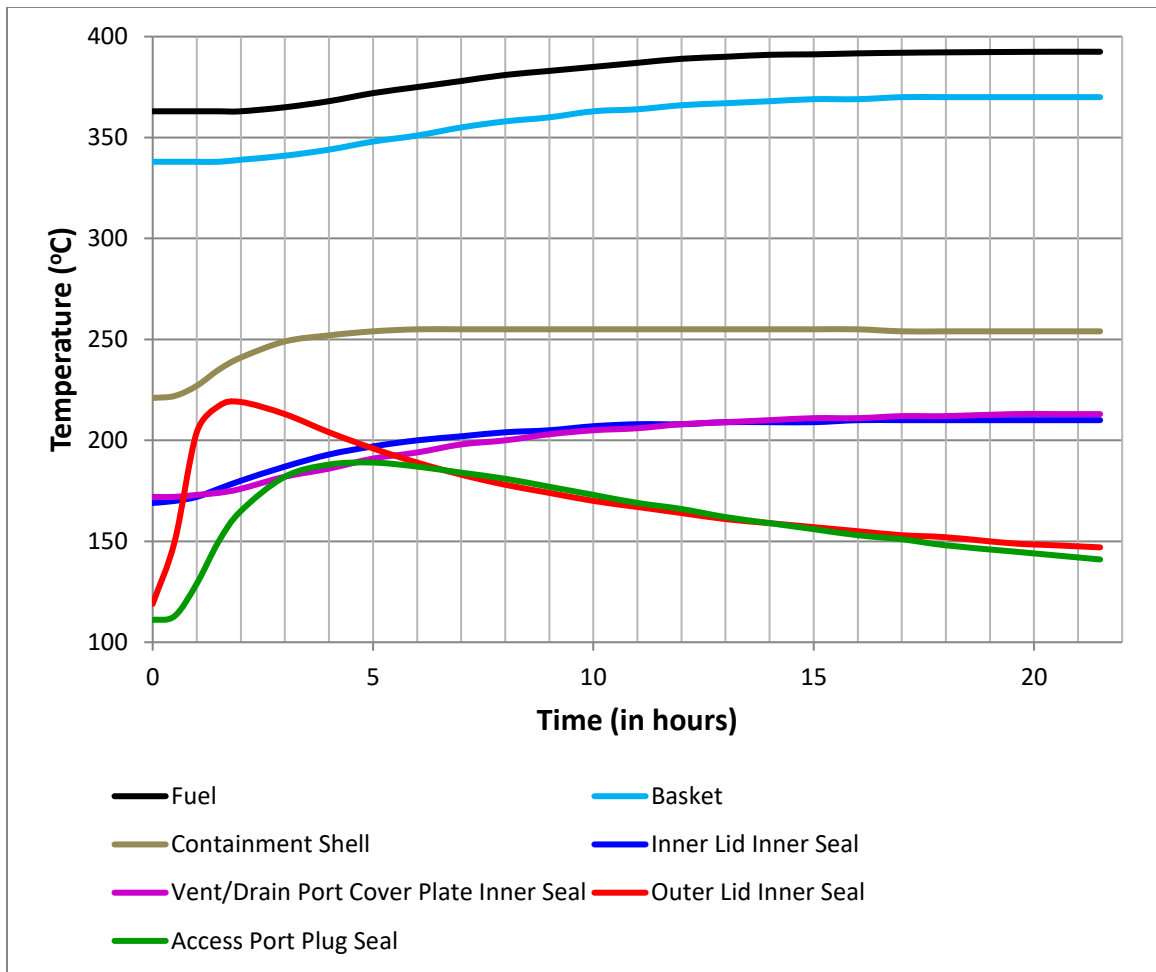
FIGURE 3.4.1: HI-STAR 180D FIRE AND POST FIRE COOLDOWN TEMPERATURE HISTORY
