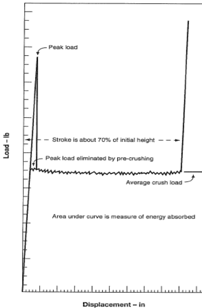
Figure 2.2.1: Load vs. Displacement Curve for Aluminum Crush Material (Typical, reproduced from [2.1.1])
