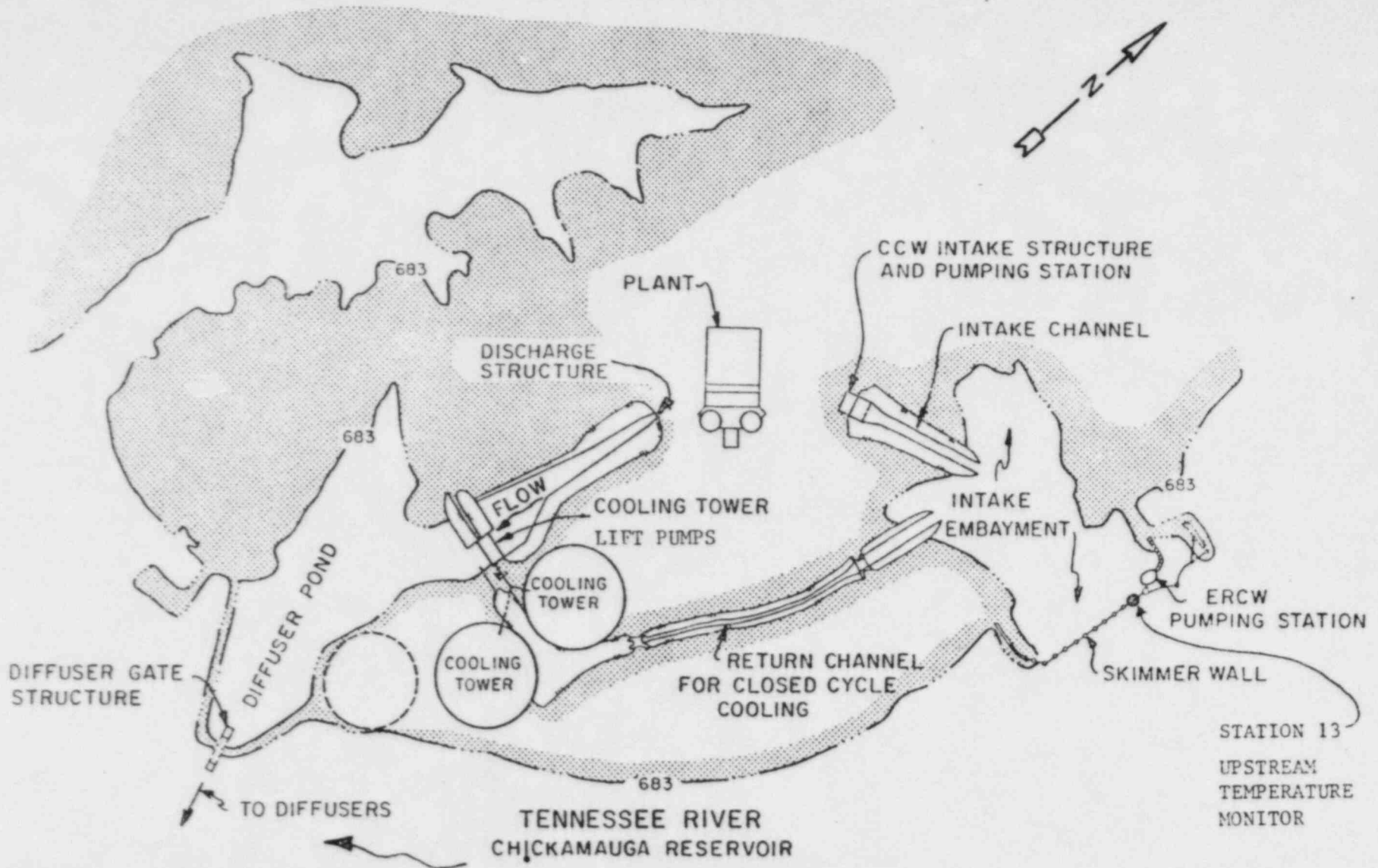
Figure 1: General Plan of the Sequoyah Nuclear Plant
