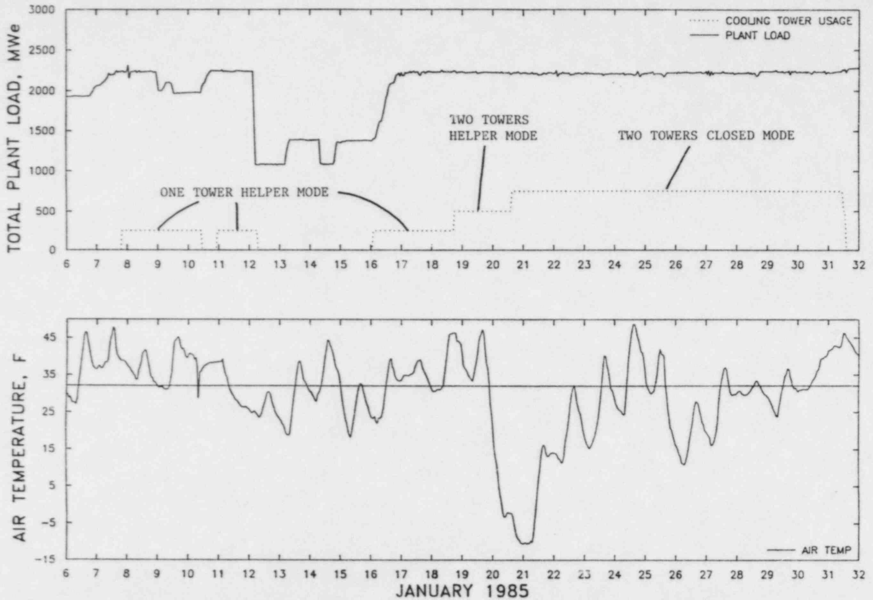
FIGURE 2. SEQUOYAH NUCLEAR PLANT OPERATION AND AIR TEMPERATURES - JANUARY 1985.
