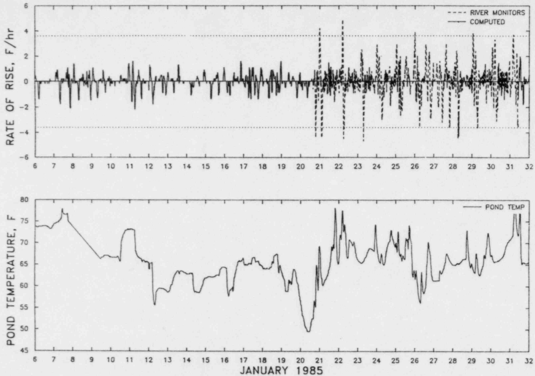
FIGURE 4. SEQUOYAH NUCLEAR PLANT RATE OF TEMPERATURE CHANGE AND DISCHARGE POND TEMPERATURES - JANUARY 1985.
