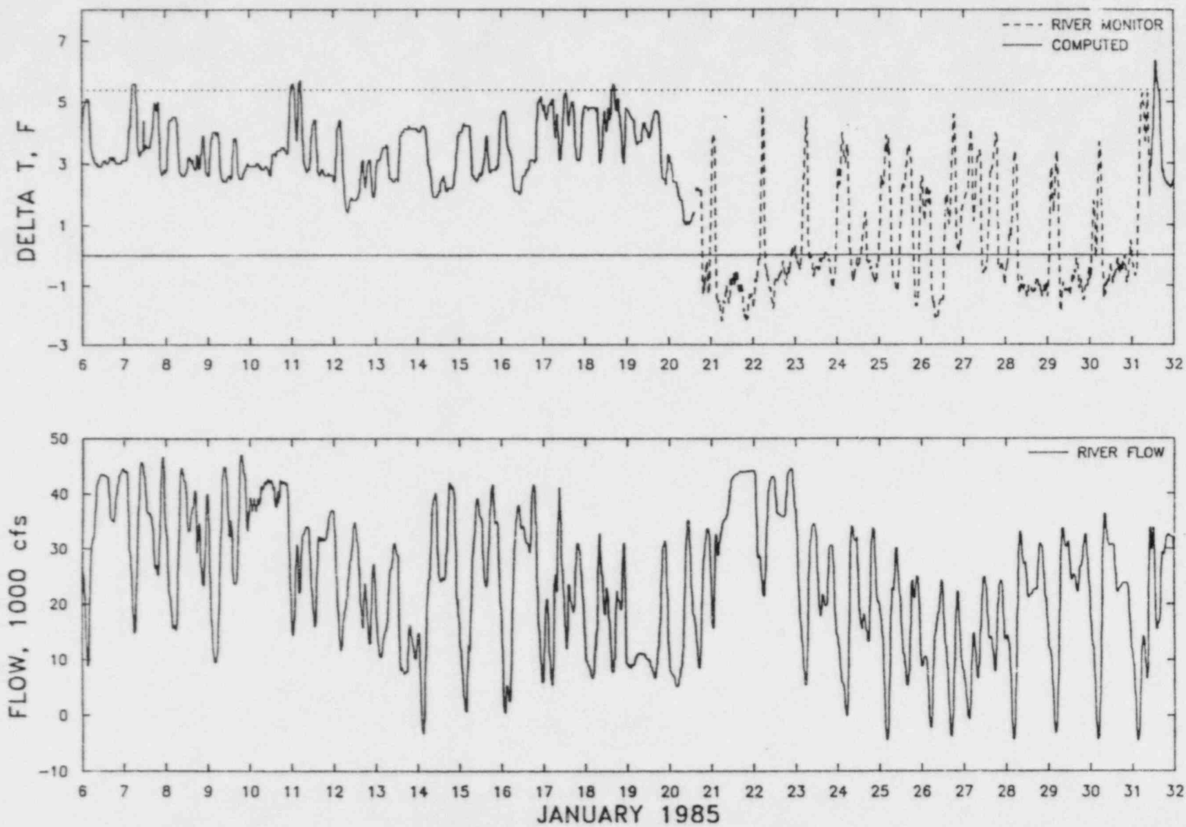
FIGURE 3. SEQUOYAH NUCLEAR PLANT TEMPERATURE RISE AND RIVER FLOW - JANUARY 1985.
