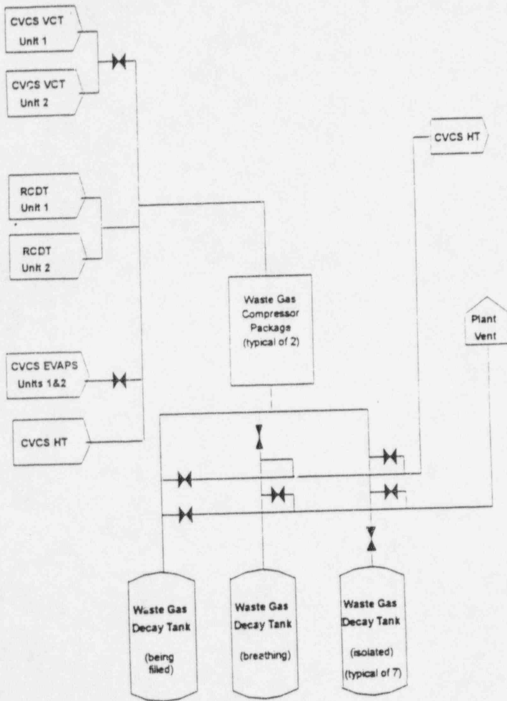
Figure 7.3 GASEOUS RADWASTE TREATMENT SYSTEM
