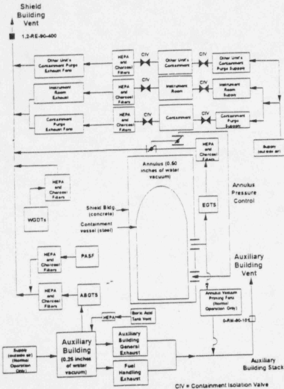
Figure 7.2 AUXILIARY AND SHIELD BUILDING VENTS (DETAIL)
