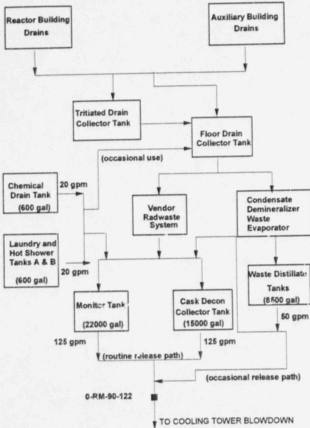
Figure 6.2 LIQUID RADWASTE SYSTEM
