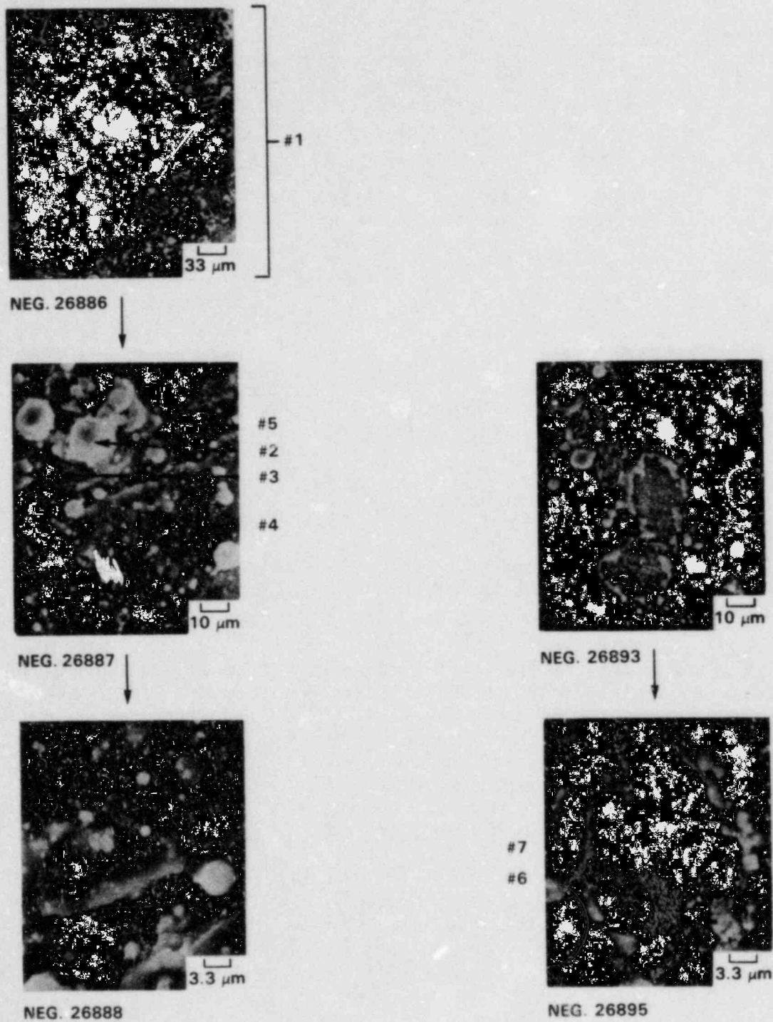
FIGURE 7-2. SEM Examination of the Primary Side Surface of the Pre-Decontamination Core Specimen From the Cold Leg Channel Head Wall
