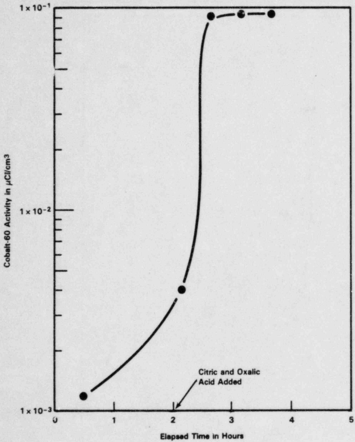
FIGURE 2. ACTIVITY RELEASED AT THE PERMANGANATE DESTRUCTION AND DECONTAMINATION PHASES OF THE AP/POD TREATMENT
