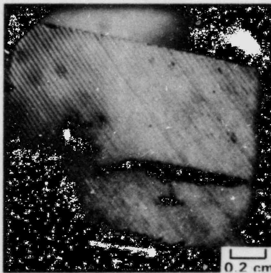
FIGURE 7-26. Appearance of Hot Leg and Recycled Cold Leg Marway Coupons After the Hot Leg Decontamination
