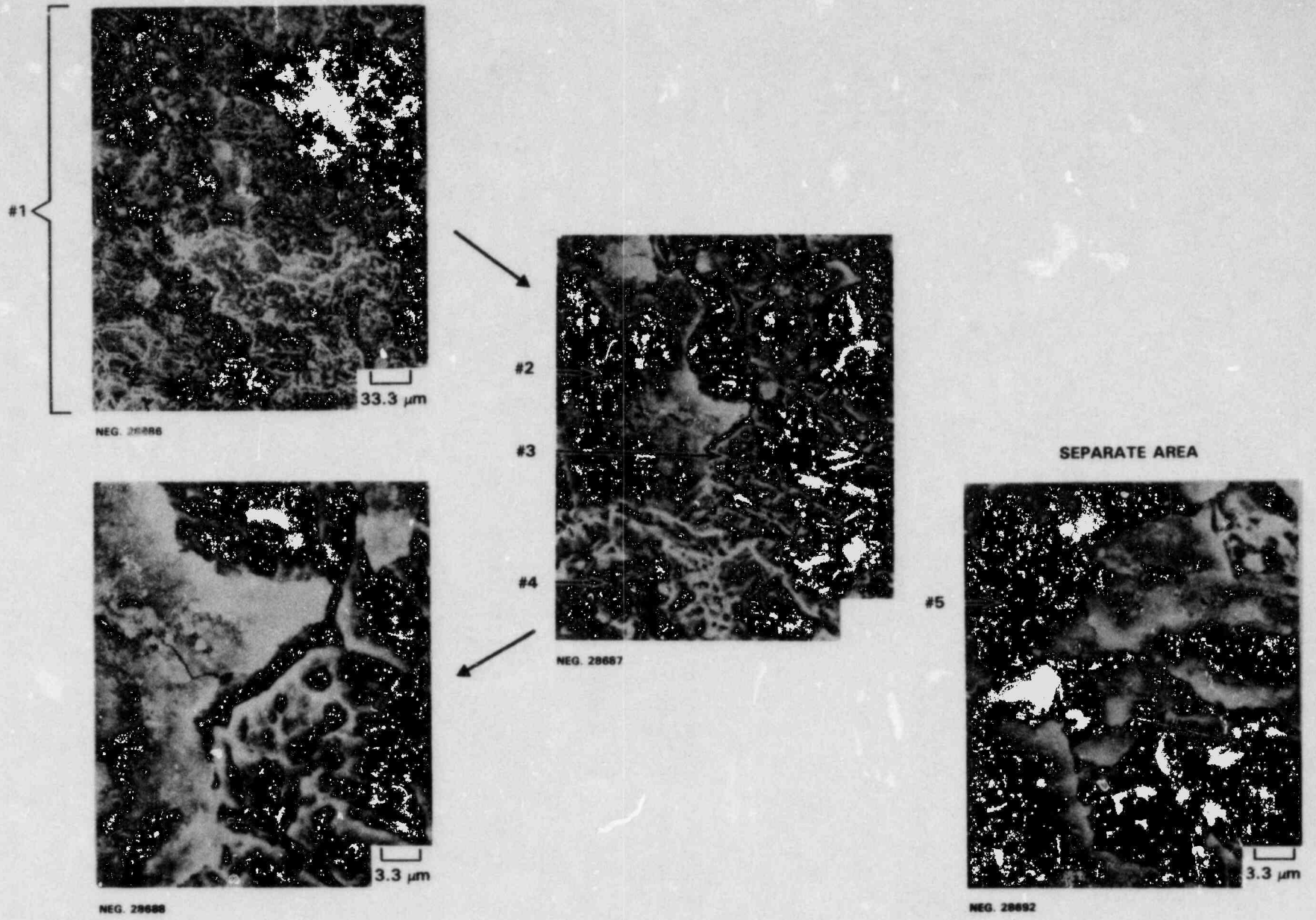
FIGURE 7-36. SEM Examination of a Specimen From the Unprotected Area of the Hot Leg Tube Sheet
