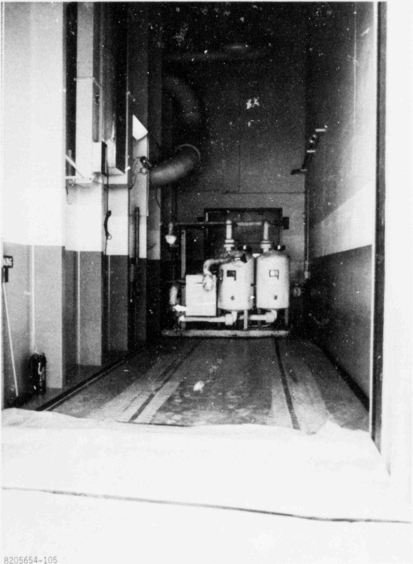
FIGURE 3-6. Size of Decontamination Equipment Compared with Available Space
