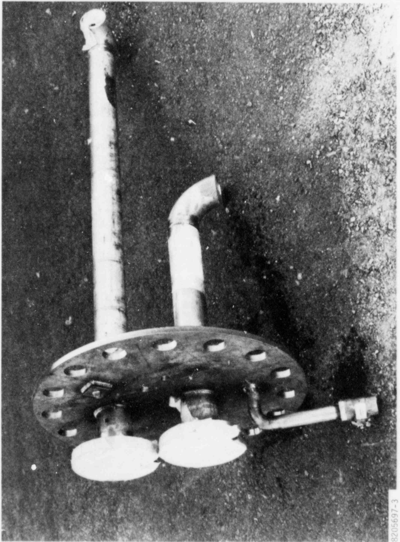
FIGURE 3-7. Nozzle and Return System Used for the Cold Leg Decontamination Operation
