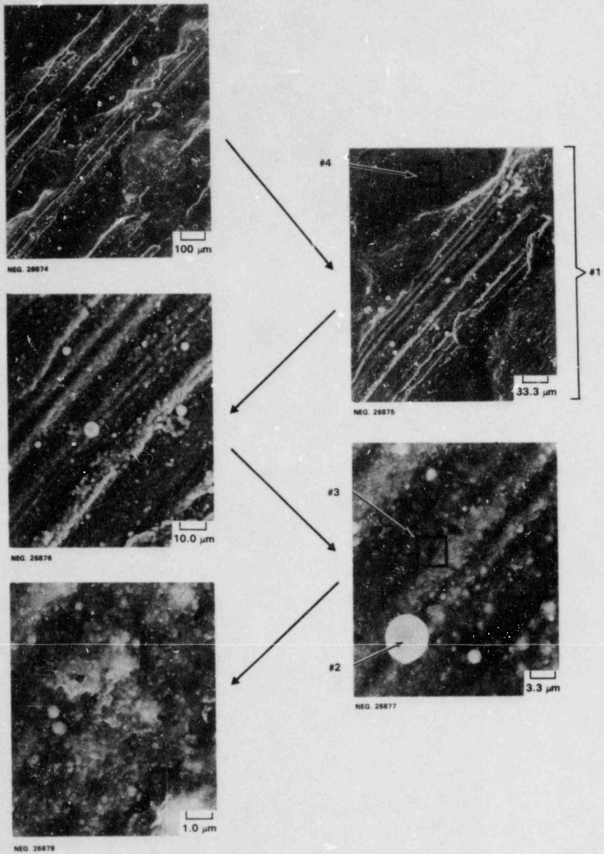
FIGURE 7-7. SEM Examination of the Primary Side Surface of the Pre-Decontamination Core Specimen From the Hot Leg Channel Head Wall
