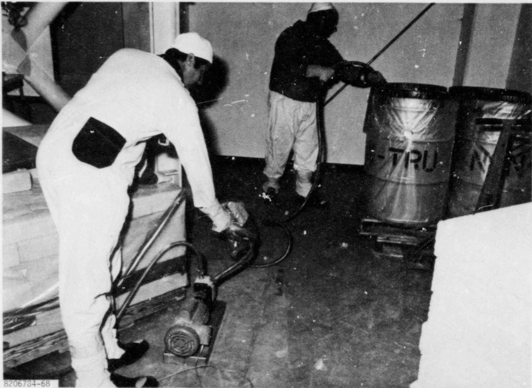
FIGURE 3-21. Dewatering the Resin
