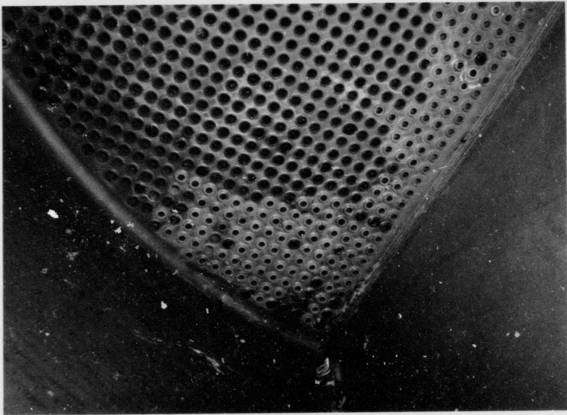
FIGURE 3-15. Cold Leg Surfaces Before Decontamination
