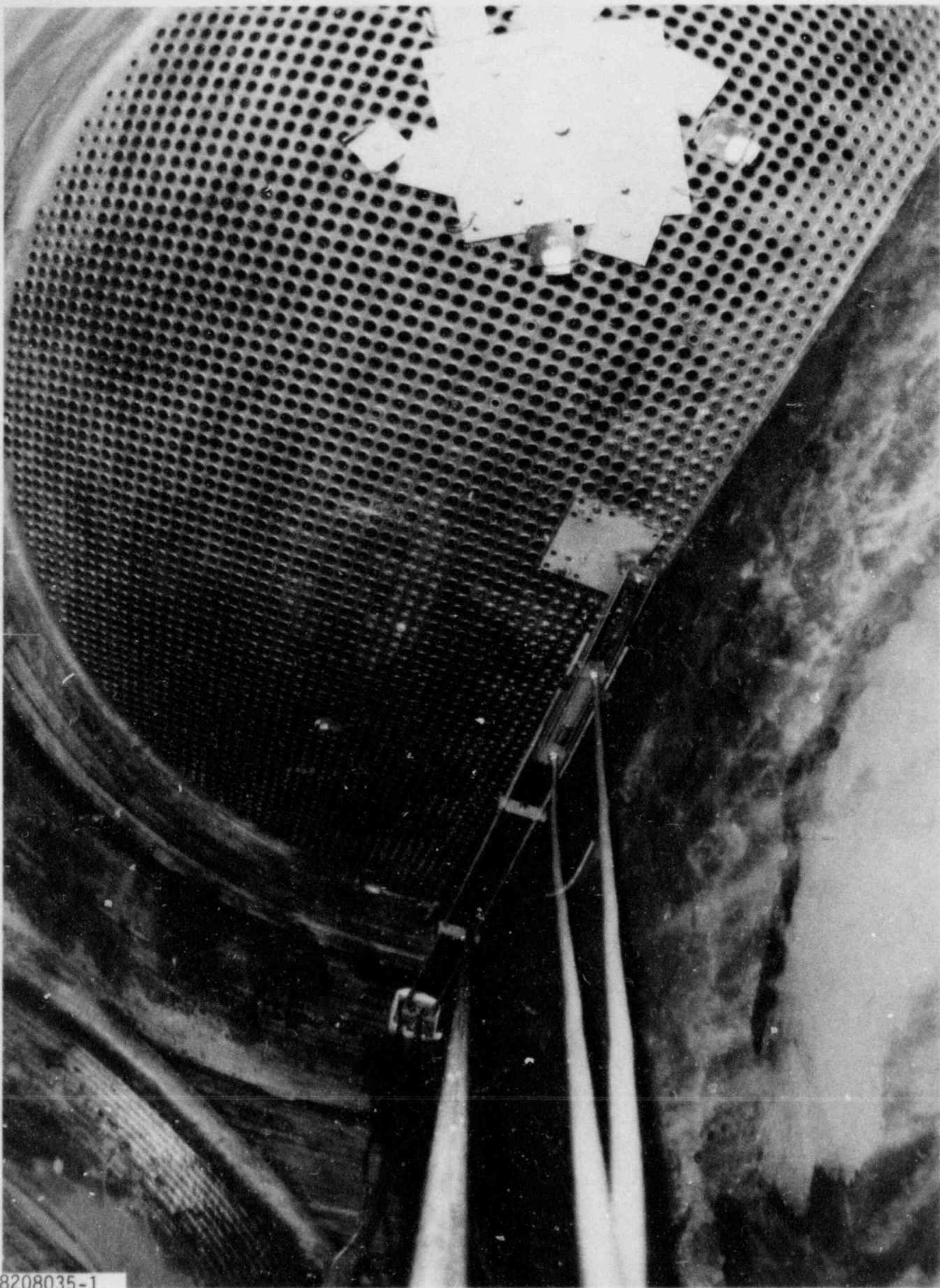
FIGURE 4-14. Electropolished Area on the Inconel 600 Divider Plate
