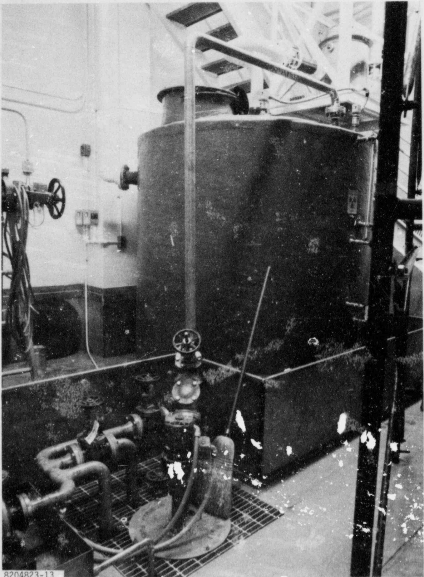
FIGURE 2-15. Basement Liquid Waste Hold Tank
