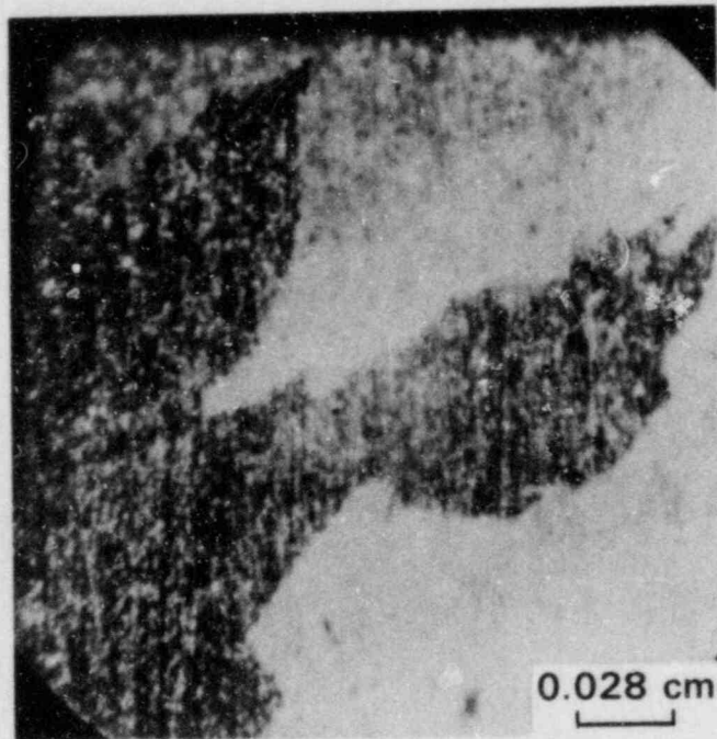
FIGURE 6-12. Prefilmed Corrosion Coupons After the Cold Leg Decontamination
