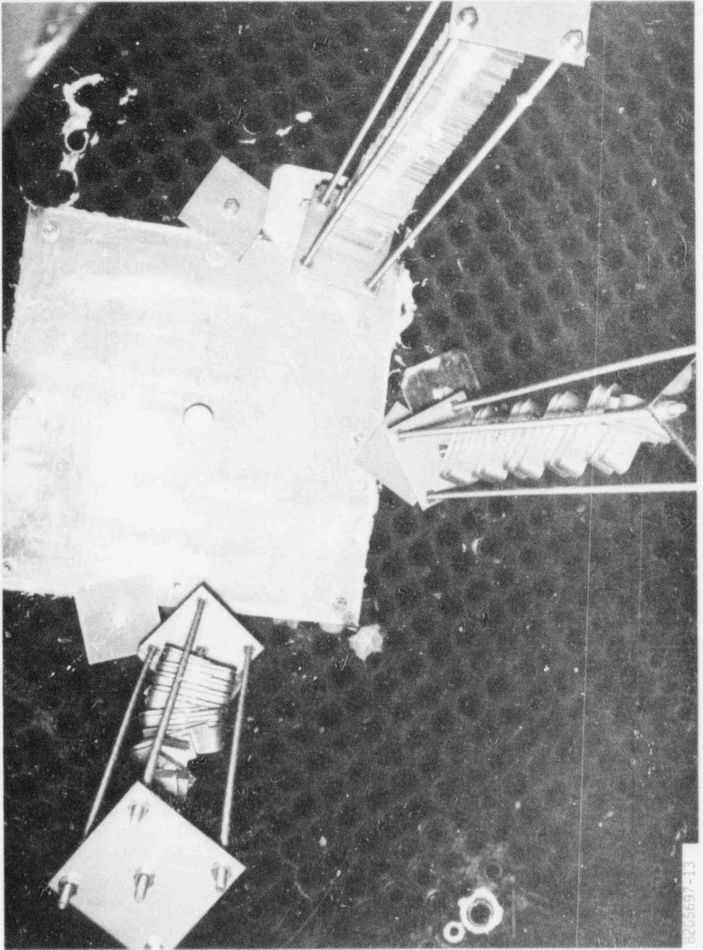
FIGURE 2-5. Installed Protective Plate and Corrosion Specimens for Cold Leg Decontamination
