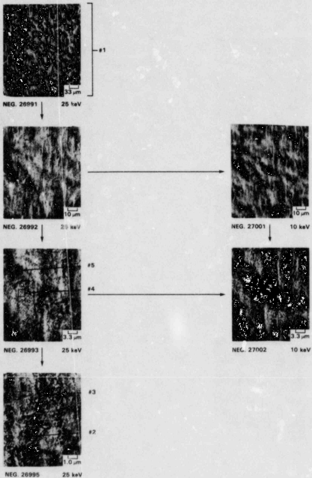
FIGURE 7-14. SEM Examination of the Primary Side Surface of Specimen R-7 From Steam Generator Tube R1C94 Before Decontamination
