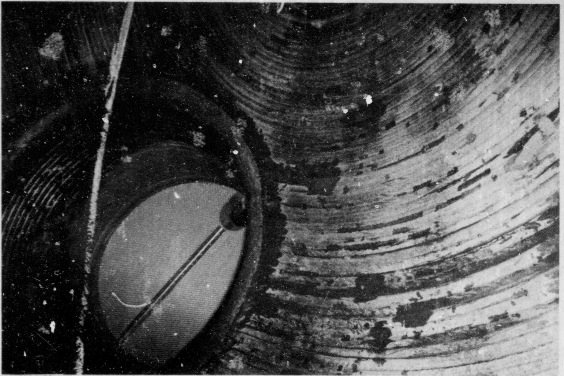
FIGURE 2-12. Installed Nozzle Cover Coating and Hold-Down
