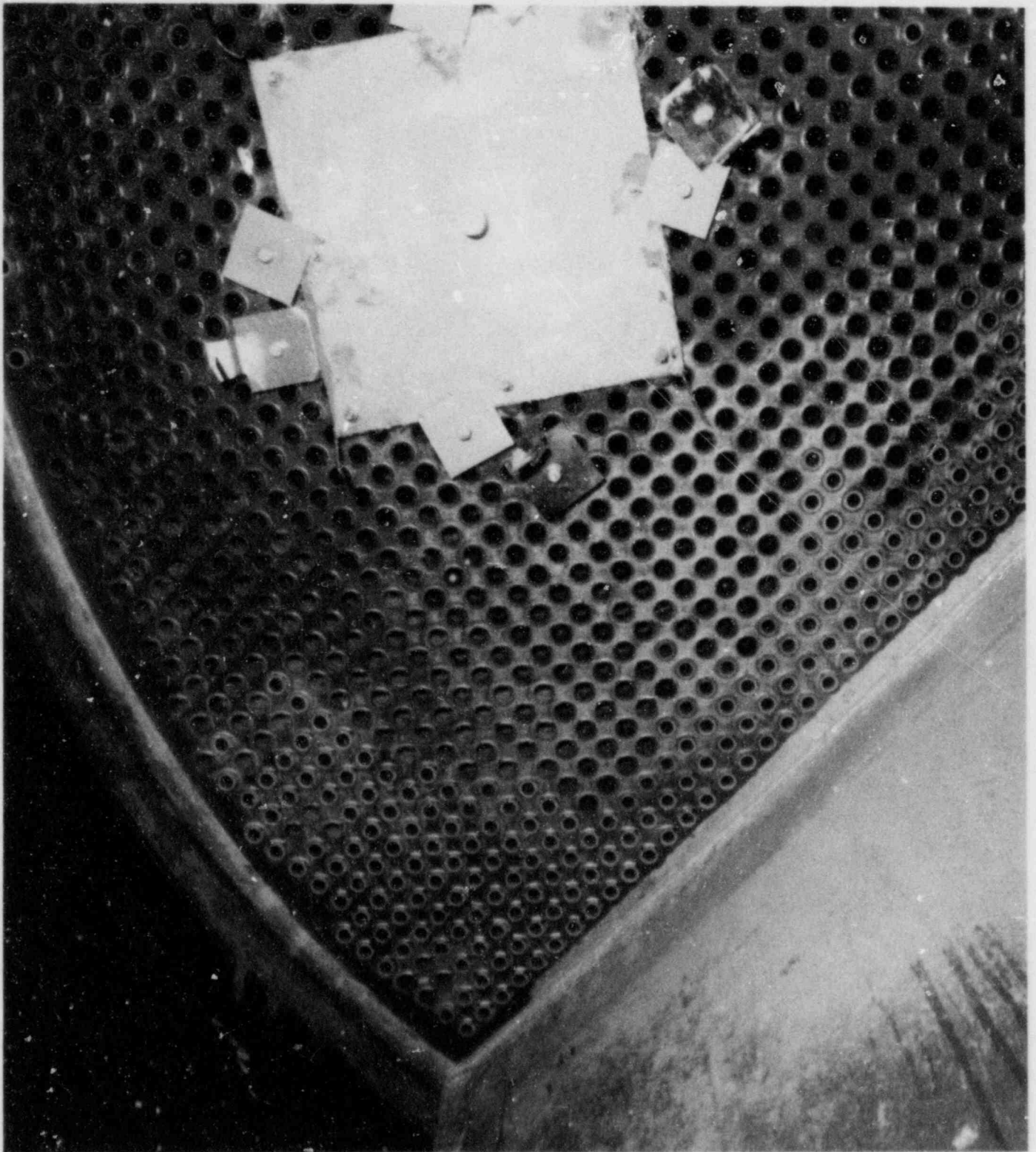
FIGURE 3-16. Cold Leg Surfaces After Two Decontamination Cycles
