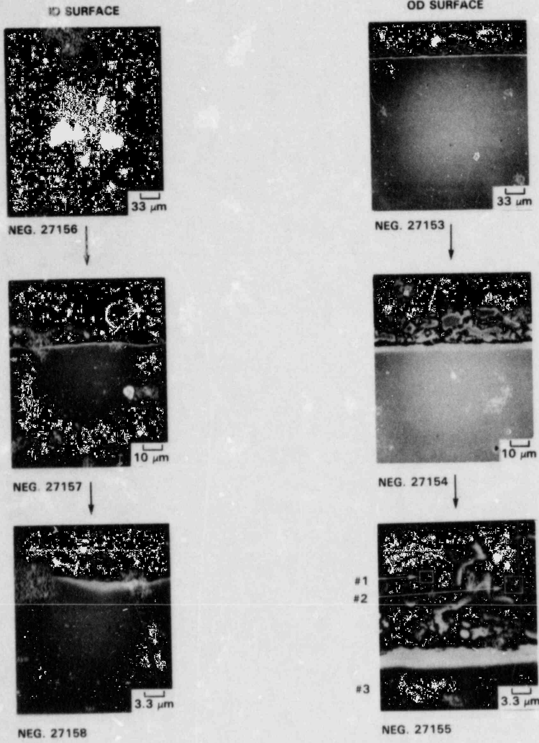
FIGURE 7-15. SEM Examination of Primary and Secondary Sides of a Metallographic Cross Section of the Undecontaminated Steam Generator Tube Specimen R-7
