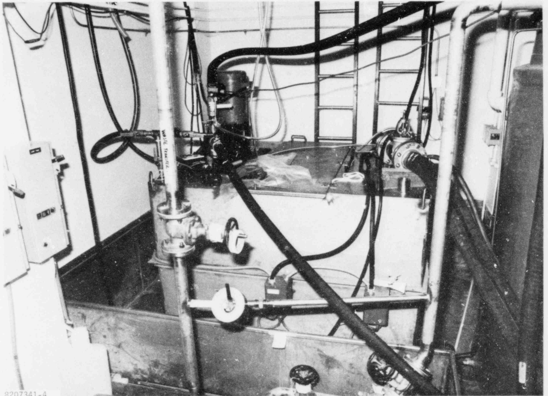
FIGURE 4-2. Surge Tank, Heater and Pump System for Hot Leg Decontamination
