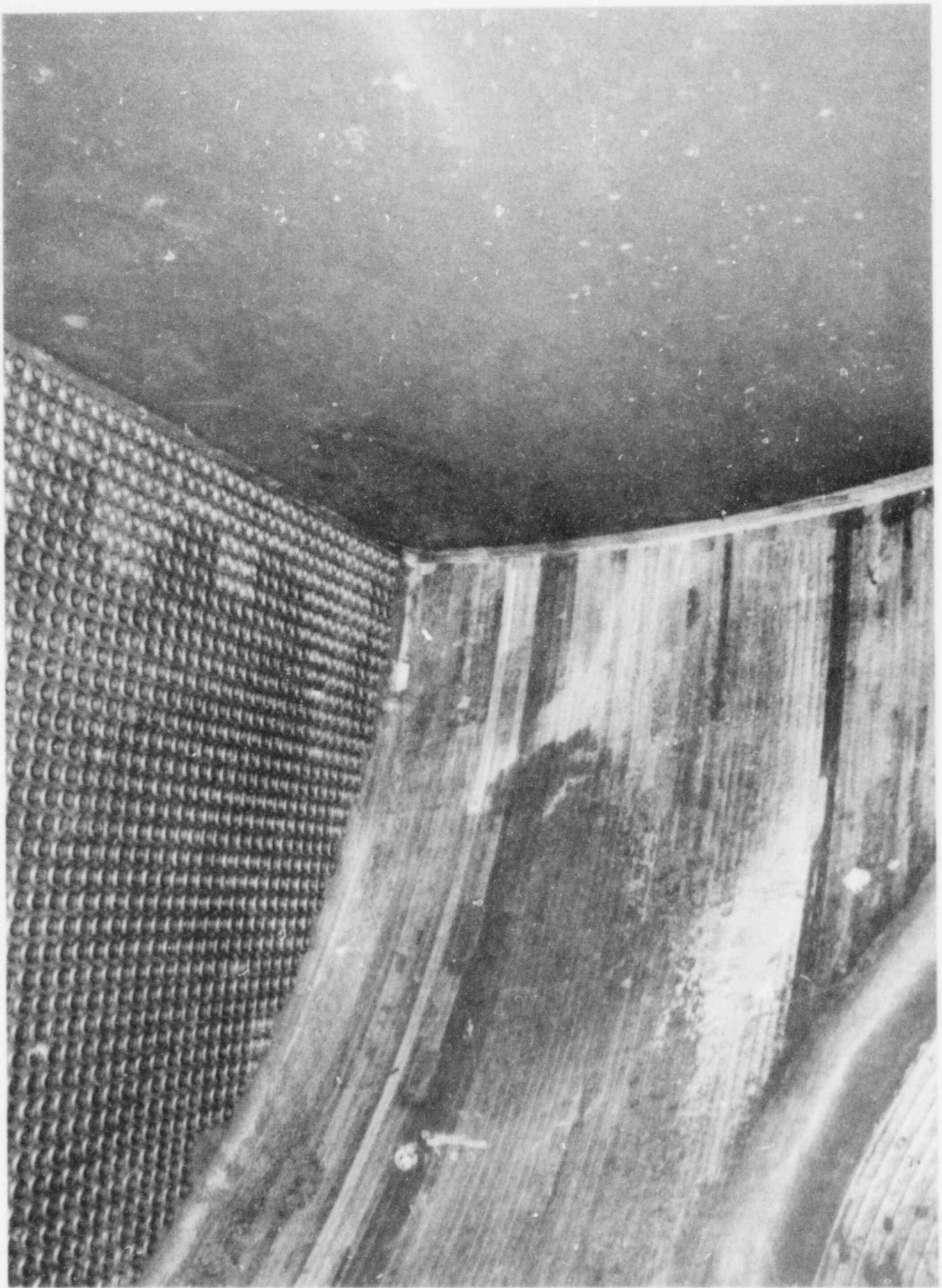
FIGURE 4-12. Hot Leg Surfaces After the AP/P0D Process
