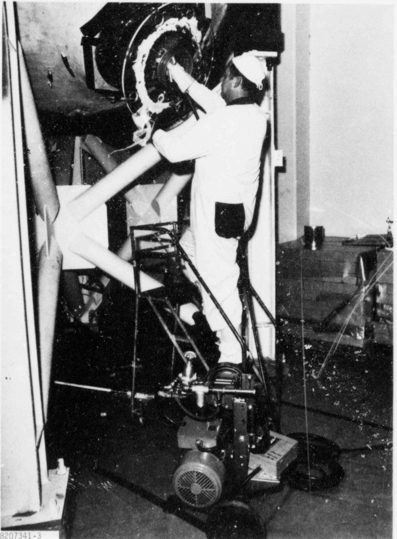
FIGURE 3-18. High-Pressure Water Rinse Operation
