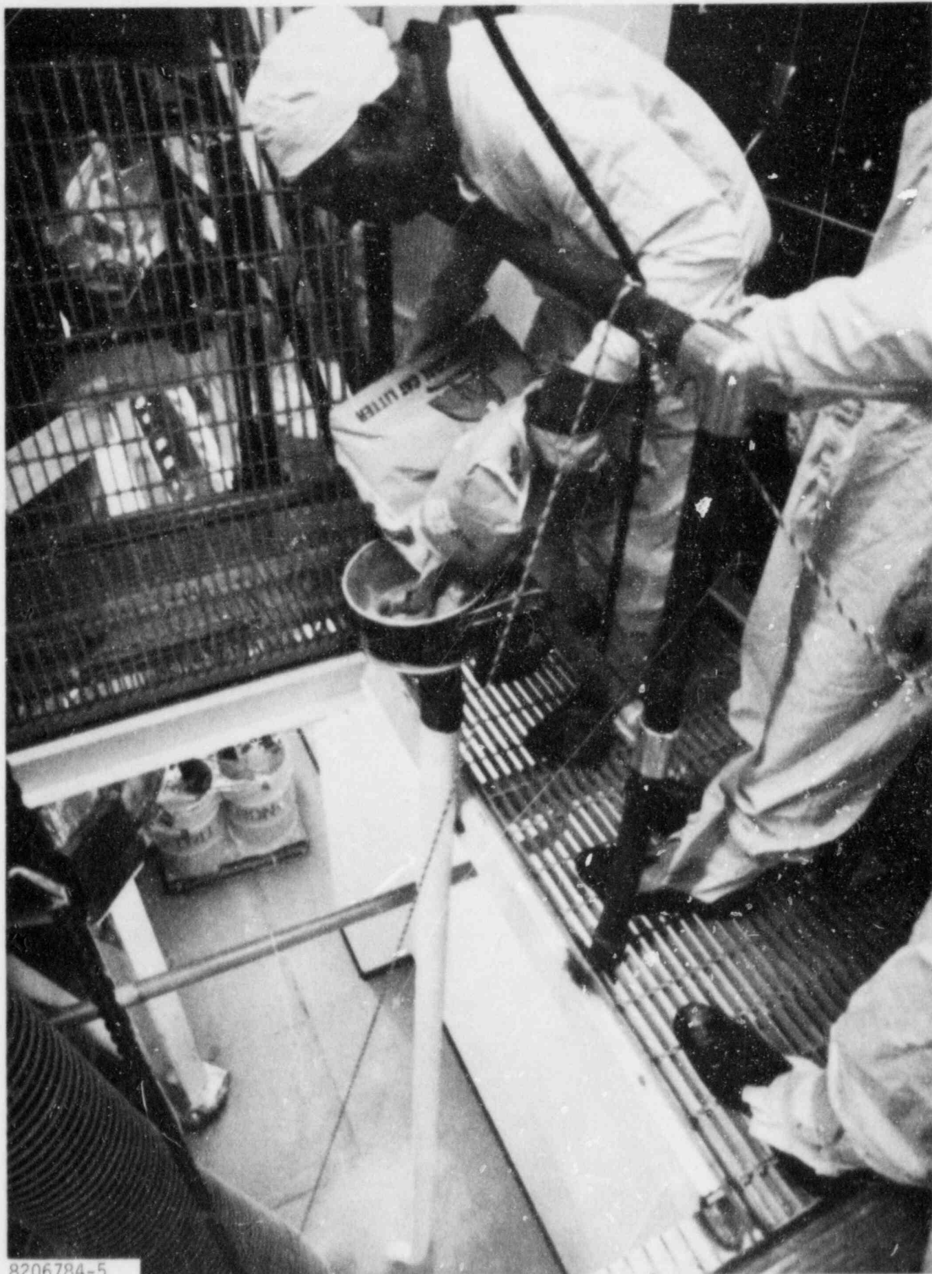
FIGURE 3-22. Remote Addition of Adsorbant Material
