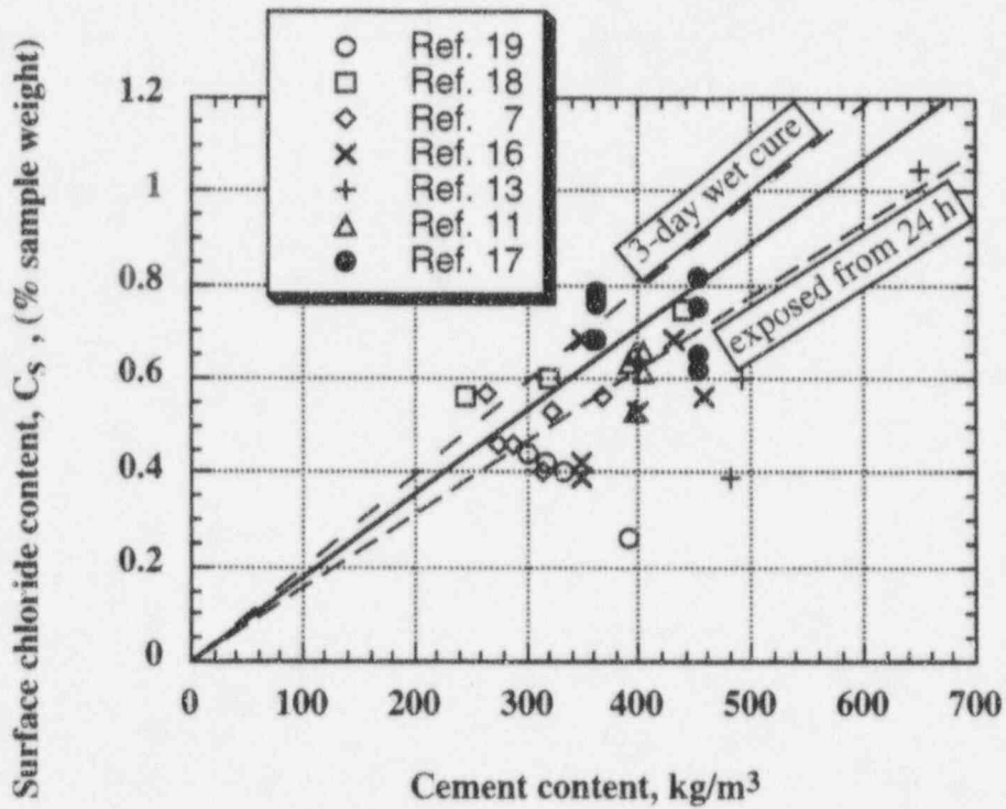
Fig. 2.15 Proposed curves for surface chloride content versus cement content for different curing conditions (Refs. refer to Ref. 123).
