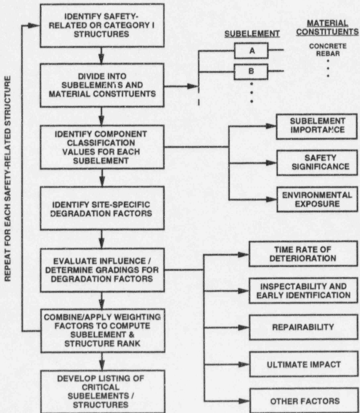
Fig. 4.1. Structural aging assessment methodology flow diagram.
