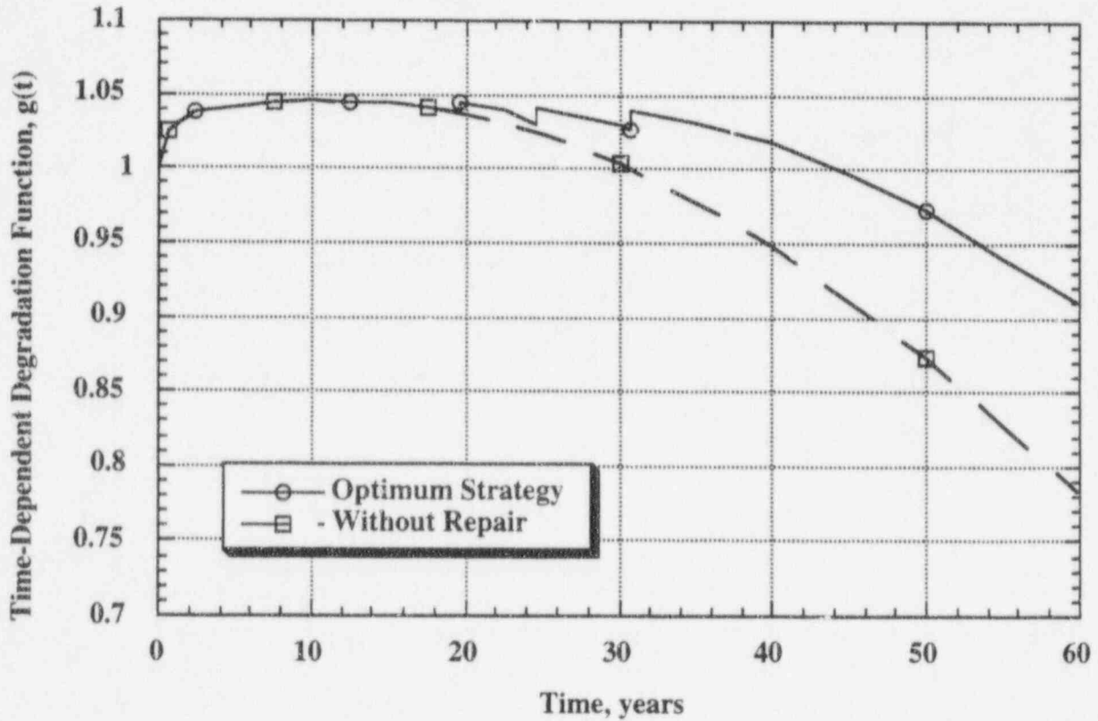
(b) Mean degradation function with optimum policy.
