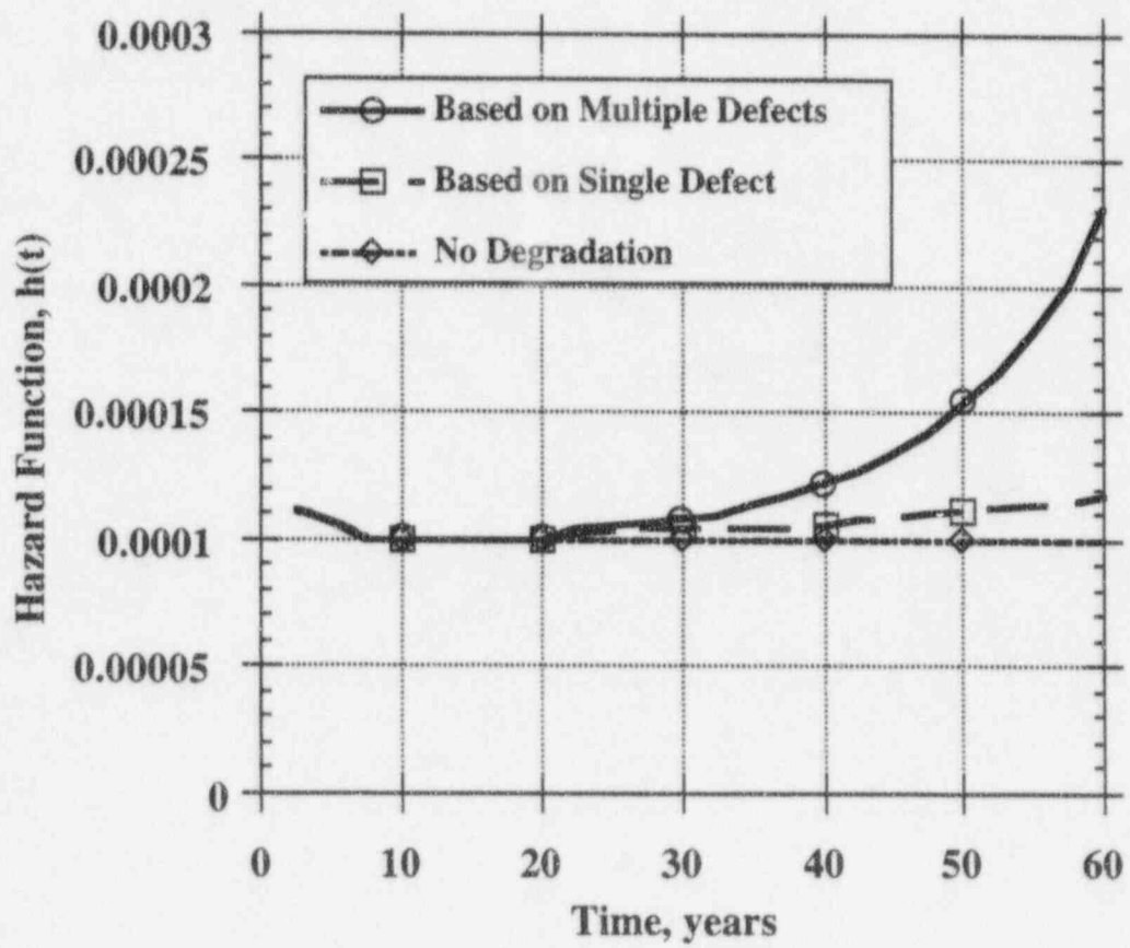
Fig. 5.7 Hazard function of wall in shear without repair.
