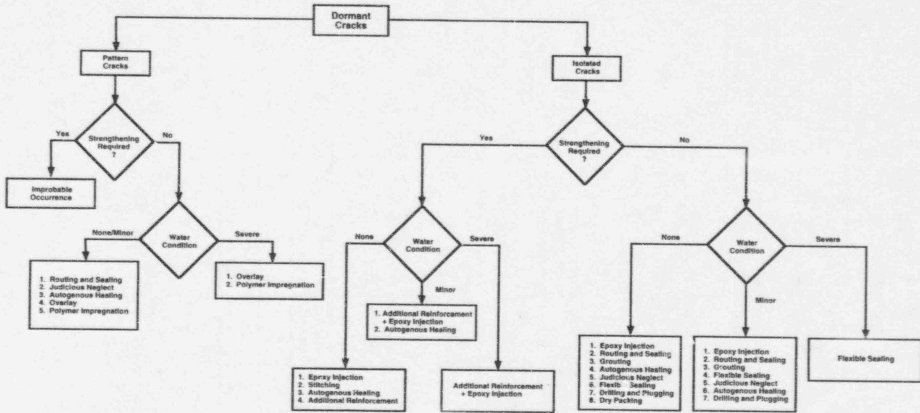
Fig. 3.5 Selection of repair technique for dormant cracks. Source: Evaluation and Repair of Concrete Structures , EM 1110-2-2003, U.S. Army Corps of Engineers, Washington, D.C., 1986.
