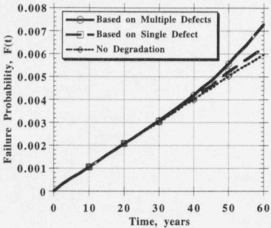
Fig. 5.6 Failure probability of wall in shear without repair.
