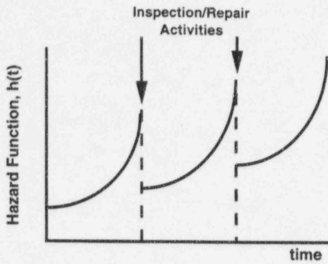
Fig. 5.9 Role of inspection/repair in controlling failure rate.
