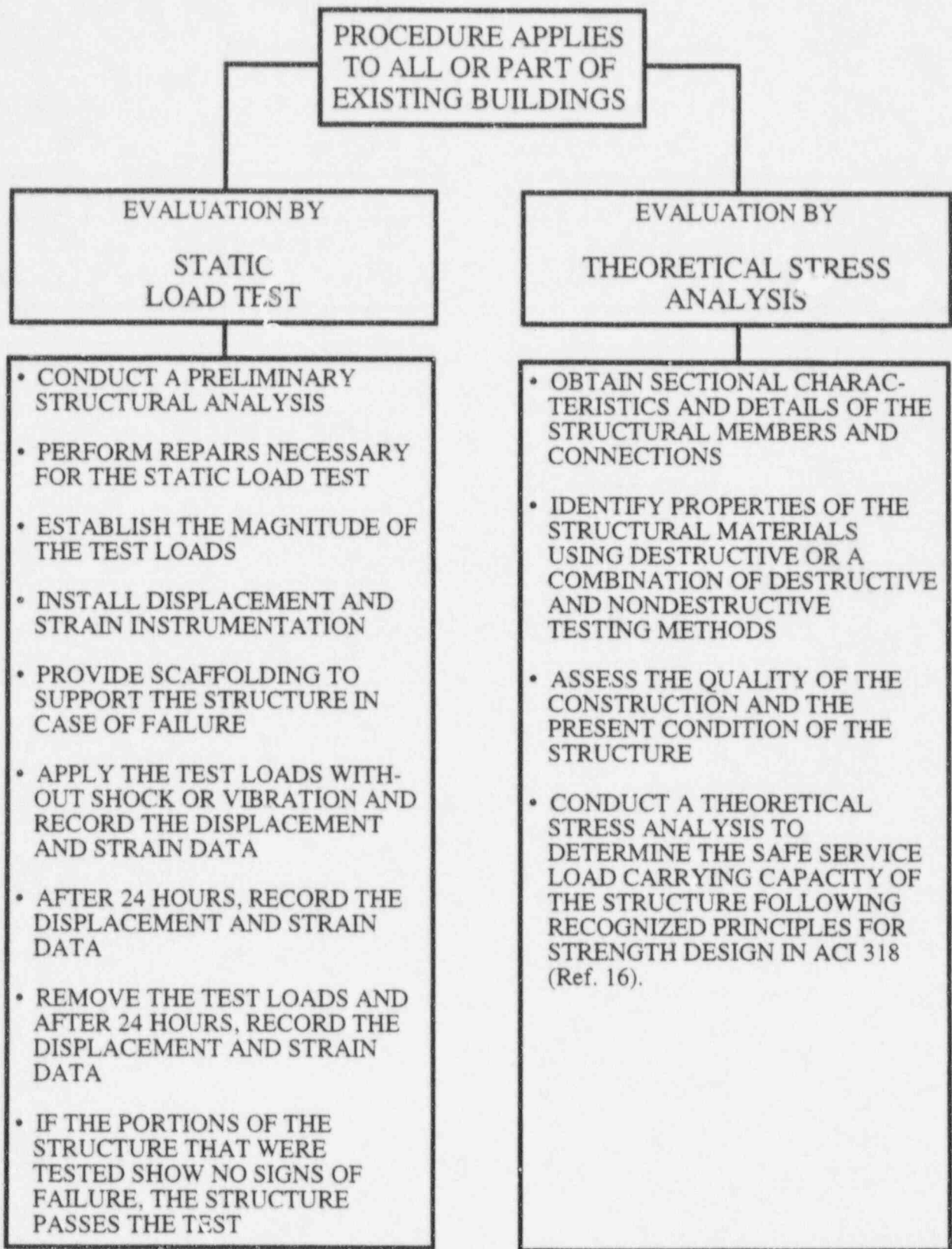
Fig. 2.23 Recommended procedure for strength evaluation of existing concrete buildings.
