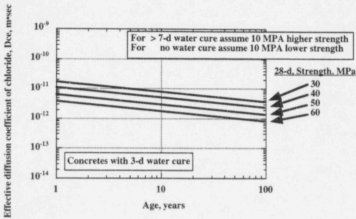
Fig. 2.16 Effective diffusion coefficient of chloride versus time for ordinary portland cement concretes. 123
