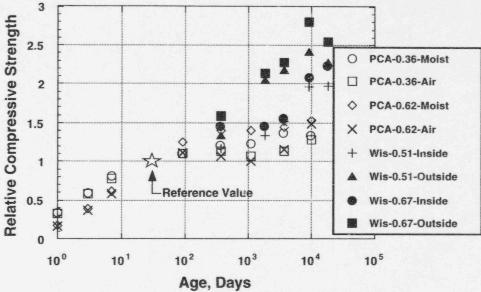
Fig 2.21 Long-term compressive strength results for selected data from University of Wisconsin and Portland Cement Association.
