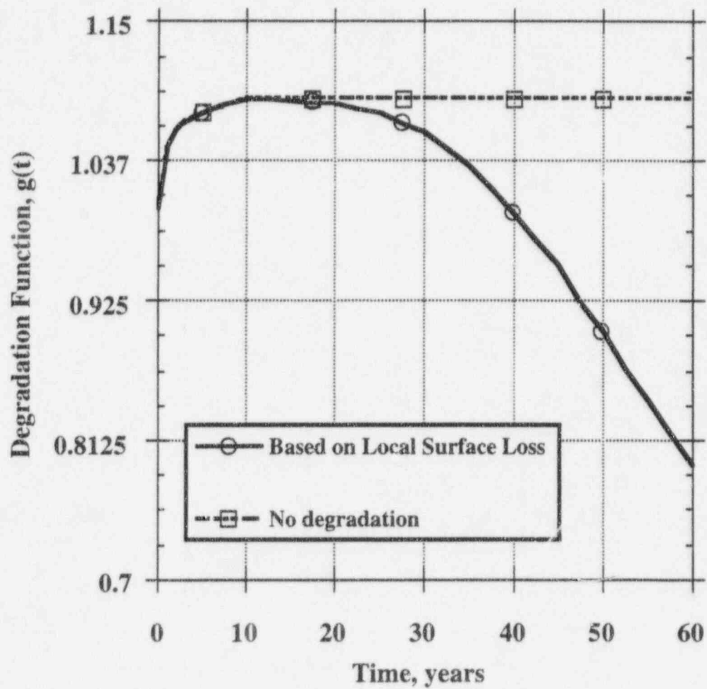
Fig. 5.8 Mean degradation function of wall in flexure/compression.
