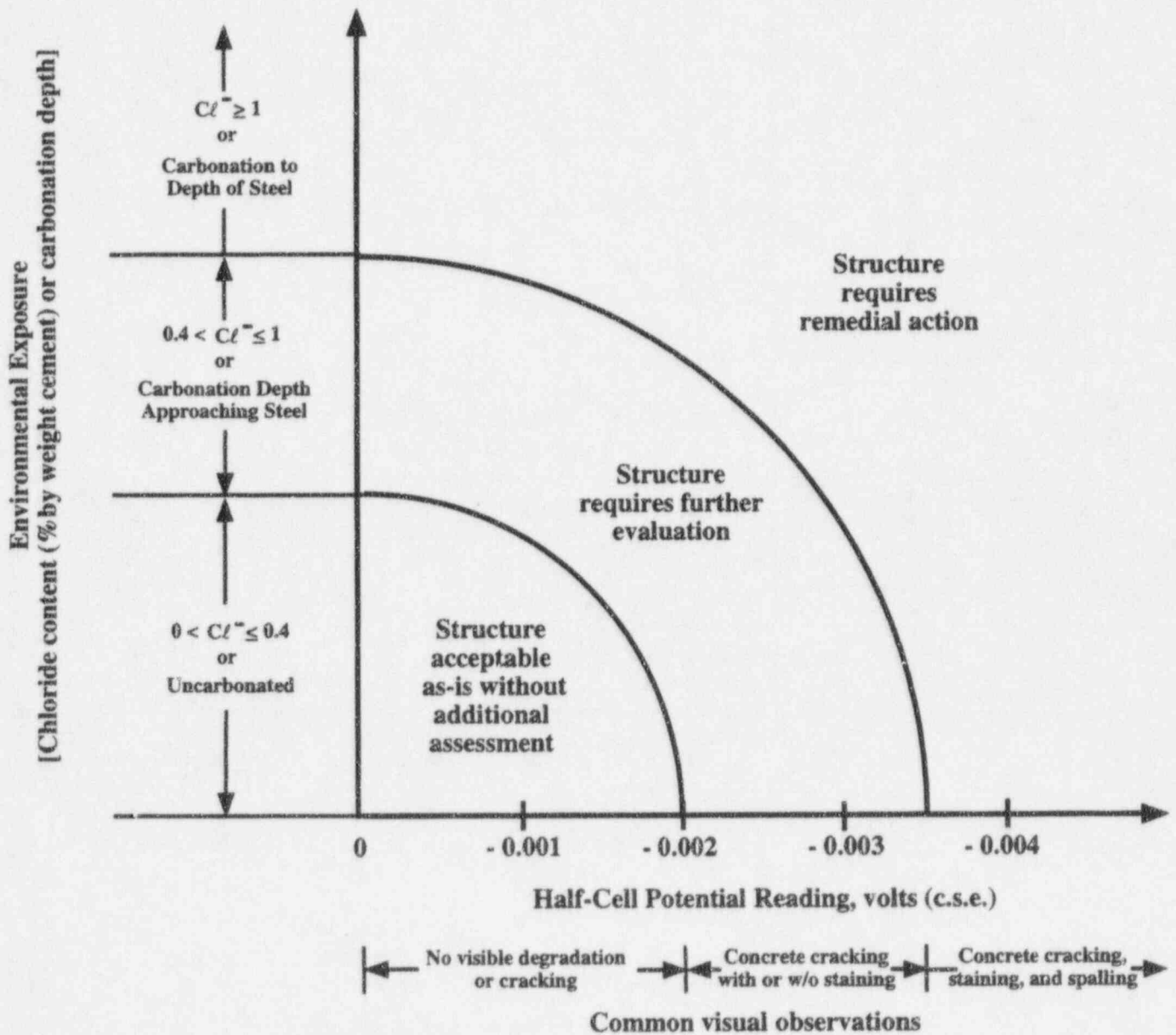
Fig. 4.3 Damage state chart relating environmental exposure, half-cell potential reading, and necessity for additional evaluation or repair
