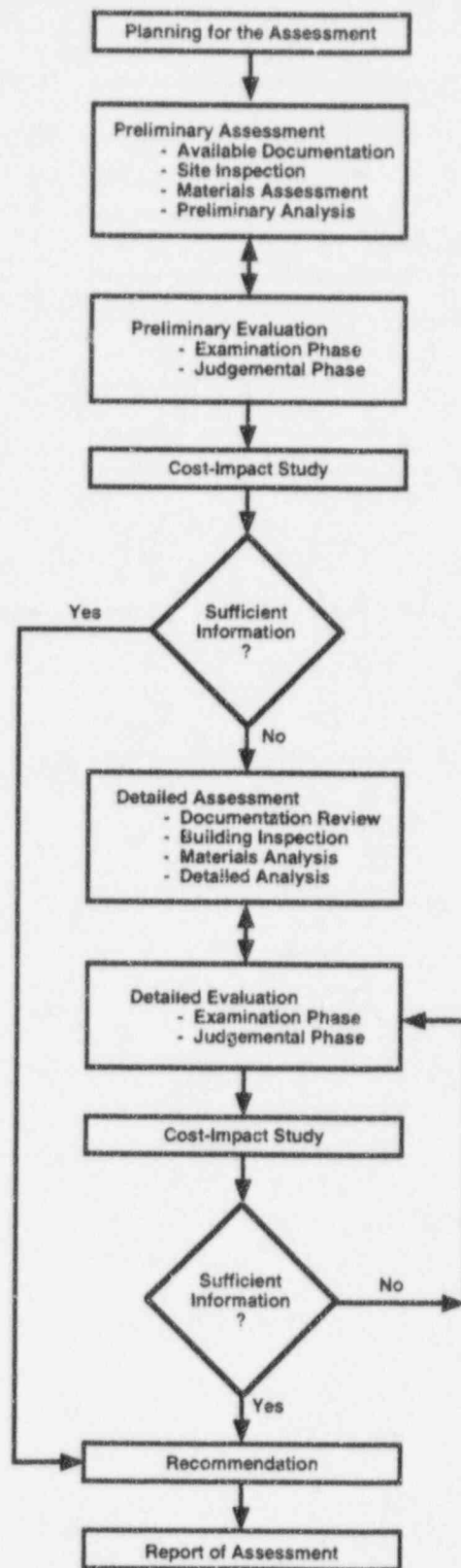
Fig. 3.2 General structural assessment and evaluation procedure for existing buildings. From ASCE 11-90, ASCE Guideline for Structural Condition Assessment of Existing Buildings , American Society of Civil Engineers, New York, New York, August 1, 1991; adapted with permission from ASCE, 1996.
