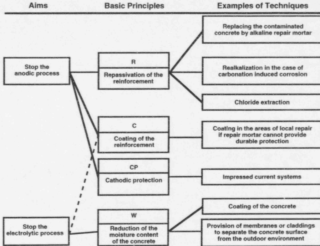
Fig. 3.7 Principles of repair to stop corrosion.
