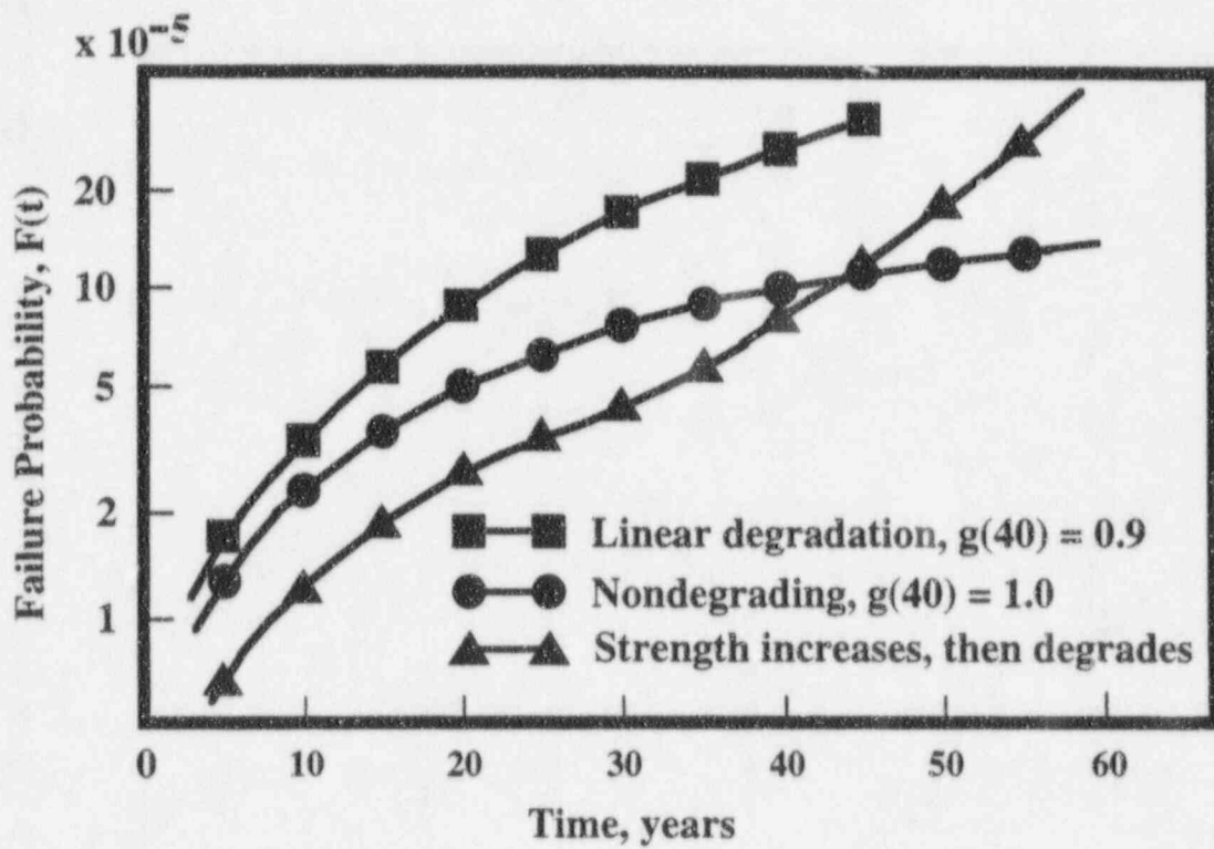
Fig. 5.3 Failure probability of a one-way slab.
