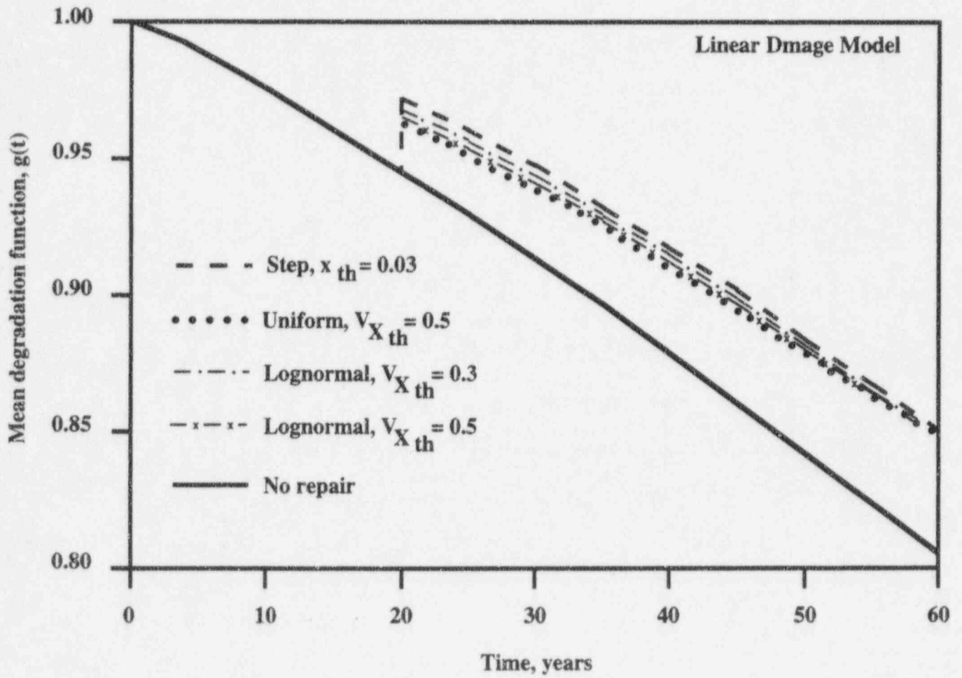
Fig. 5.11 Effect of several detectability functions on mean degradation function of inspection/repair.
