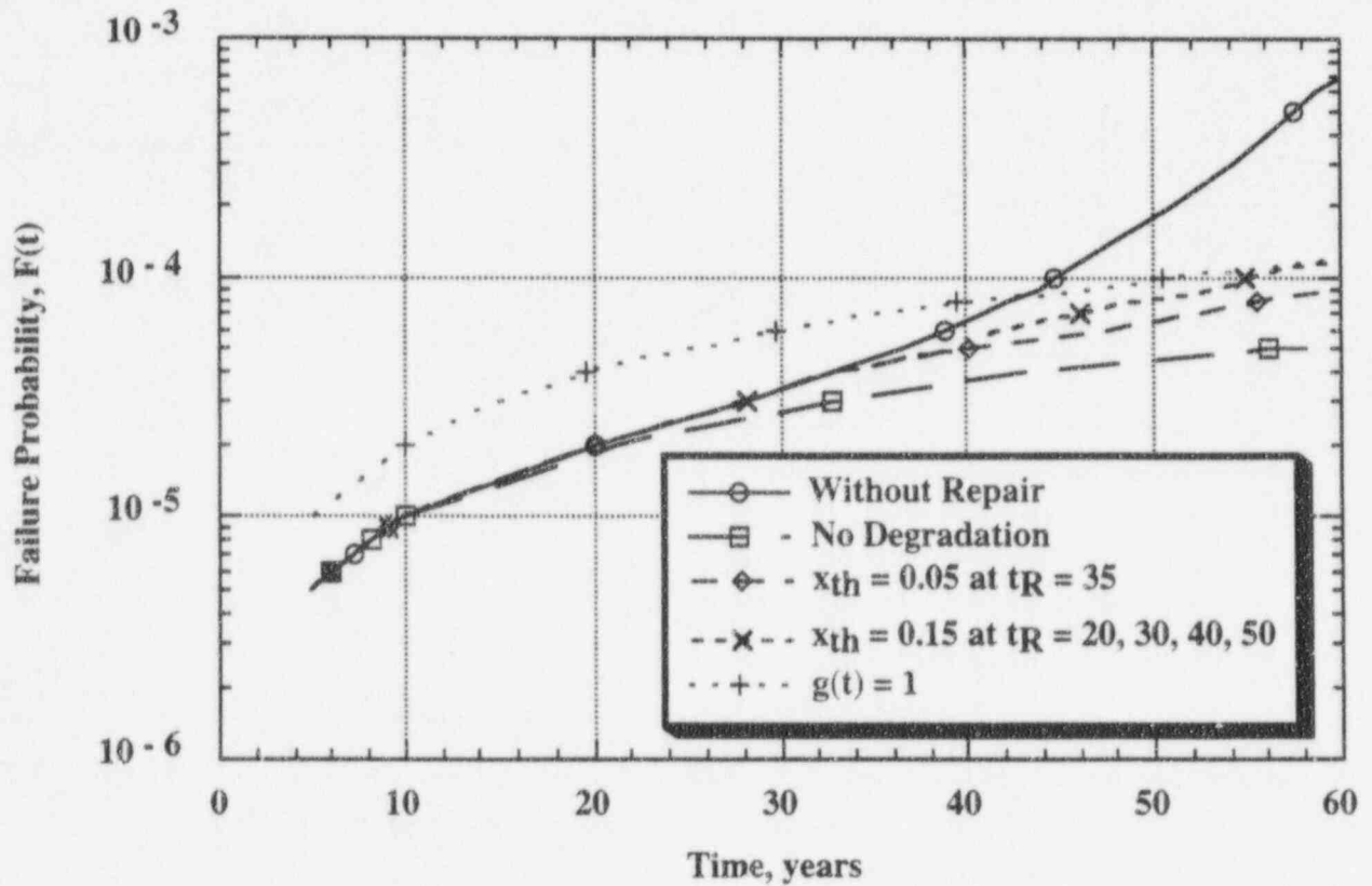
Fig. 5.19 Failure probability of slab with mean strength degradation in Fig. 5.18.
