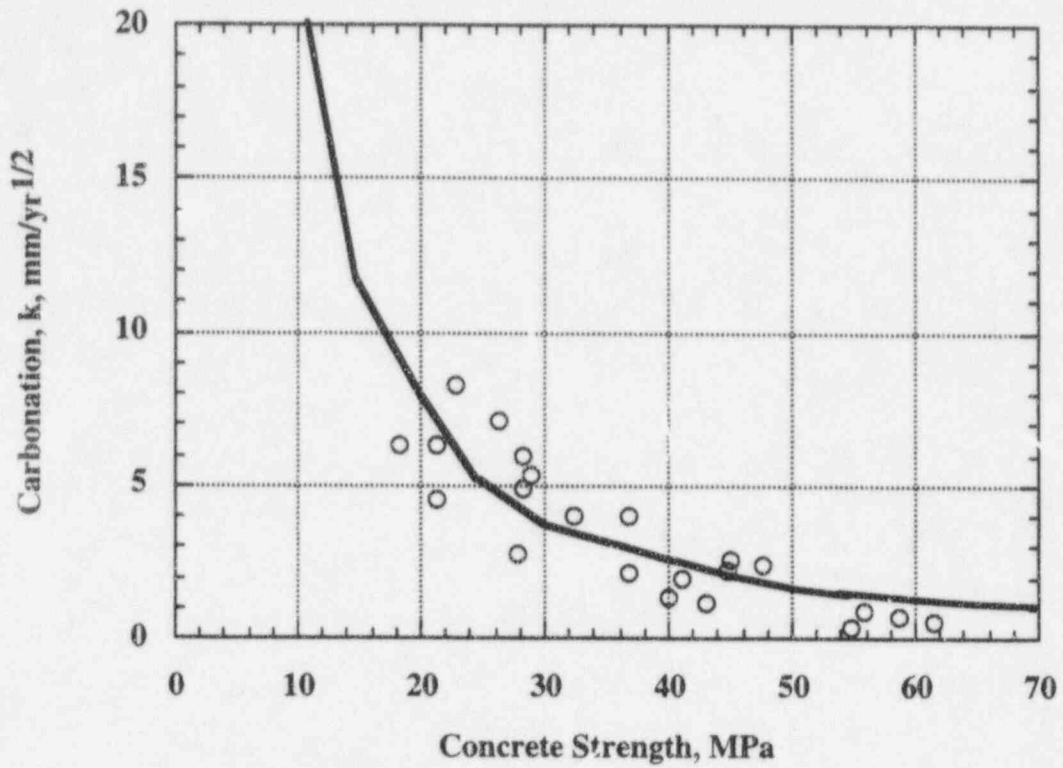
Fig. 2.14 Carbonation data for exterior sheltered concrete. 123
