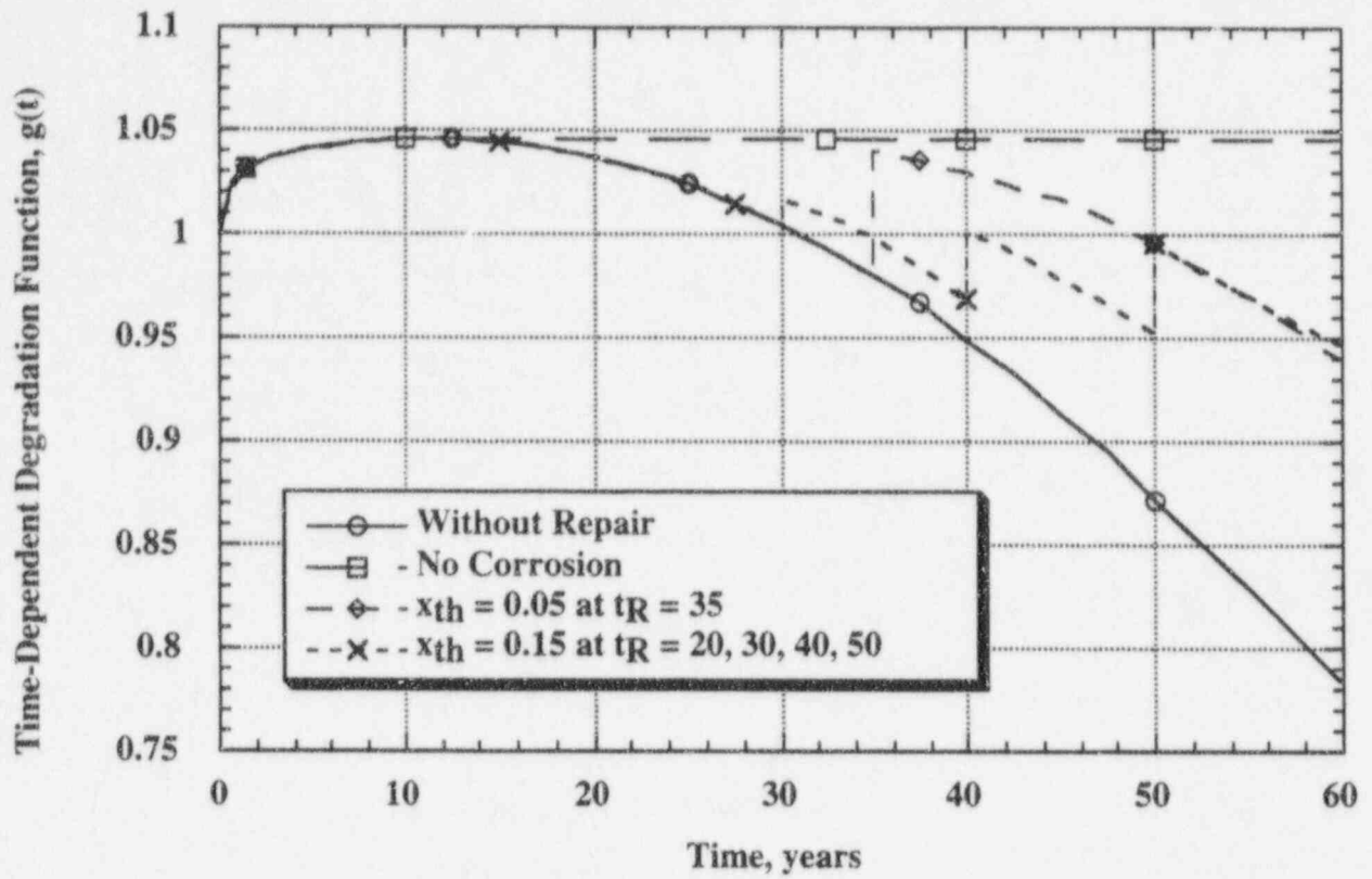
Fig. 5.18 Mean degradation function of slab subject to rebar corrosion.
