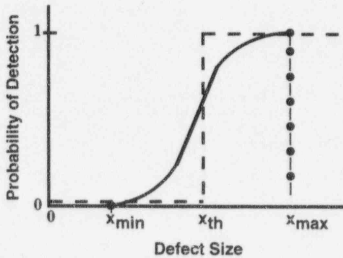
Fig. 5.10 Probability of detection of a defect of size x .
