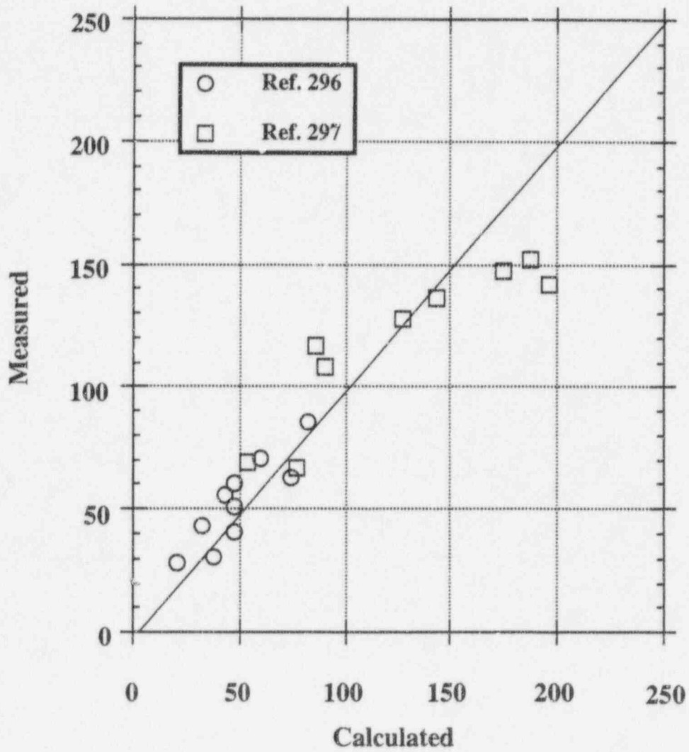
Fig. 5.4 Comparison of measured and calculated shear strength of low-rise reinforced concrete wall.
