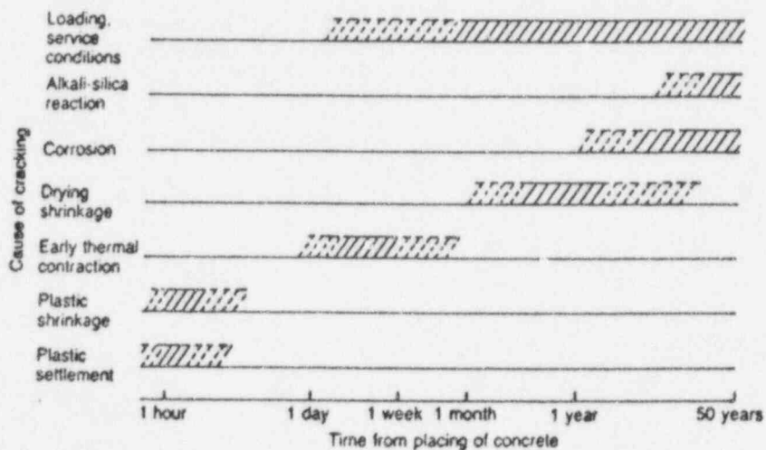
Fig. 2.11 Time of appearance of cracks from placing of concrete. Source: Comité Euro-International du Béton (CEB), Durable Concrete Structures-Design Guide , published by Thomas Telford Services Ltd., London, England, 1989; reprinted with permission from CEB and Thomas Telford Services Ltd.
