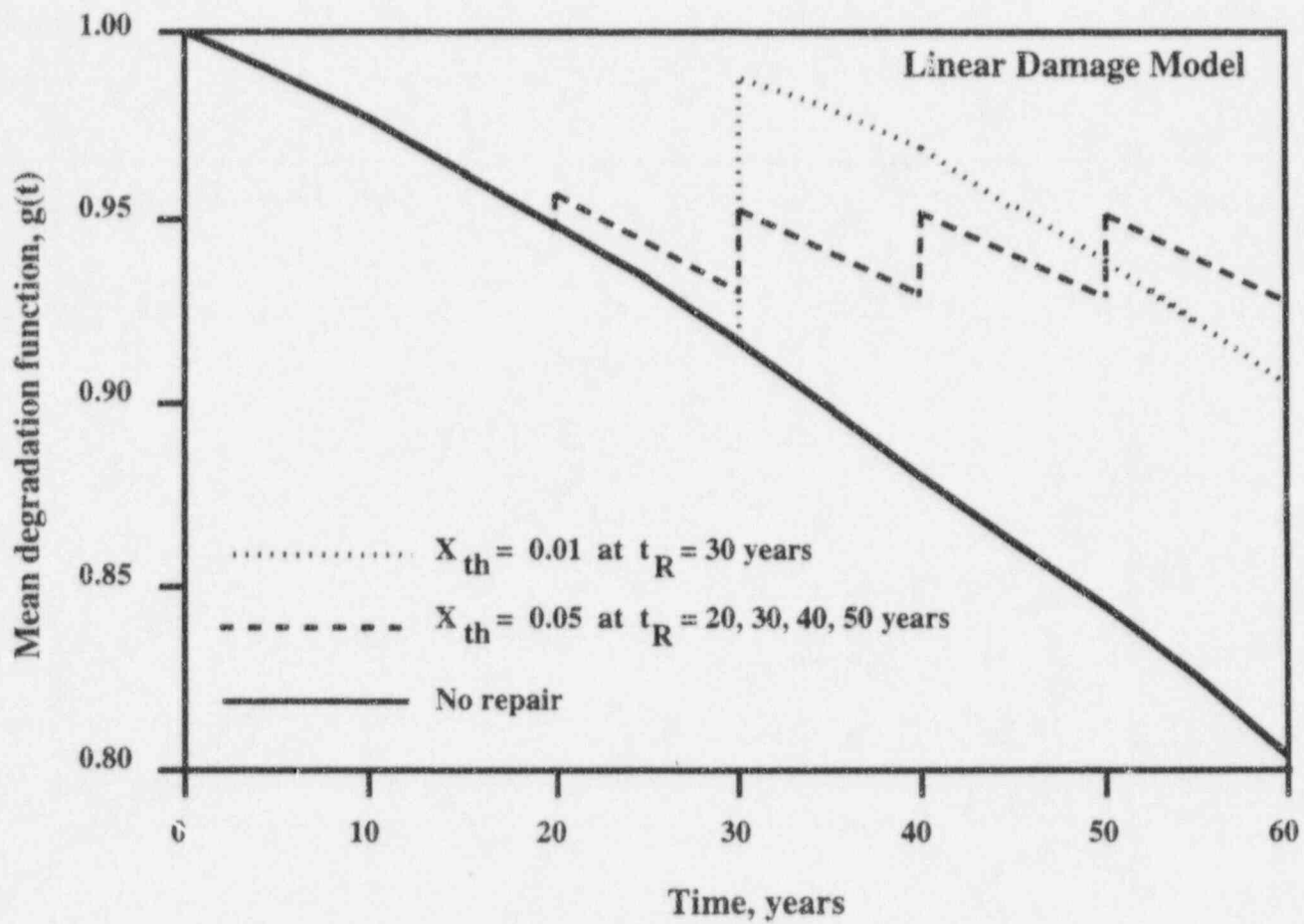
Fig. 5.12 Effect of multiple inspection/repairs on mean degradation function.
