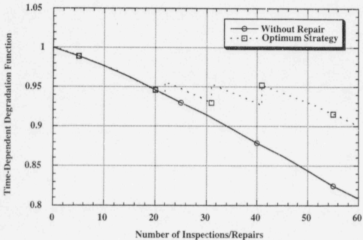
(b) Mean degradation function with optimum policy.
