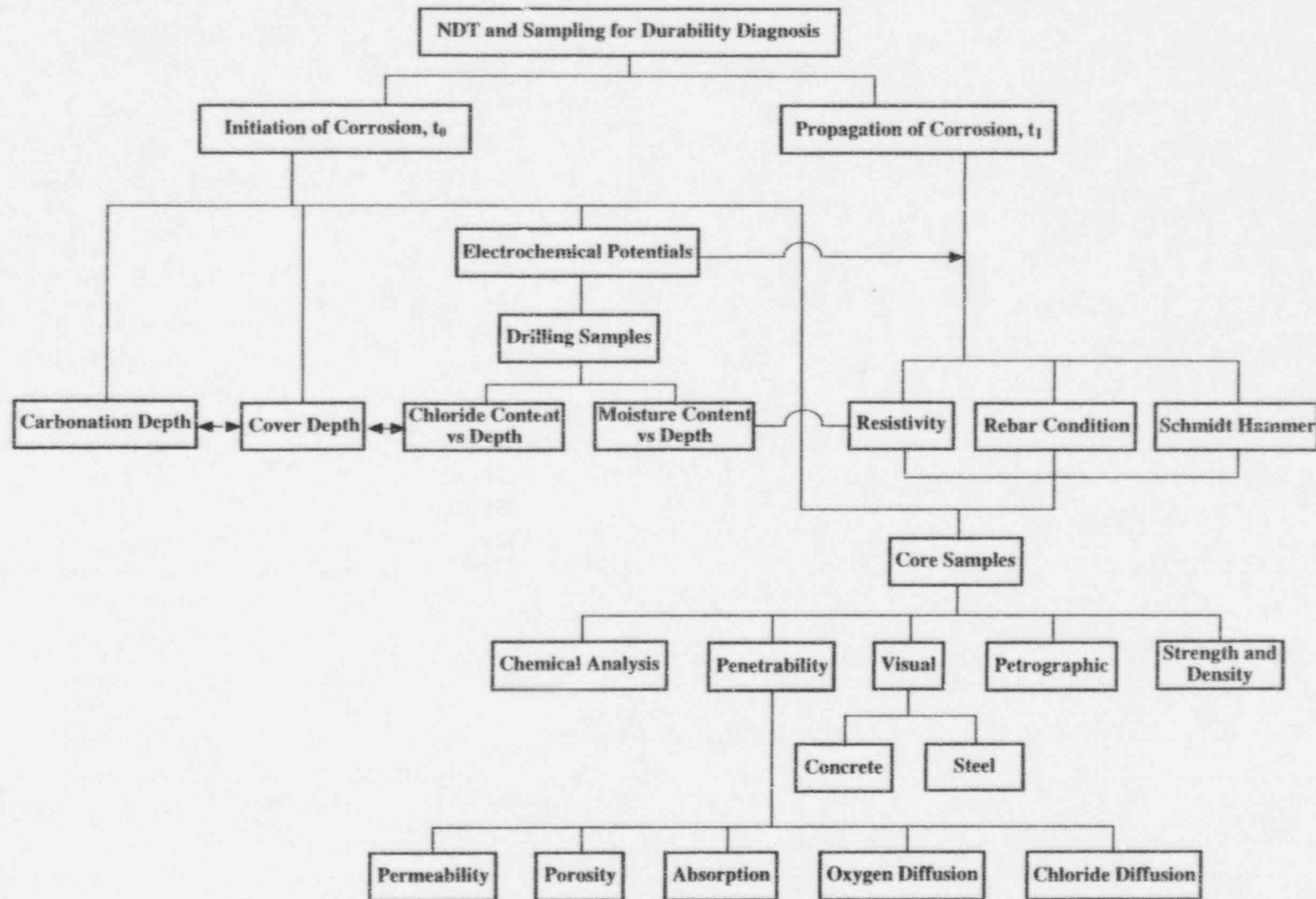
Fig. 3.1 Techniques for assessing deterioration. Source: R. D. Browne, "Durability of Reinforced Concrete Structures," Pacific Concrete Conference , Proceedings Vol. 3, Auckland, New Zealand, New Zealand Concrete Society, November 1988; reprinted with permission from author.
