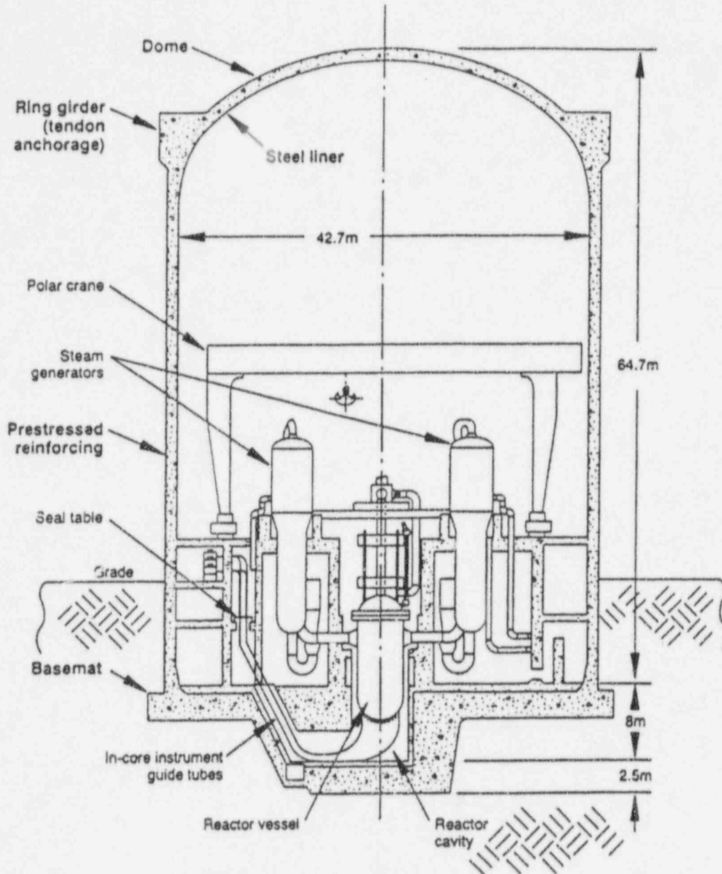
Fig. 2.6 PWR large dry prestressed concrete containment.
