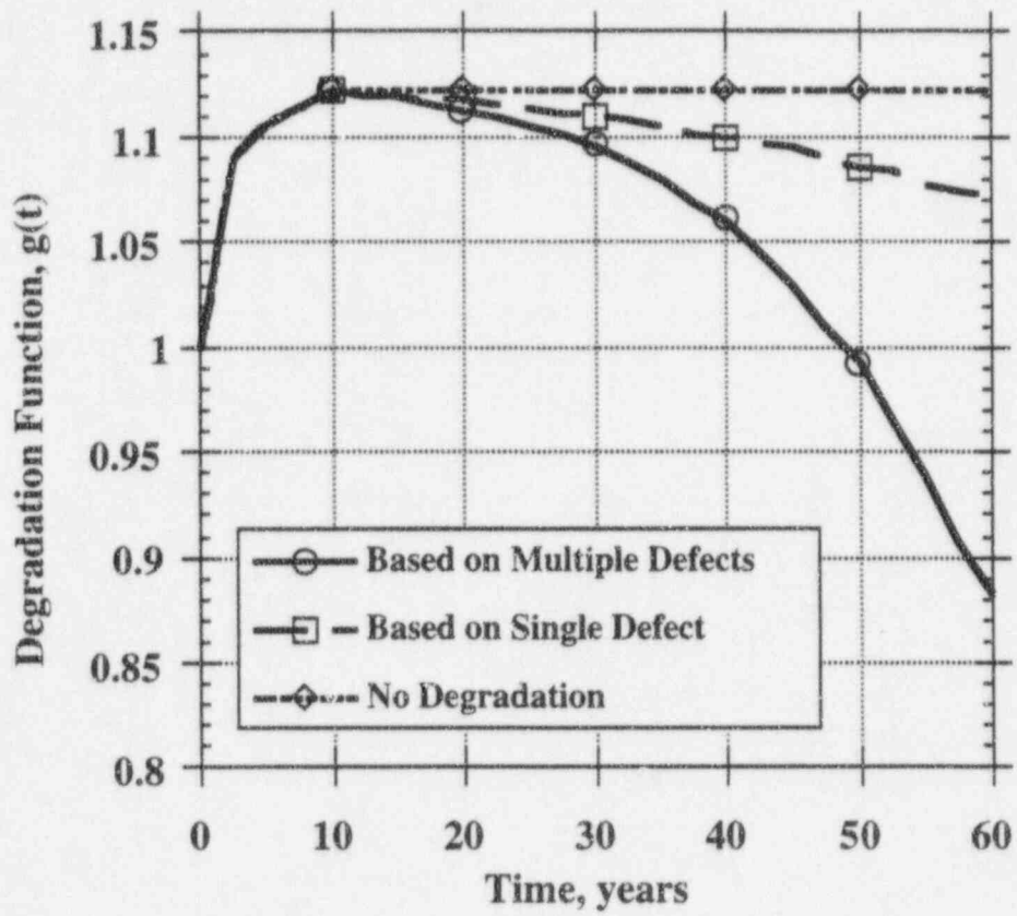
Fig. 5.5 Mean degradation function of wall in shear without repair.
