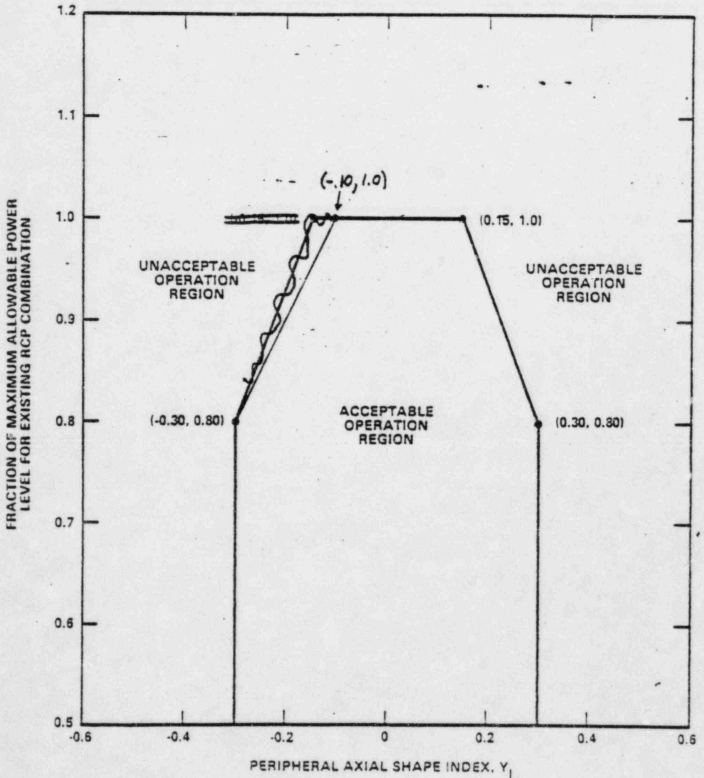
Figure 3.2-4 DNB Axial Flux Offset Control Limits
